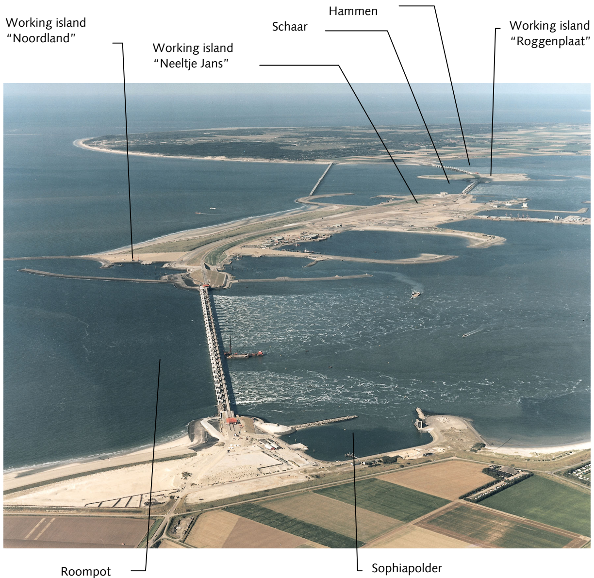
Figure 2.5: An aerial photograph of the Eastern Scheldt storm surge barrier with the channel "Roompot" in the front and in the back the channels "Schaar" and "Hammen" (photograph courtesy of RWS-Meetskundige Dienst).
