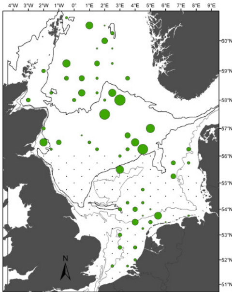
Fig. 1: Location of matching stations with distances apart superimposed (m).
