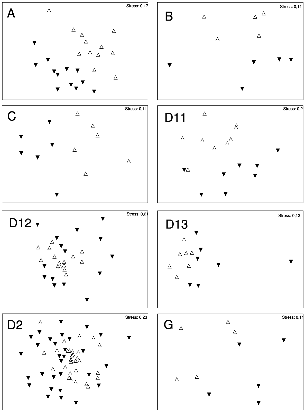
Fig. 6: MDS-plots revealed with fourth-root transformed abundance data of 1986 ( \Delta ) and 2000 ( \blacktriangledown ) for the stations of each cluster (see Fig. 3).
