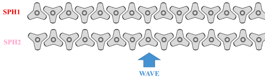
Fig. 11. Two different configurations can be simulated according to the initial orientation of the Tetrapods.
