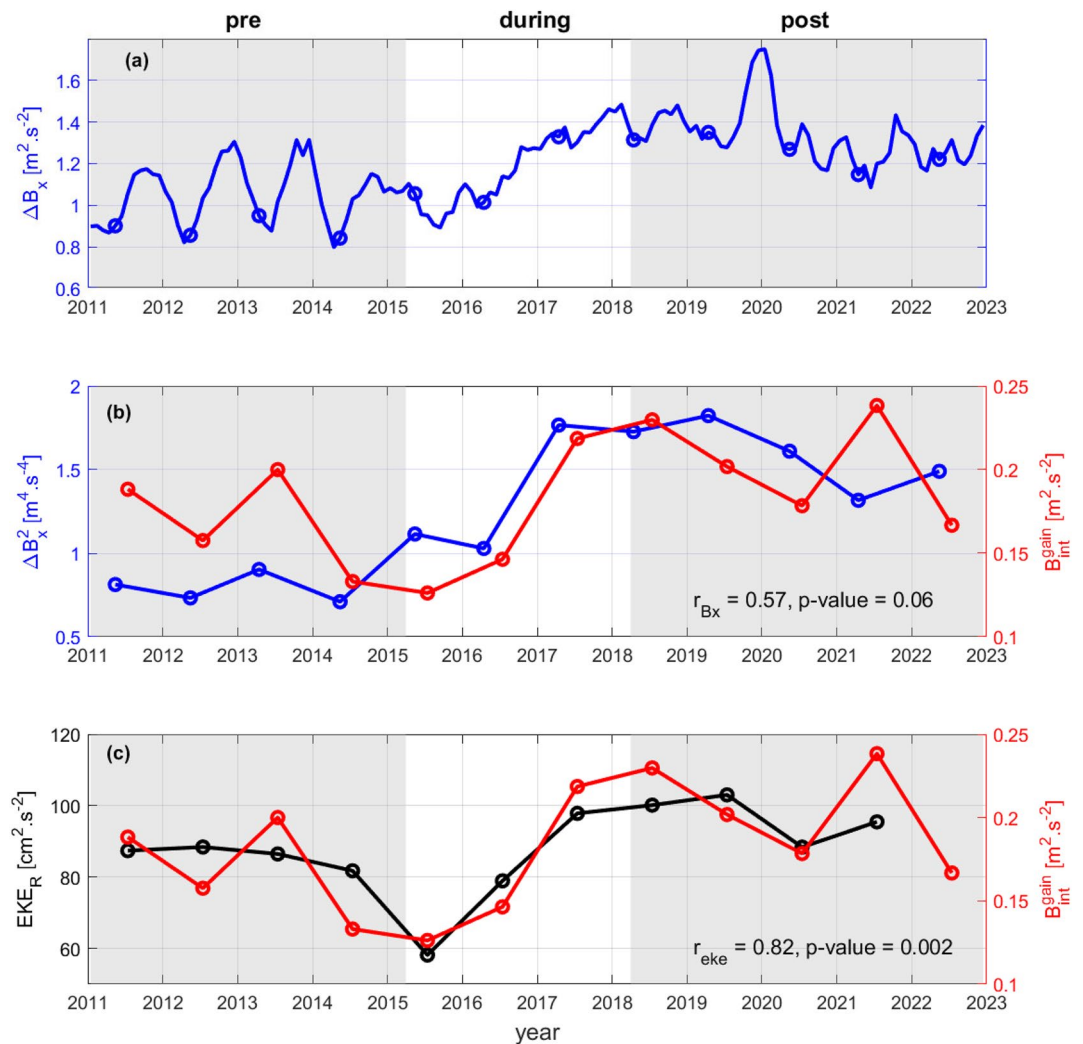
Figure 3. (a) Monthly time-series of the horizontal difference in buoyancy content (integrated over the 100–1,000 m layer) across the Irminger Current (IC), from x_1 to x_2 (see Figure 1a), circles show the \Delta B_x value at the start of the restratification period. (b) Comparison of the interannual variability in the square of the horizontal difference in buoyancy content over the IC at the start of the restratification period, \Delta B_x^2 (blue) and the buoyancy content gain in the interior over the restratification period in the 100–1,000 m layer, B_{\text{gain}}^{\text{int}} (red). (c) Comparison of the interannual variability in the average eddy kinetic energy (EKE) in the IC region during the restratification period, EKE_R (black) and B_{\text{gain}}^{\text{int}} (red).
