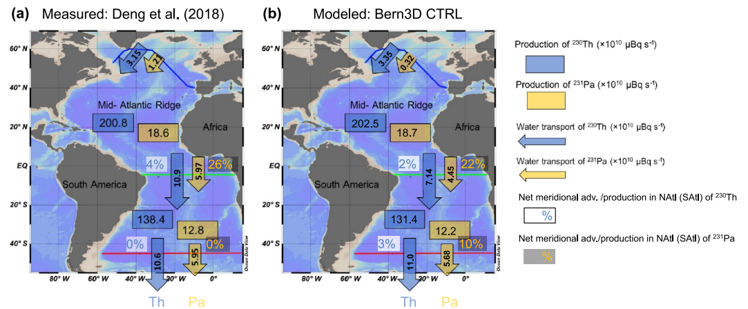
Figure 8. Budget of Atlantic ^{231}\text{Pa} (yellow) and ^{230}\text{Th} (blue) in \mu\text{Bq s}^{-1} as computed (a) from observational estimates by Deng et al. (2018) and (b) from the Bern3D model CTRL run. Boundaries of the North and South Atlantic follow the transects GEOVIDE, WOCE A07 (4.5°S), and WOCE A11 (simplified version shown) (Deng et al. (2014); see Figure C4 for the transects on the Bern3D grid). Percentages express how much of the produced ^{231}\text{Pa} and ^{230}\text{Th} is exported out of the North or South Atlantic sub-basin by advection. The rest either sinks to the sediment within the sub-basin or is transported out of it by horizontal diffusion of ^{231}\text{Pa} and ^{230}\text{Th} . Adapted from Deng et al. (2018).
