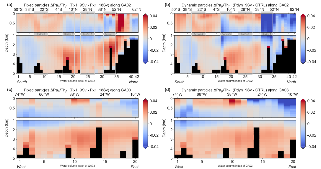
Figure 11. Response of modeled ^{231}Pa/^{230}Th_p to a ~50% Atlantic Meridional Overturning Circulation (AMOC) weakening along the two major Atlantic transects: GA02 in the upper panels (a), (b) and GA03 in the lower panels (c), (d). Red indicates increasing ^{231}Pa/^{230}Th_p when AMOC decreases, and blue indicates decreasing ^{231}Pa/^{230}Th_p when AMOC decreases. The result is shown for fixed particles (PI particles \times 1 ) in the left panels (a), (c) by subtracting run's Px1_18Sv ^{231}Pa/^{230}Th_p from that in Px1_9Sv, and for dynamic particles in the right panels (b), (d), where CTRL = Pdyn_18Sv. See Figures 3c and 3d for trajectory maps of GA02 and GA03.
