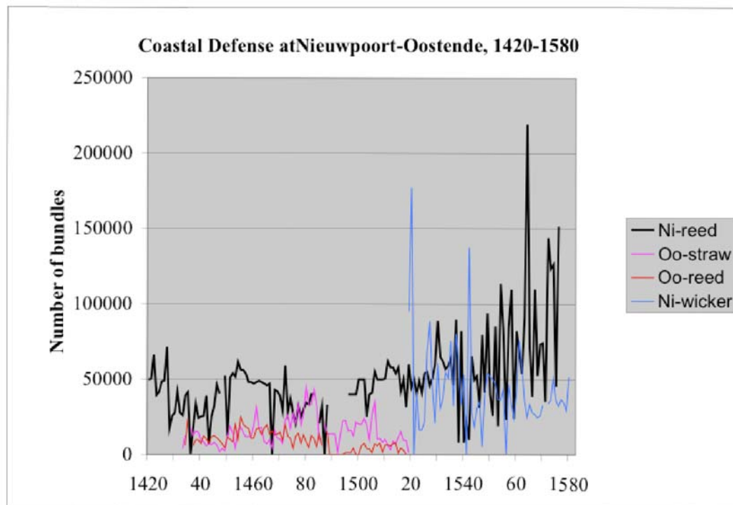
Fig. 5. Use of reed and straw for coastal protection and annual maintenance at Nieuwpoort and Oostende, 1420-1580.
