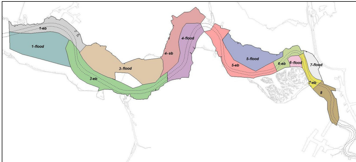
Figure 4. Division of the Scheldt Estuary in macro-cells.
