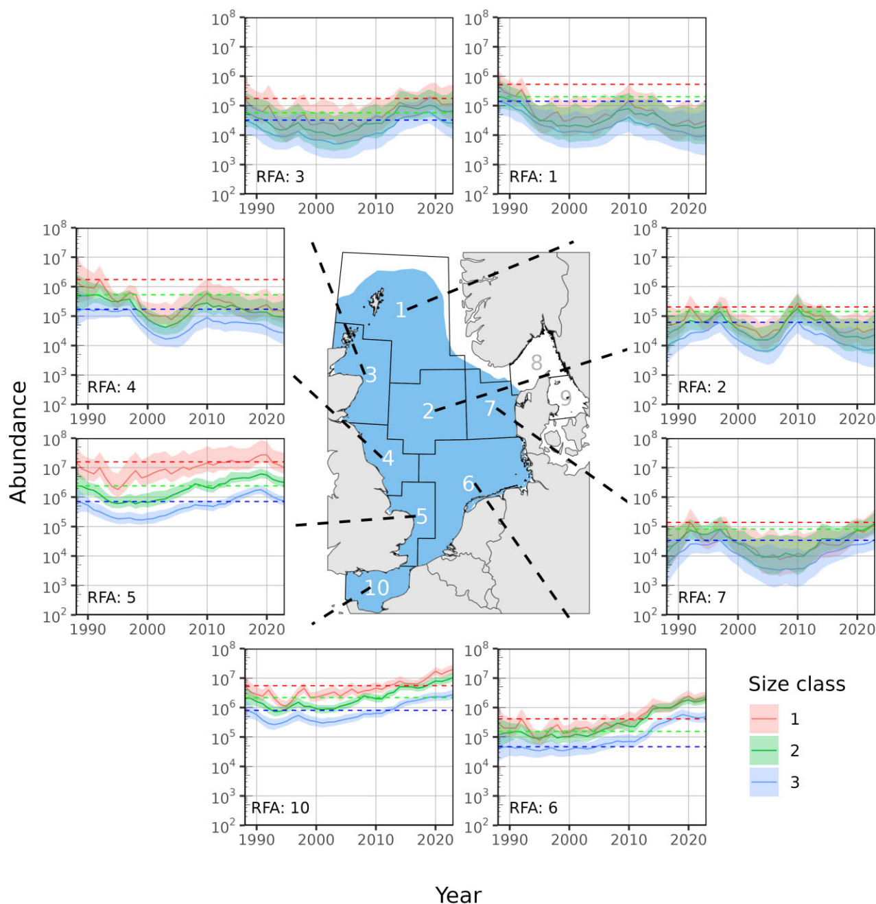
Figure 4. Predicted abundance (in number of individuals) of size classes of R. clavata from 1988 to 2023 for RFA 1–7 and 10, with 95% credible intervals and pre-2000 abundance peak baselines (dashed line) for size class 1, size class 2, and size class 3. The blue polygon indicates the area used for abundance predictions. Note that y-axes are log-scaled.
