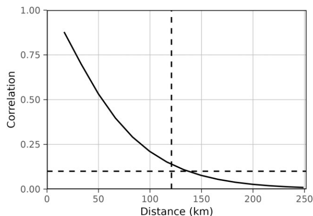
Figure 2. The Matérn correlation function (solid line) describes the correlation between locations in the SPDE model in relation to their distance to each other. The vertical dashed line indicates the estimated range, at which the correlation is ~0.1 (horizontal dashed line).
