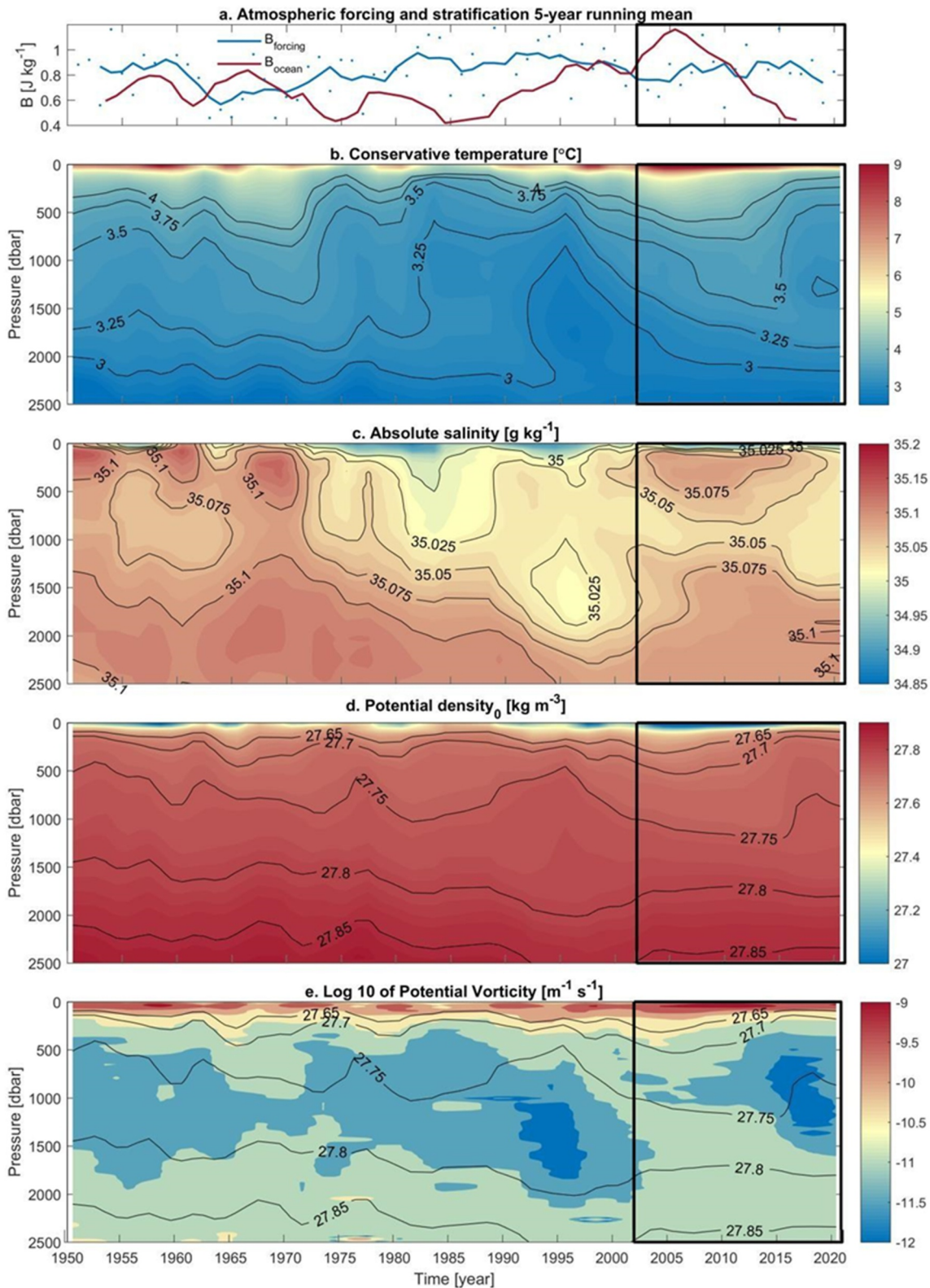
Figure 2. Central Irminger Sea multi-decadal hydrographic time series of (a) 5-year running mean values of the stratification over the upper 1,000 m (red) and the cumulative atmospheric forcing (blue). Annual forcing values shown as blue dots. (b) conservative temperature, (c) absolute salinity, (d) potential density, and (e) potential vorticity. The mooring period is indicated with the black box.
