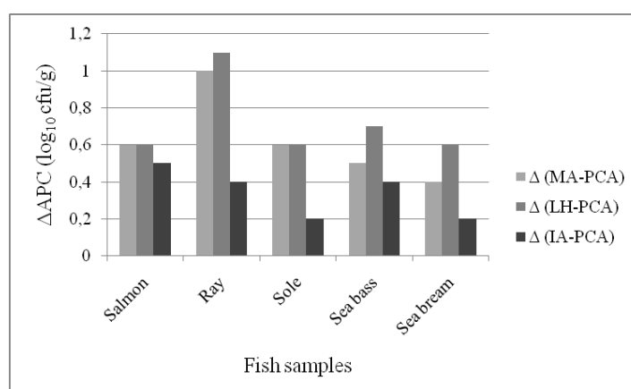
Fig. 3.1. Differences ( \Delta ) in total aerobic psychotolerant count (APC) ( \log_{10} cfu/g) between MA, LH, IA and PCA growth media at arrival ( T_1 ) of fish samples. Only those fish samples are shown where a higher difference than 0.5 \log_{10} cfu/g between PCA and the salt-containing media (MA, LH and IA) was observed.
