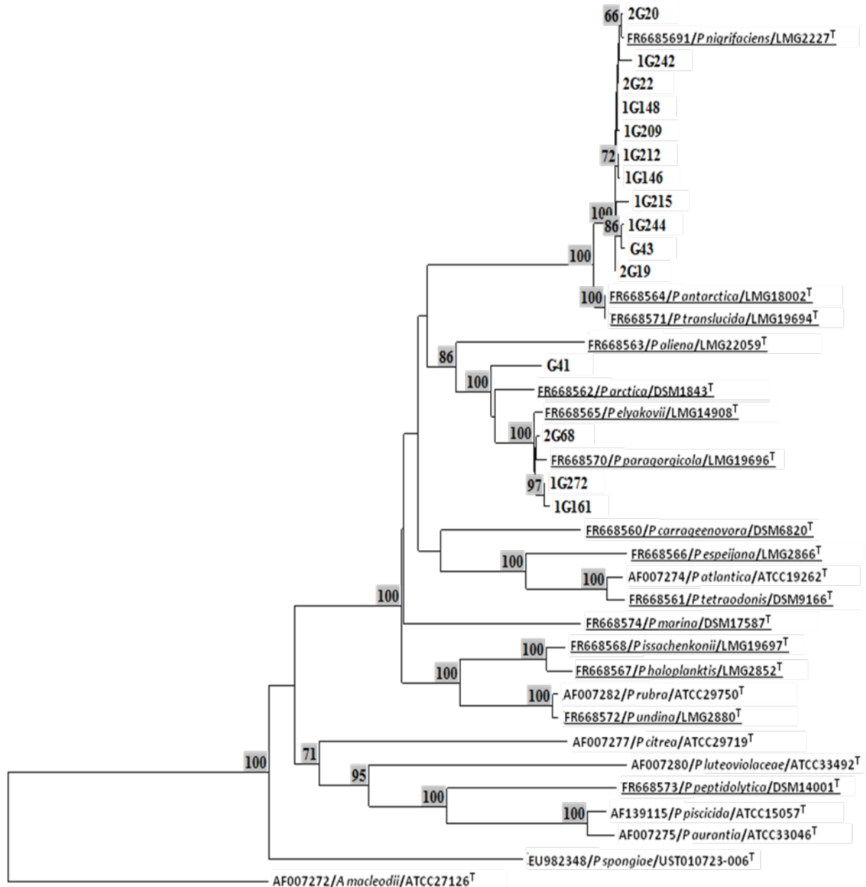
Fig 4.4. Phylogenetic tree of the genus Pseudoalteromonas , with the isolates from brown shrimp included, based on the gyrB gene sequence (1500bp). The type strains which were sequenced and submitted to the EMBL nucleotide sequence database are underlined. The tree was constructed with the neighbour-joining method. Genetic distances were calculated by the Jukes & Cantor model. The scale shows the genetic distance of 0.02. The percentages on the nodes give the bootstrap values (on 1000 bootstrapped trees). Only values above 65% are shown. Alteromonas macleodii was used as outgroup.
