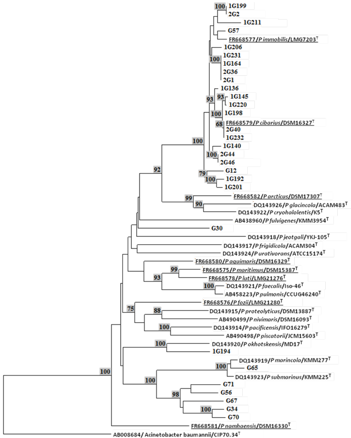
Fig 4.3. Phylogenetic tree of the genus Psychrobacter , with the isolates from brown shrimp included, based on the gyrB gene sequence (1500bp). The type strains which were sequenced and submitted to the EMBL nucleotide sequence database are underlined. The tree was constructed with the neighbour-joining method. Genetic distances were calculated by the Jukes & Cantor model. The scale shows the genetic distance of 0.02. The percentages on the nodes give the bootstrap values (on 1000 bootstrapped trees). Only values above 65% are shown. Acinetobacter baumannii was used as outgroup.
