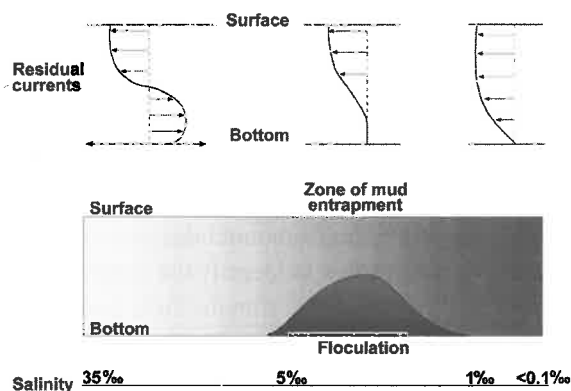
Fig. 1. Influence of density currents on the residual transport of suspended matter and on sediment accumulation in a partially well mixed estuary.
