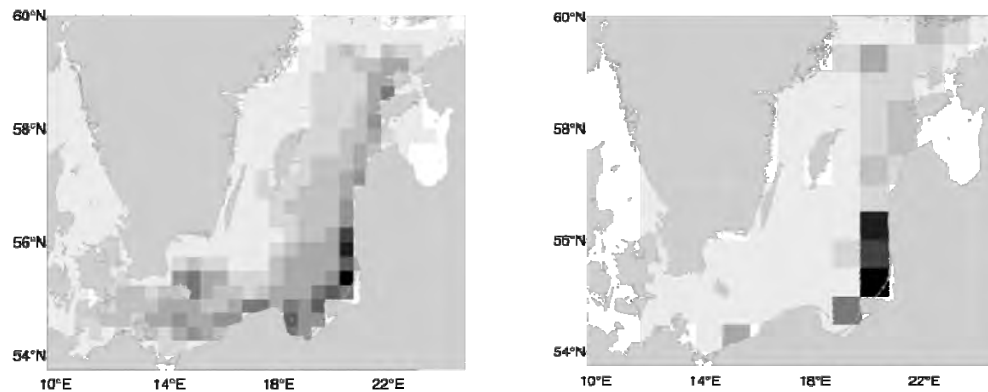
Figure 7.4. Mean observed distribution of sprat juveniles, based on hydroacoustics (left) and coupled hydrodynamic modelling 1979–2002 (right).
