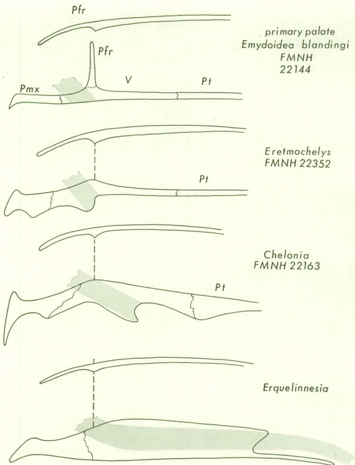
FIG. 6. — Diagrammatic sagittal sections through the skulls of turtles with primary and differing degrees of secondary palates. The course of the nasal passages — on either side of the sagittal plane — is indicated by shaded areas.
