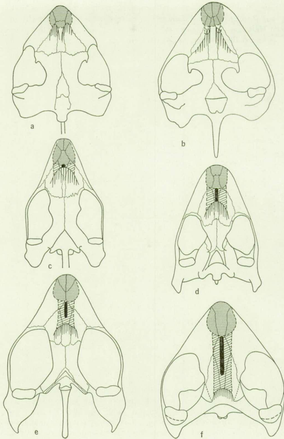
FIG. 8. — Comparison of the nasal cavity, nasal passages and position of the choanal opening(s) in turtles with primary and secondary palates.
