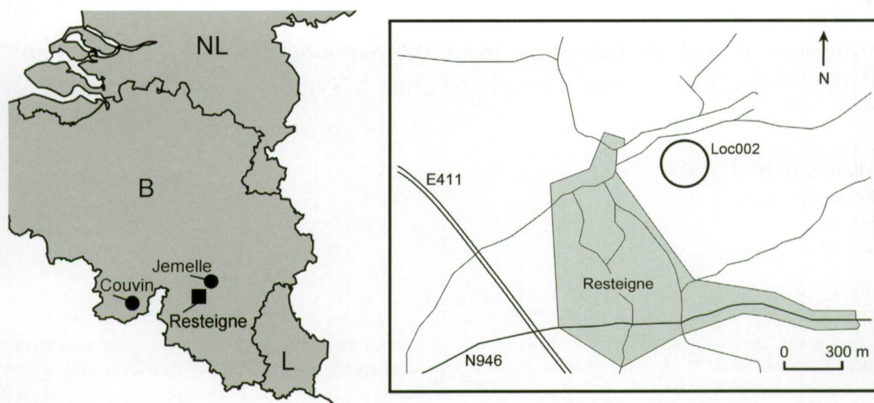
Fig. 1 — Location of abandoned quarry of Resteigne (Loc002) in southern Belgium. Square on overview map indicates position of local map within Belgium.
