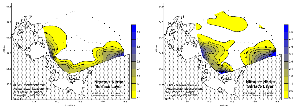
Figure 3 Distribution patterns of nitrate in the surface layer before (left) and during (right) and outflow event in September 1993. Sampling positions are marked on the map with a plus (+)
