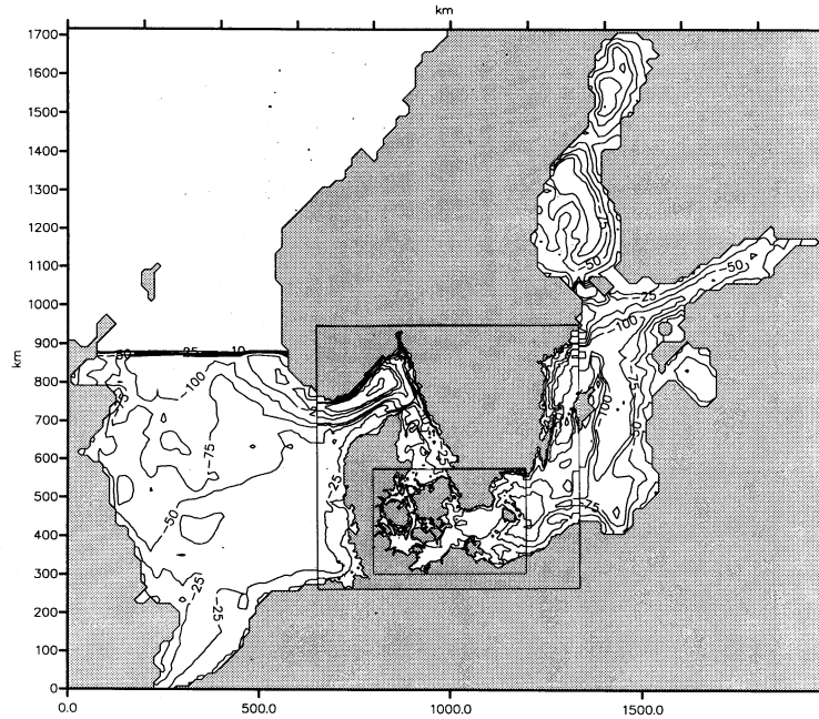
Figure 1 The DYNOCS model set-up with 3 levels of two-way interactive nesting; 9 nm, 3 nm and 1 nm grid resolution
