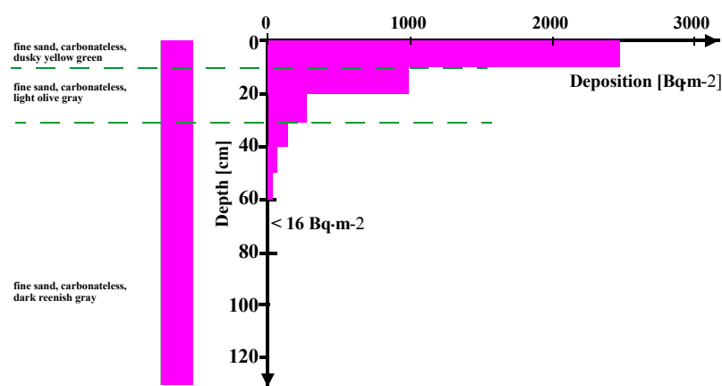
Figure 4 Vertical deposition of Cs-137 at station 23 (54°27.27'; 19°36.31')
