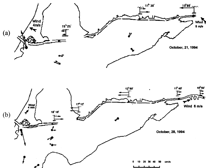
Figure 4 Currents in Kaliningrad Marine Channel and the Gulf of Kaliningrad with winds from the south-east and south-west
