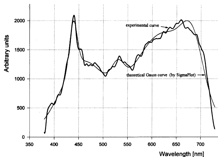
Figure 3 Experimental and calculated fluorescent spectrum
