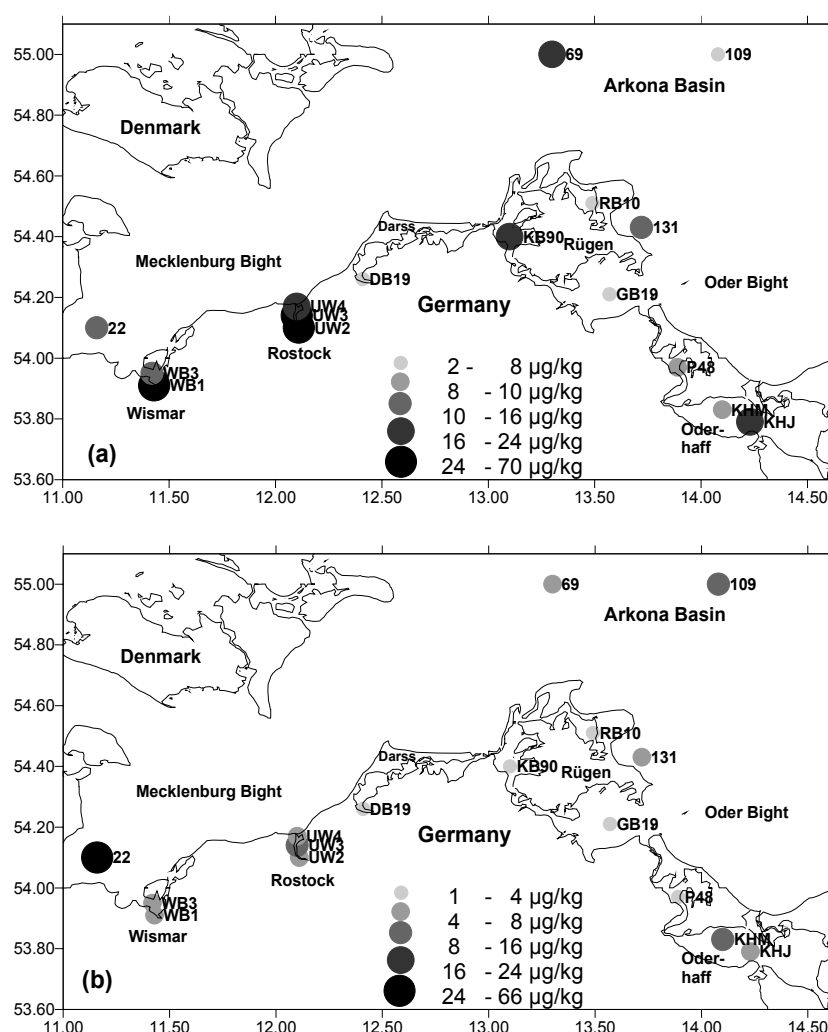
Figure 3 Distribution of PCDDs (a) and PCDFs (b) in the investigated sea area
