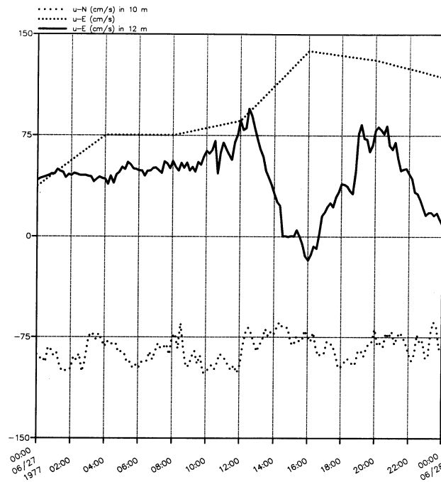
Figure 9 Current speed towards N at station 532 at 10m depth in Langelands Belt, and towards E at station 528 at 12m depth and at Fehmarn Belt lightship.
