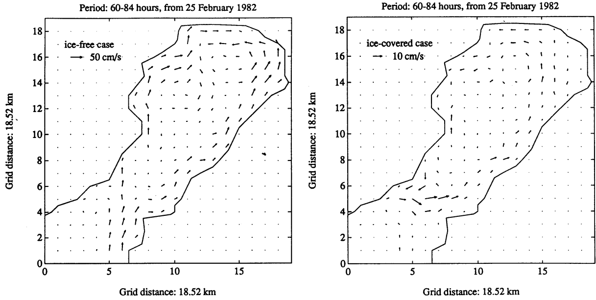
Figure 5 The depth-averaged current velocity in the Bay of Bothnia in case 1. The velocities are means over the strongest winds period (24 hours)
