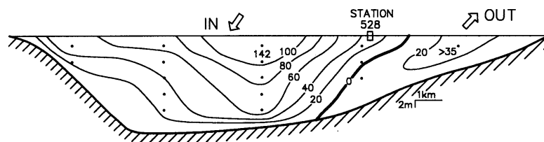
Figure 8 The velocity distribution in the Fehmarn Belt during inflow to the Baltic based on ship measurements from 15.00 to 16.30 on 27 June, 1977.
