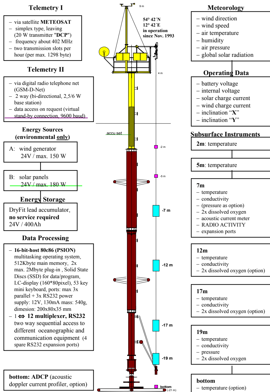
Figure 2 Baltic Station—DARSS SILL Mast
