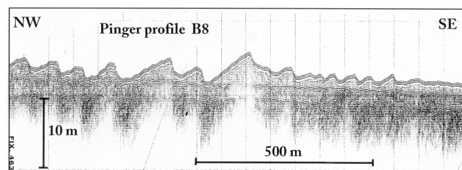
Figure 3 Pinger profile (B8) of sandwaves in the western part of Fehmarn Belt. Location indicated on Figure 1.
