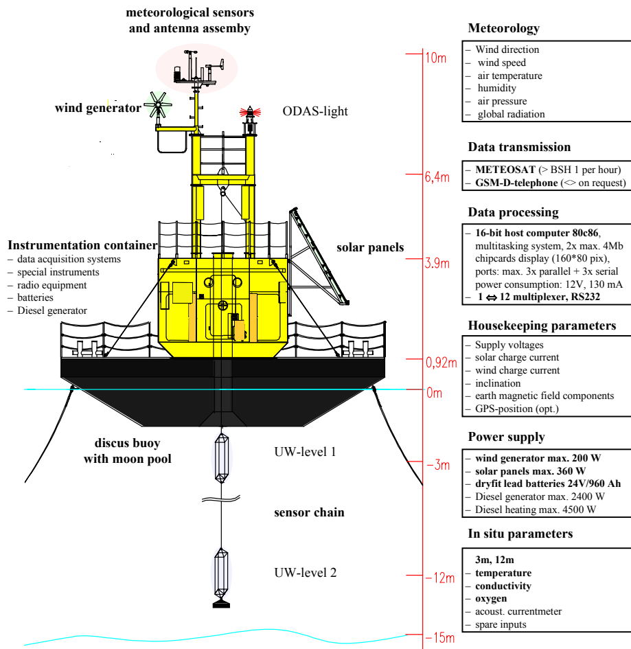
Figure 3 Discus Buoy at ODER BANK for monitoring of the exchange processes between the Pomeranian Bay and the Arkona Basin
