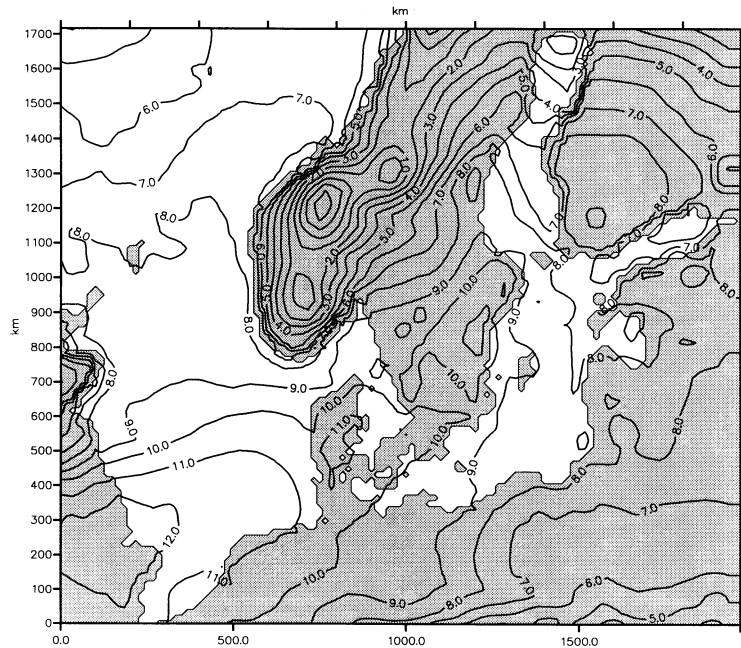
Figure 5 Example of air temperature distribution used in the heat exchange calculations (24 November 1994 00 GMT)
