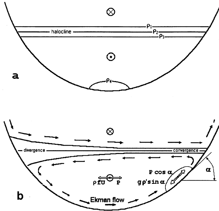
Figure 7 An explanation of the fan-like shape of isopycnals and northward displacement of the densest water pool from the deepest connection observed on transects across the Stolpe Furrow.
