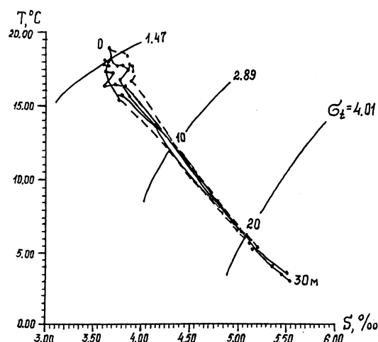
Figure 2 T, S -curves for stations of the Luga-Koporye polygon obtained from STD-sounding with vertical spacing z=2 cm
