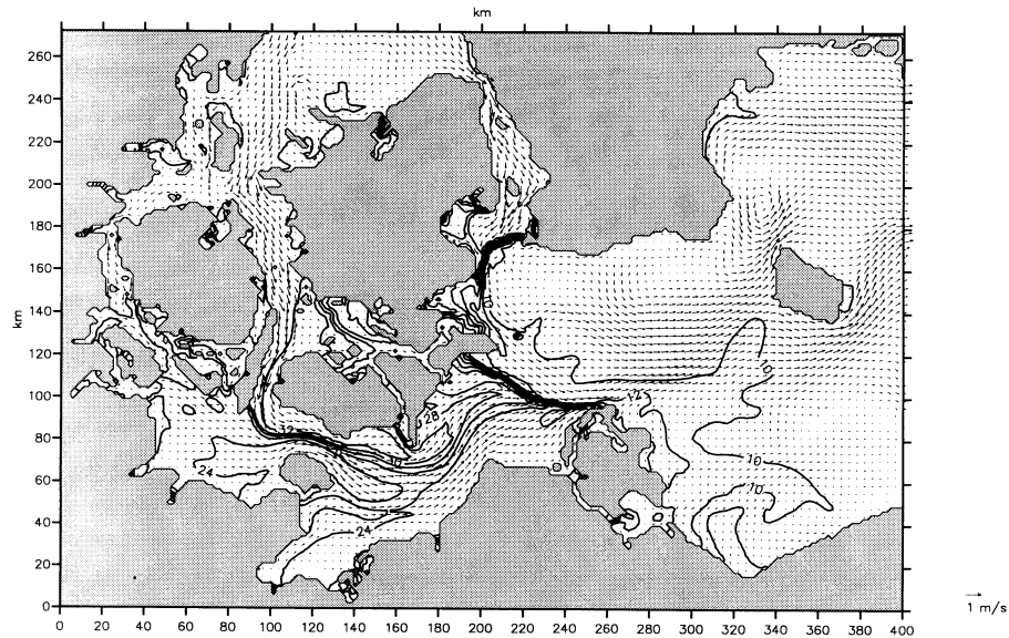
Figure 7 Calculated surface currents and salinities in 1 nm grid (24 November 1994, every second vector is shown)
