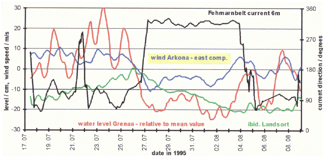
Figure 5 Time series of east component of wind velocity measured at the meteorological station Arkona (blue), sea level at Grenaa in the Kattegat (red) and Landsort in the Baltic proper (green), and direction of current measured in the Fehmarn Belt at a depth of 6m (black). Outflow from the Baltic Sea toward the Kattegat is about 310^\circ in the Fehmarn Belt.
