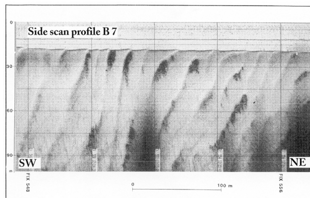
Figure 2 Side scan sonar image (B7) of sandwaves in the south-western part of Fehmarn Belt. Location indicated on Figure 1.
