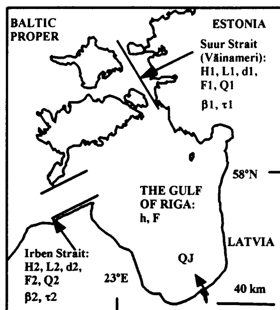
Figure 1 Plan of the Gulf of Riga and the model parameters
