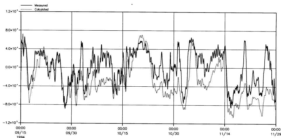
Figure 10 Calculated and measured discharge through Øresund (positive is outflow from Baltic Sea)
