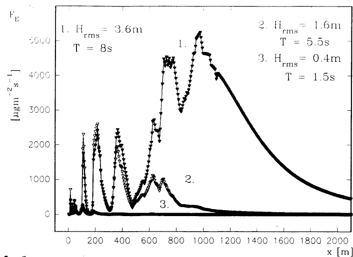
Figure 3 The aerosol emission flux obtained from model for three boundary conditions for the sea bottom profile in Lubiatowo
