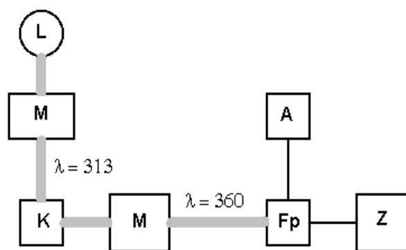
Figure 2 Layout of the measurement equipment (L—lamp; M—monochromator; K—chamber with the sample; Fp—photoelectric multiplier; Z—feeder; A—microamperometer).
