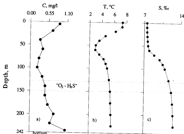
Figure 3 Vertical profile of suspension concentration in the Gotland Deep. Dotted lines show the geochemical “O 2 –H 2 S” barrier.
