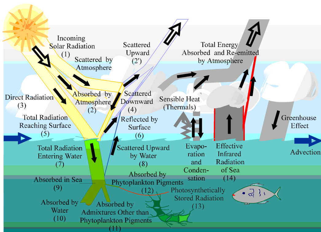
Figure 1 The main elements of energy balance in the atmosphere-sea system
