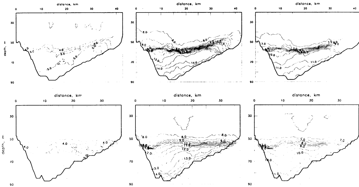
Figure 4 Temperature, salinity, and potential density anomaly vs. distance and depth for transects across the Stolpe Furrow (April 1923, 29th cruise of r/v “Professor Shtockman”). Top panels are from transect 1a and bottom panels are from transect 3a.
