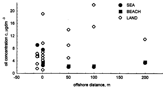
Figure 8 Concentration of hydrocarbons in seawater for different wind sectors: from sea, from land or along the coast.
