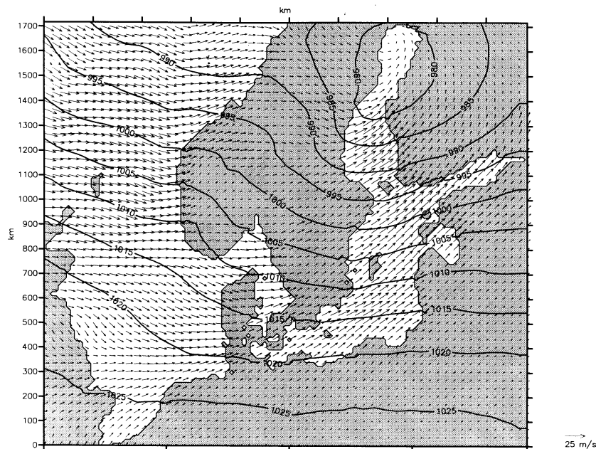
Figure 2 Applied Meteorological Forcing (Example from 24 November 1994, 00 GMT, every second vector is shown)
