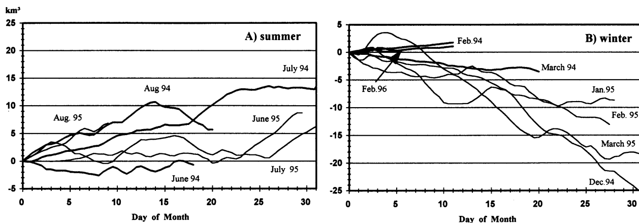
Figure 5 Integral volume transports grouped by seasons and months.
