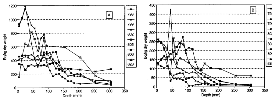
Figure 4 Radiometric profiles of sediment cores from the Gotland Basin. For location of sampling position see Figure 1.
