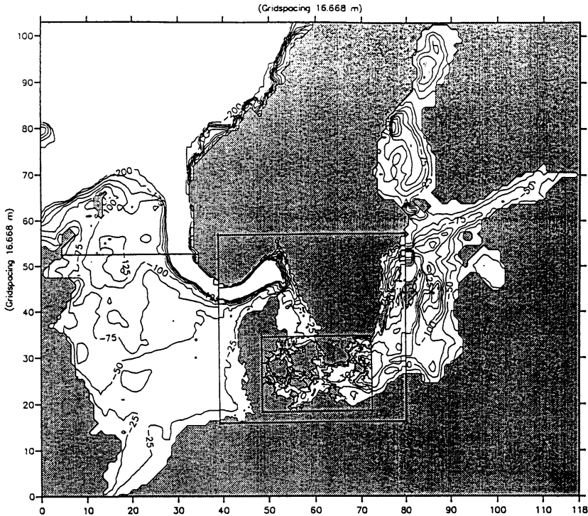
Figure 4 A numerical model bathymetry, covering the entire North Sea–Baltic Sea area has been compiled from echo sounding survey data and from navigational sea charts. The bathymetry has a resolution of one nautical mile and is based on more than 3 million data points.
