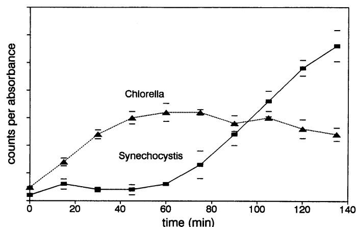
Figure 7 Kinetics of radioactively-marked phaeophytin labelling after increasing the irradiance from 25 to 260 \mu\text{mol photons m}^{-2}\text{s}^{-1} . The concentration of radioactively labelled phaeophytin at different time points after the beginning of the light stress is shown (disintegrations per absorption unit), with standard deviations for 4 samples. The algae were marked with \text{NaH}^{14}\text{CO}_3 6 h before the start of the experiment. For further details see Schubert (1996).
