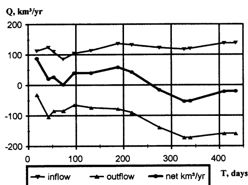
Figure 4 Evolution of the estimates of total in- and outflows and net exchanges depending on the lengthening of the direct measurements series in 1993–95
