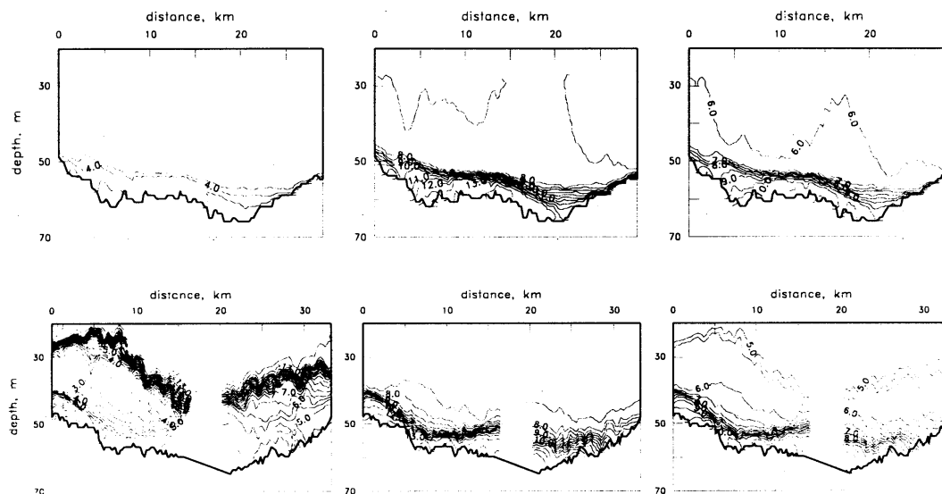
Figure 3 Temperature, salinity, and potential density anomaly vs. distance and depth in the western part of the Stolpe Furrow (over the sill). Top panels are from transect 2a (April 1993, 29th cruise of r/v “Professor Shtockman”), and bottom panels are from transect 1b/01b (September 1994, 33rd cruise of r/v “Professor Shtockman”)
