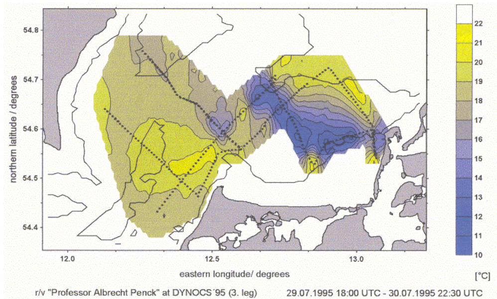
Figure 2 Distribution of sea surface temperature measured by the thermosalinograph of r/v “Professor Albrecht Penck”. The dotted lines mark the ship’s tracks.
