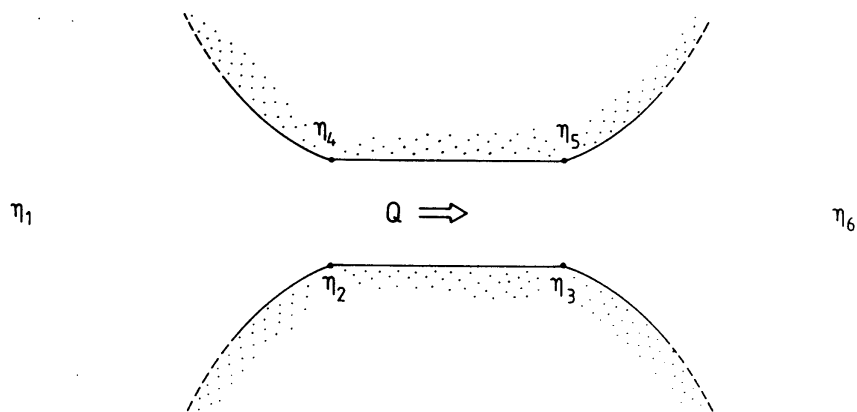
Figure 2 The sea level ( \eta ) at various positions in and outside a strait with flow rate Q = VHW
