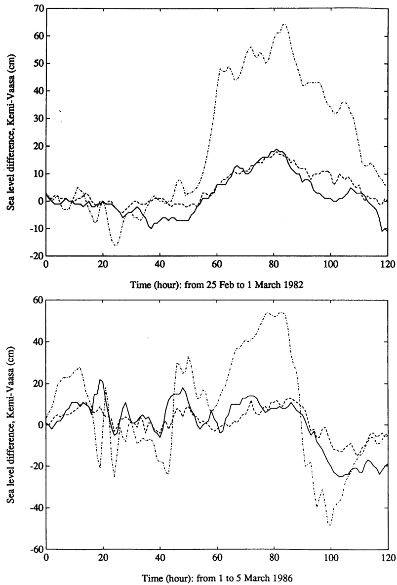
Figure 4 Time series of the water pile-up between Kemi and Vaasa. The solid line indicates observed data, the dashed line is from the coupled model and the dash-dot line is from the ice-free model.
