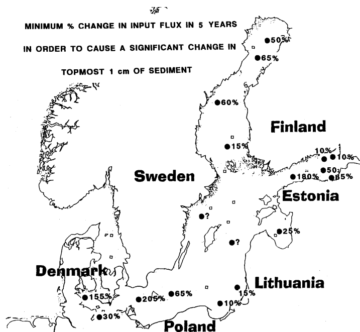
Figure 2 Result of sensitivity analysis based on evaluation of the Pb210 profile
