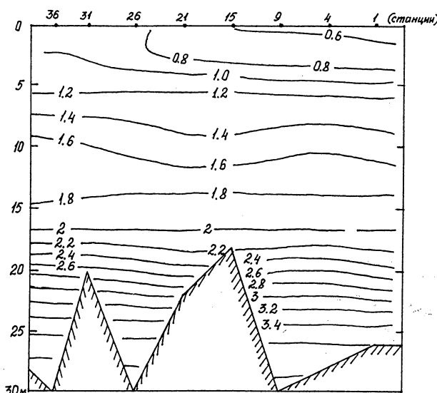
Figure 5 Distribution of density relation R_p = -E_T/E_S at the transect along the parallel of latitude 60° N (stations 36-31-26-21-15-9-4-1)
