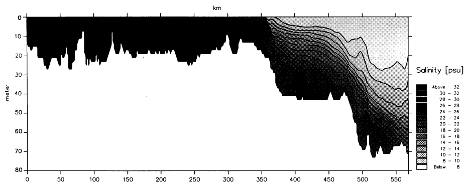
Figure 8 Vertical distribution of salinity along a line from Kattegat to Bornholm Basin (24 November 1994)
