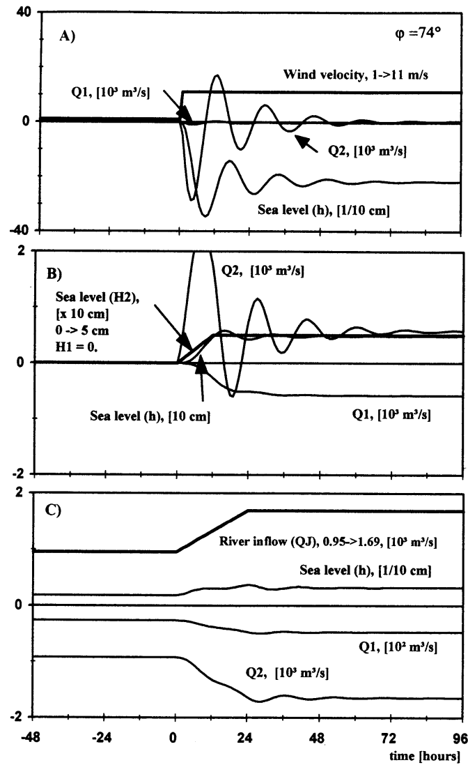
Figure 4 Some examples of model behaviour. Response of volume flows ( Q_i ) and sea level ( h ) to A) the increase in the wind velocity, B) open sea level H_2 (5cm for 12h) and C) river inflow.
