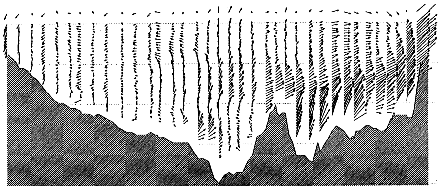
Figure 1 Example of measured current profiles along a transect crossing the Bornholm Strait at the entrance to the Baltic Sea
