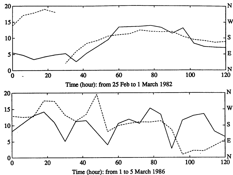
Figure 3 Wind speed (solid line) and direction (dashed line) for the two study cases
