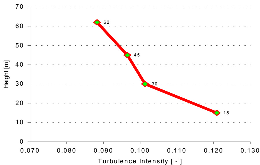
Fig. 2.6: Turbulence Profile at Horn's Reef [3].
