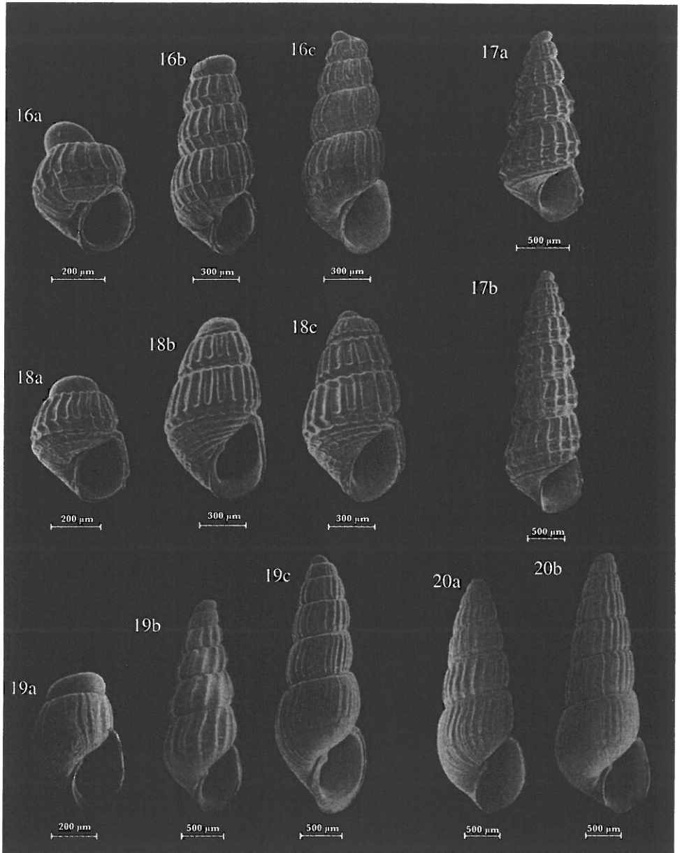
Fig. 16-20. Black Sea Pyramidellidae shells, Chrysallida spec. 16a-c, Chrysallida emaciata (Bulgaria, Ropotamo estuary); 17a-b, Chrysallida fenestrata (Ukraine, 20 km SW. of Sevastopol — ex coll. ZMRAS); 18a-c, Chrysallida incerta (Bulgaria, Ropotamo estuary); 19a-c, Chrysallida obtusa (a, Bulgaria, Djuni; b-c, Bulgaria, Ropotamo estuary); 20a-b, Chrysallida terebellum (a, Bulgaria, Ropotamo estuary; b, Bulgaria, Djuni).
