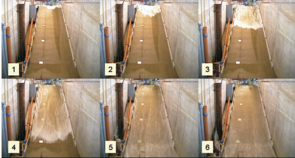
Fig. 5.40: Overtopping flow on the landward slope (Large Wave Flume, Hannover) (photo: SCHÜTTRUMPF)
