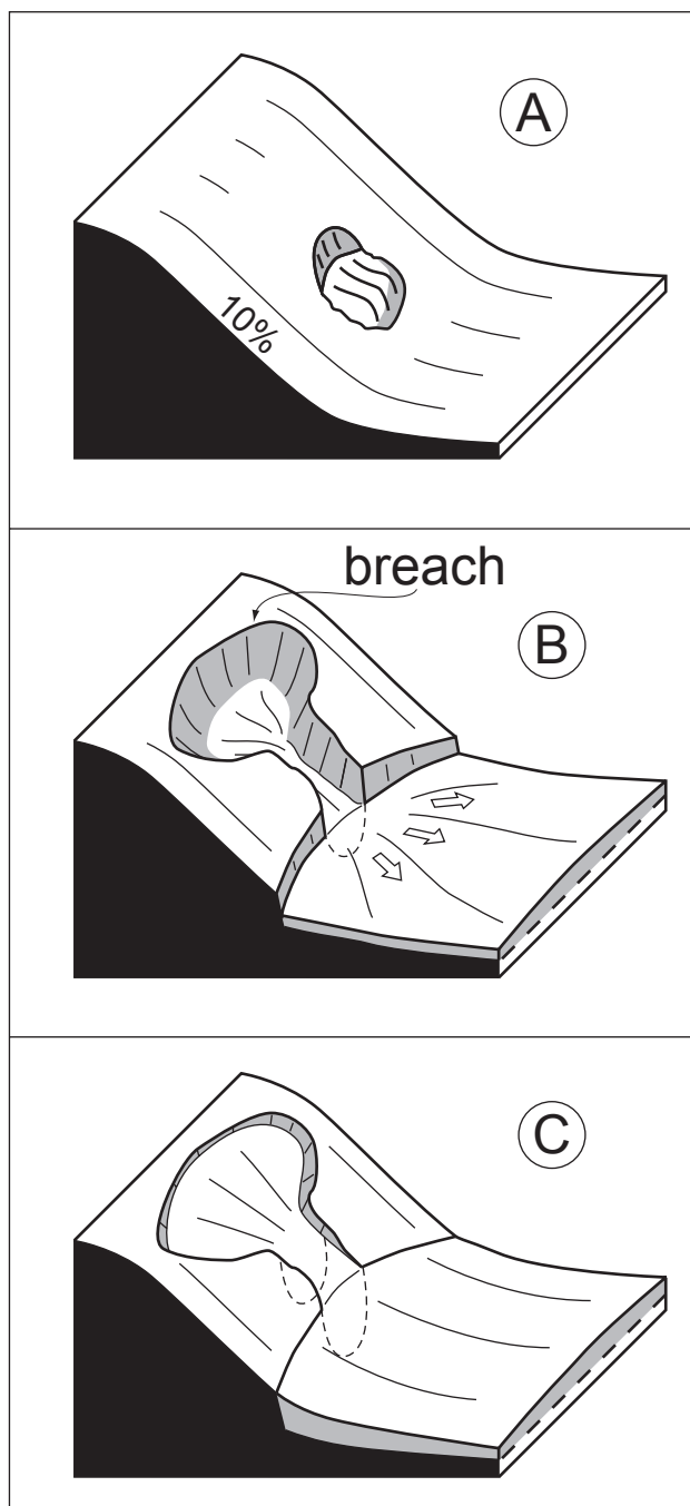
Figure 13. Processes reconstructed for explaining the observed facies M geometry fit well van den Berg et al. (2002)'s breach failure mechanism. Depicted is the western bank of the Brussels embayment. Slope angles are relatively steep as a result of continuous lateral accretion. A : some initial slope failure causes a small breach with vertical walls. B : the breach grows into the bank sediments. Slices of sand dropping from the receding walls create a high-density, sandy turbidity flow that cuts a canyon and quickly drops its load at the foot of the bank. C: the process goes on for some time, until the transport canyon is choked. A slope apron and a canyon fill of facies M have developed.
