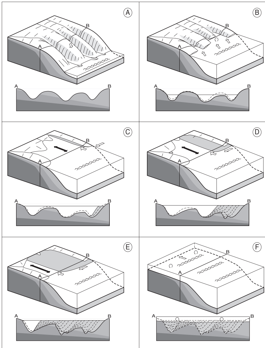
Figure 18. Sedimentary model for the Brussels Sands. The area represented is approximately the present-day Brussels Sands occurrence area, such as depicted in Fig. 1. The dimensions are schematic and not to scale. The view of the block diagrams is from NE. White arrows indicate net sediment transport, full arrows represent the tidal currents. The cross sections are East-West. In the cross sections, thick dashed lines represent the basin base at the previous step. A : consequent rivers drain into the North Sea. The sea-level fall Yp10 causes a forced regression and the rivers start to incise, creating a valley-and-interfluvium relief cut in the topographic slope near the shoreline. B : sea-level rises again. The sea enters the incised valleys, turning them into estuaries. Tidal erosion, probably assisted by wave erosion over the previous interfluvia, reworks the topography, pushing sediments inland and creating an estuary in the former incised valley area. C : near highstand, a tidal embayment is installed at the former incised valleys' location. Tidal currents continue to refashion the inherited morphology. Meanwhile, an important West-East sand transport path sets in under littoral drift at the North Sea shore west of the Brussels embayment. This path brings in a continuous supply of sand that
