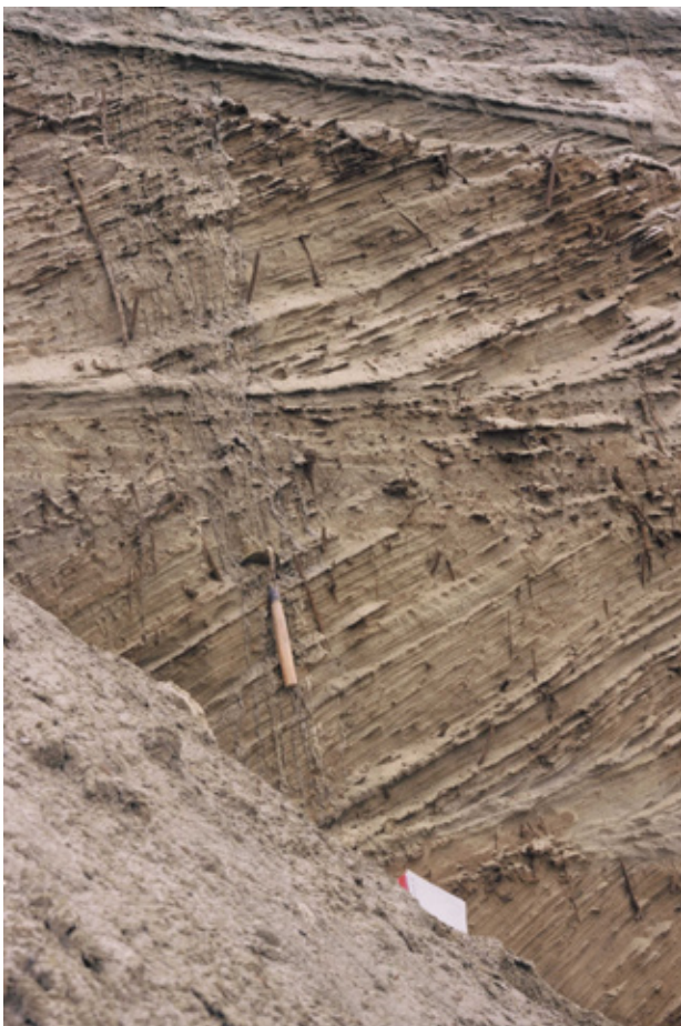
Figure 3. Facies X : thick cross beds, here in tabular beds. Note burrows of the Ophiomorpha type, either vertical or perpendicular to the foreset laminae. Bouillon sandpit, Haasrode, 1989. Scraping tool for scale is 40 cm long and the blade is 12.5 cm wide.
