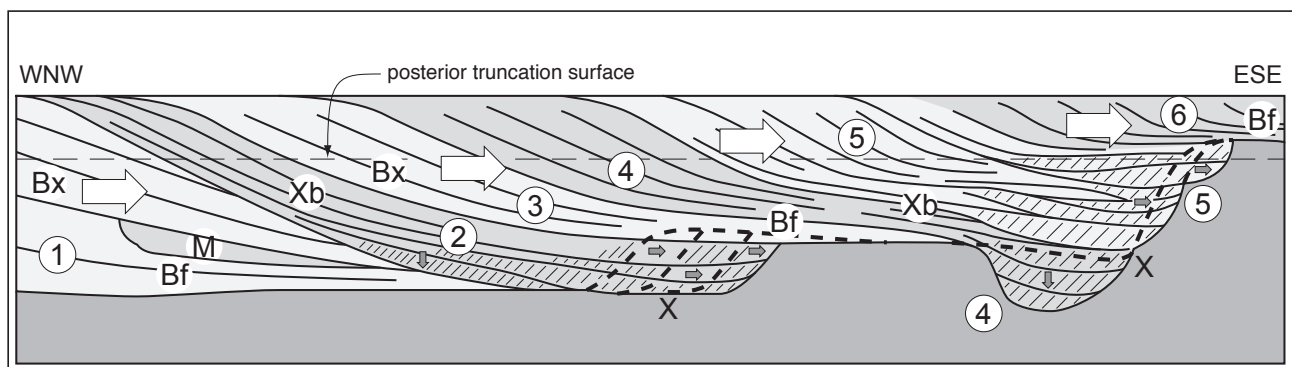
Figure 16. Profile resulting from different scales of hydraulic flow-section restriction. Thick white arrows represent the westerly lateral accretion. Small shaded arrows indicate the lateral and vertical erosion caused by flow-section restriction. This figure reads from left to right. Shades in the Brussels Sands fill indicate the following steps : 1: the continuing accretion from WNW to ESE causes the Brussels Sands basin to fill rapidly. The resulting westerly lateral accretion consists predominantly of facies Bf, Bc, Bx and M. 2: caused by the sedimentation and the inherited fluvial incision morphology (thick dashed line), a locally restricted flow section arises near the bottom. The flow is locally enhanced and cuts both vertically and laterally (shaded arrows). Sedimentation from the West outpaces the locally created accommodation space. Thick cross beds are the rapid filling of the created space. 3: the westerly lateral accretion, which never ceased to function, causes the westerly arrangement to roll over the filled local channel. Facies Bf covers directly facies X. 4 and 5: sedimentation from the WNW continues and the flow section is now seriously restricted as a high inherited morphological feature is met. Now, vertical incision is more important than lateral erosion. Again, sedimentation outpaces creation of accommodation and the scour pit is filled rapidly with thick cross beds. 6: while the embayment is not entirely filled, the westerly lateral accretion continues to function. Due to posterior truncation, these particular sediments are no longer present (e.g. in Bierbeek, Fig. 14C).
