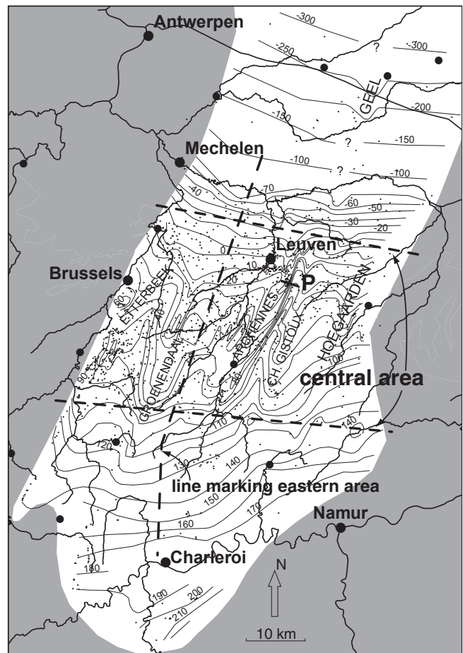
Figure 2. 10-metre contour lines of the Brussels Sands base surface (50-metre interval below -70 m TAW/DNG). Map updated from Houthuys (1990, fig. 4.5). Dots represent data density for updated part of map. Thick lines indicate subareas. The central area (indicated by short-dashed lines) has only an indicative boundary. This area has pronounced scour structures in the base surface, relatively coarse-grained sand, and the M facies intercalations are only found here. The eastern area (bordered by the long-dashed line) has coarse glauconite at the base and has a greater abundance of thick cross beds than the area west of the line. The bold, short line near “P” indicates the profile of Fig. 14.
