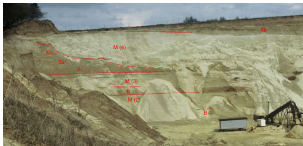
Figure 10. The Alconval sandpit in Braine-l'Alleud showed 5 stacked units of facies M, three of which can be seen in this picture taken in 1994. Note incision of M(4). Sandpit face is about 30 m high and oriented N (left) -S (right).
