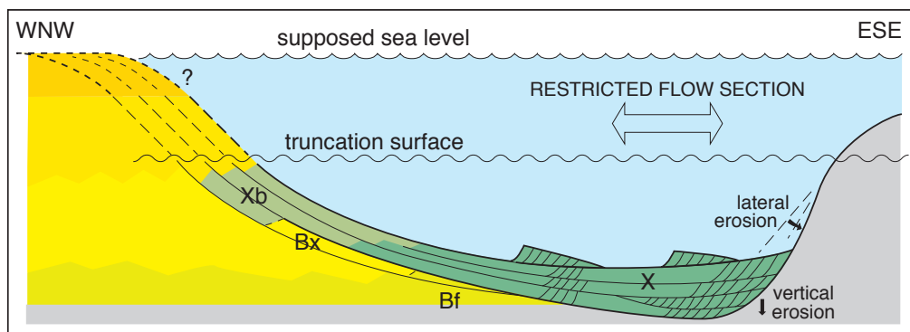
Figure 15. General layout of the “closure arrangement” at an eastern submerged paleorelief scarp in the base of the Brussels Sands. Main flow direction is SSW-NNE, perpendicular to the profile. The truncation surface is posterior to the deposition of the Brussels Sands.
