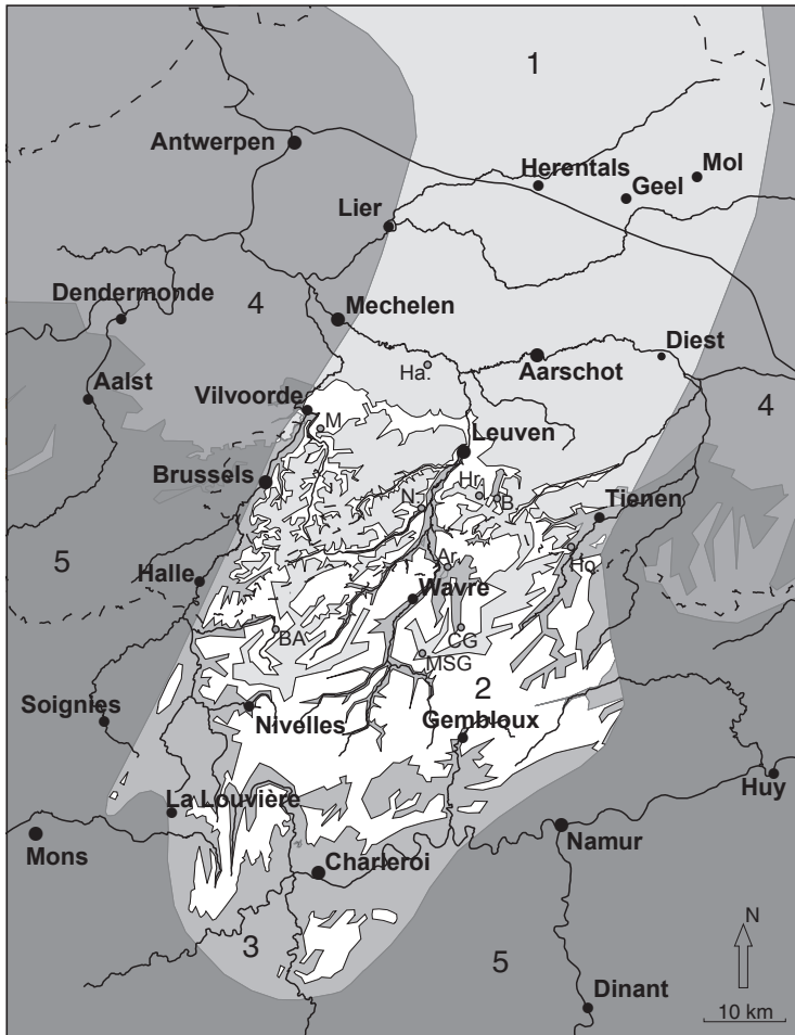
Figure 1. Occurrence of the Brussels Sands in Central Belgium. 1 = subcrop; 2 = outcrop; 3 = eroded outcrop; 4 = no Brussels Sands, with younger cover; 5 = no Brussels Sands, older outcrops. Brussels Sands basin = 1 + 2 + 3. Localities mentioned in text and captions : Ar: Archennes; B: Bierbeek; BA: Braine-l’Alleud; CG: Chaumont-Gistoux; Ha: Haacht; Ho: Hoegaarden; Hr: Haasrode; M: Machelen; MSG : Mont-Saint-Guibert; N: Neerijse.
