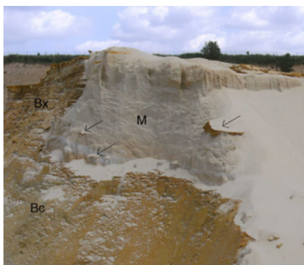
Figure 7. Erosive incision filled with well-sorted, massive sand (facies M). The massive sand embeds lumps (arrows) eroded of adjacent layers that consist here of facies Bc grading vertically into Bx. Note irregular erosive contact showing nearly vertical wall in upper part of the section. Exposed section is approximately 6 m high. Hoslet sandpit, Chaumont-Gistoux, 2009.
