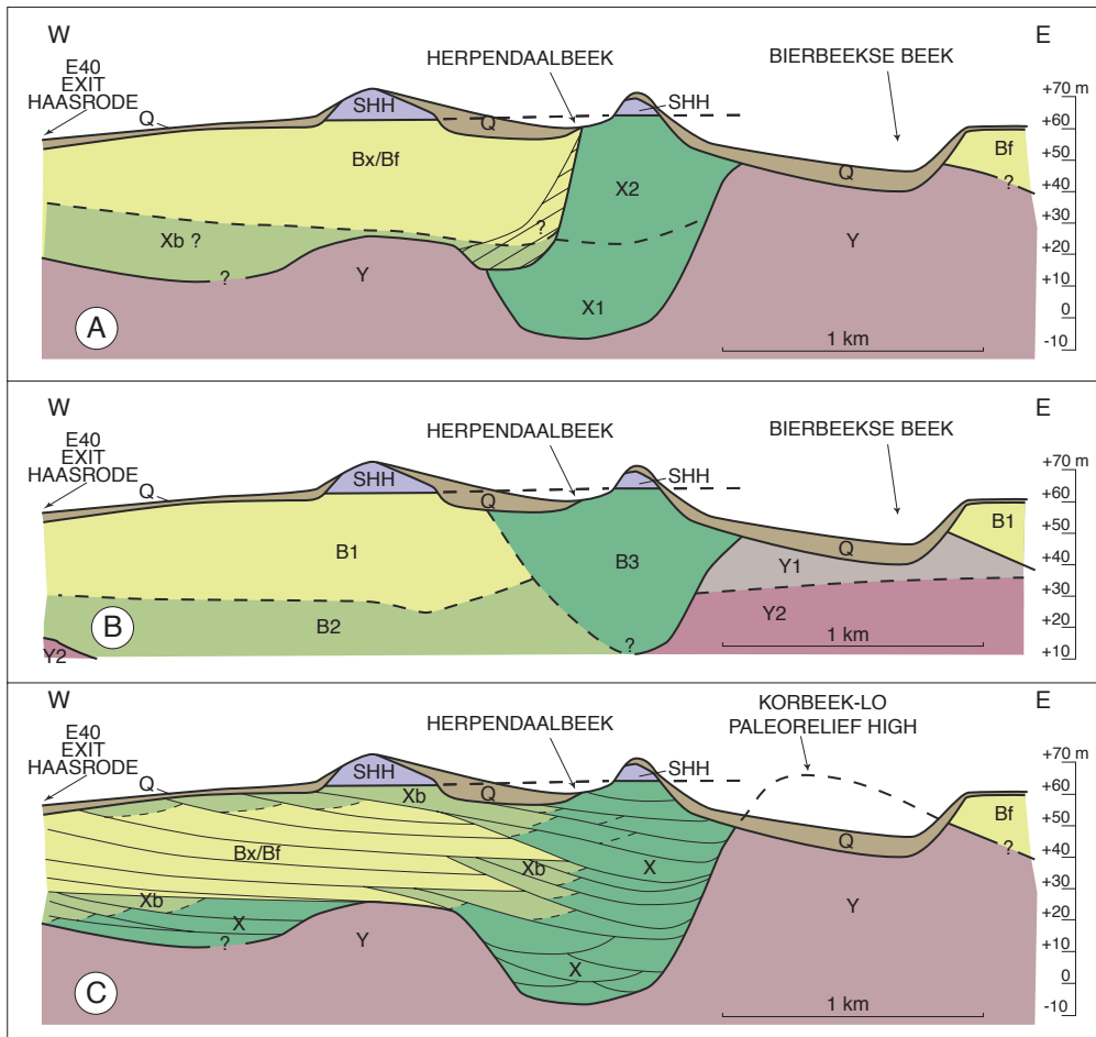
Figure 14. Successive interpretations of a profile situated along the E40 motorway SE of Leuven (position : see Fig. 2). A : interpretation by Houthuys (1990). B : interpretation by De Geyter for Tucrail NV/SA (1993, unpublished). C : author's current interpretation. Y, Y1, Y2: deposits of pre-Brussels Sands Ypresian age. SHH: Sint-Huibrechts-Hern Formation, base Oligocene. Q: Quaternary sandy löss and alluvial and colluvial deposits.
