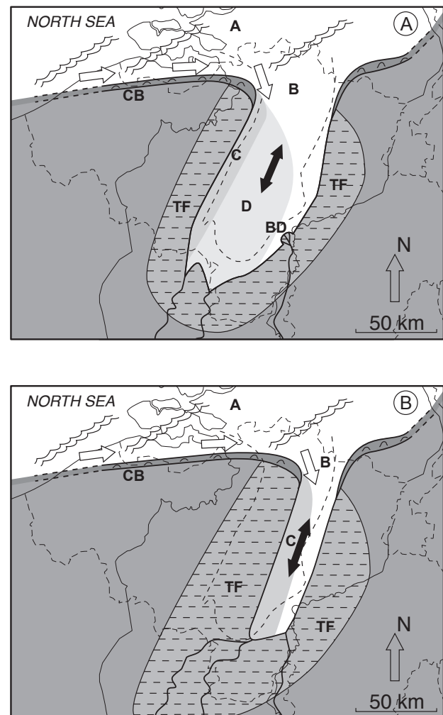
Figure 17. Inferred paleogeography during deposition of the Brussels Sands. (A) : during initial highstand with beginning sedimentation at west shore of tidal embayment; (B) near closure of the tidal embayment. Explanation of letters : A : open sea; waves and wind from sector W-NW causing west-east littoral drift; B : relatively narrow entrance to bay shelters it from swell; C : area of rapid sand deposition in westerly lateral accretion arrangement; D : area of slow deposition of fine sand and carbonate mud; BD : bayhead delta; CB : coastal barrier and beach; TF : tidal flats and marshlands; white arrows : sediment transport; black arrows : tidal currents in embayment. Darkest shade is wooded flat lowland. All areas and lines outside preserved Brussels Sands basin are indicative. Present-day national boundaries, North Sea coast and main rivers for reference.
