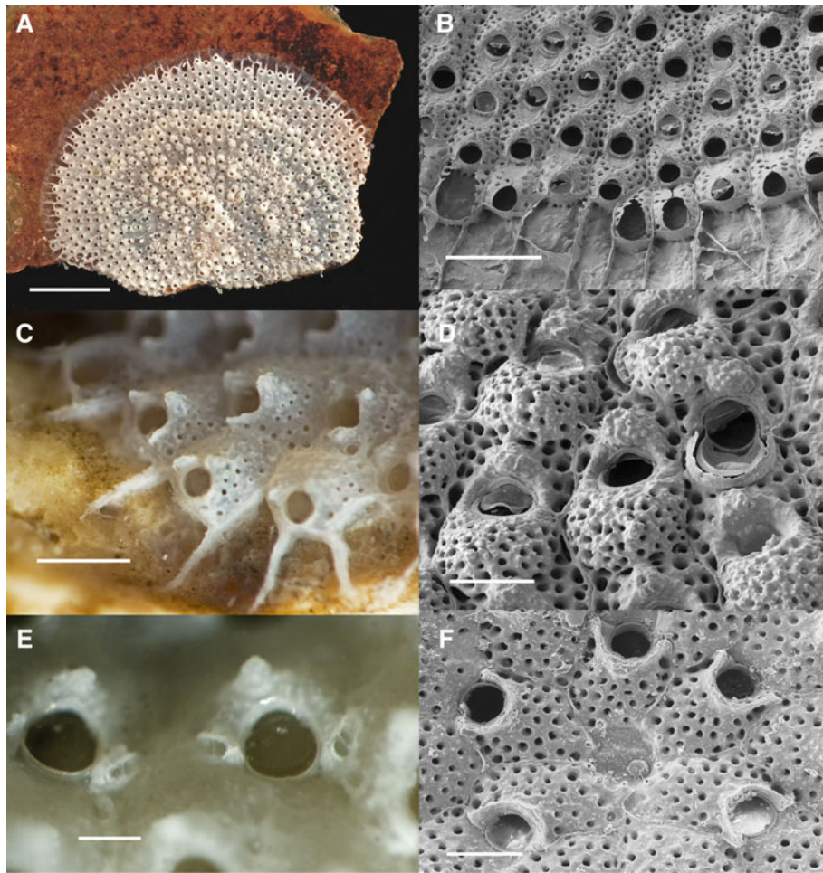
Fig. 1. Schizobrachiella verrilli (Maturò & Schopf, 1968): A, C, E: preserved material from Tiefe Rinne, Helgoland. B, D, F: SEM preparations of Belgian material. (A) Mature colony on shell fragment; (B) Detail of colony; (C) Zooids with prominent umbo and lateral flappets; (D) Zooids with ovicells, one ovicell under construction; (E) Two zooids with avicularia on either side of the operculum; (F) Centre of young colony with ancestrula showing remnants of spines. Scale bars: A, 3 mm; B, 500 µm; C, 300 µm; D, 200 µm; E, 100 µm; F, 200 µm.
