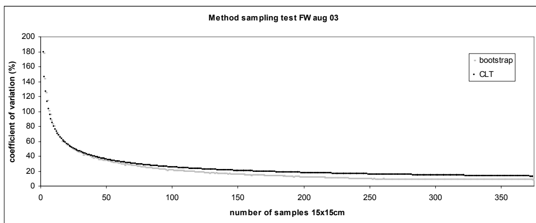
Figure 7: The coefficient of variation in relationship to the number of samples taken within the dataset: bootstrap output and output obtained by the central limit theorem of fresh weight biomass (FW) within the method test section.
