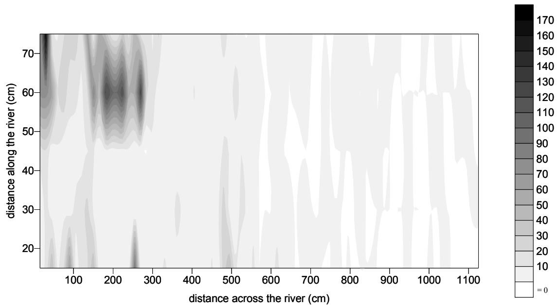
Figure 5: Fresh weight total biomass (expressed in g/225cm 2 ) in the method test section: surfer diagram (top view).
