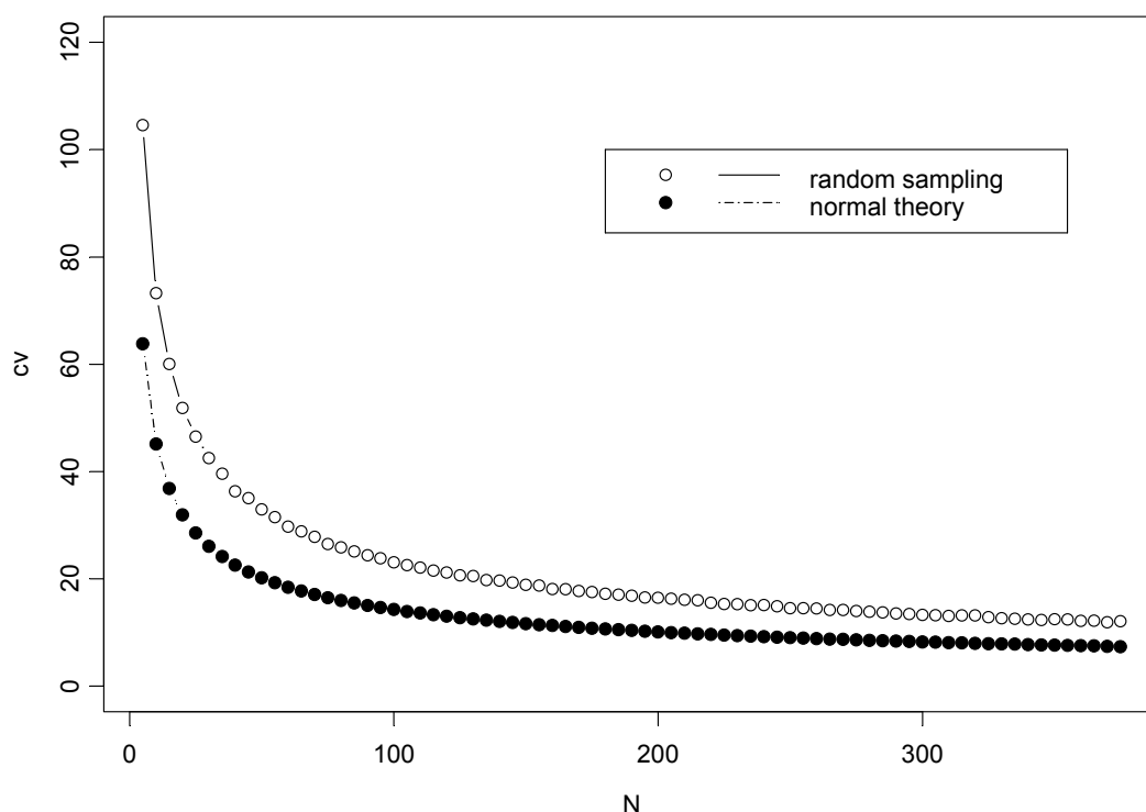
Figure 10: Bootstrap outputs with extra condition factor. Relationship between coefficient of variation in % (CV) and number of samples (N) for fresh weight biomass within the method test section. (◇) "Random sampling": random sampling occurs with equal sampling within the five subblocks. (●) "Normal theory": random sampling with equal sampling within the five subblocks, assuming data are normally distributed.
