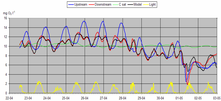
Figure 55: Model results, run 1 (22 April – 3 May 2004) Solar irradiance (Light) is given in arbitrary units, for the purpose of daily comparison only. Csat is the oxygen saturation concentration for the mean temperature observed.
