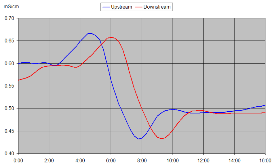
Figure 52: Propagation of a concentration front through the test reach (May 1, 2004)
