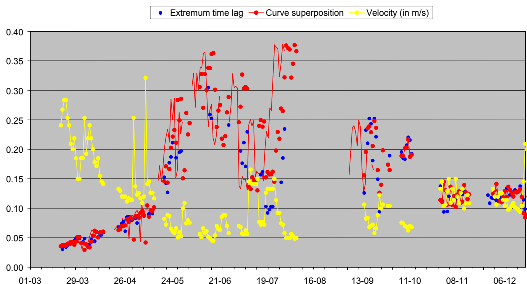
Figure 53: Seasonal evolution of the Manning roughness coefficient in 2004. Values have been obtained using a curve superposition technique (red dots, daily average) or by measuring the time lag between marker events (blue dots, instantaneous values). The mean daily velocity is also shown.
