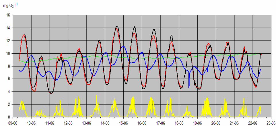
Figure 57: Model results, run 3 (9 June – 23 June 2004)
