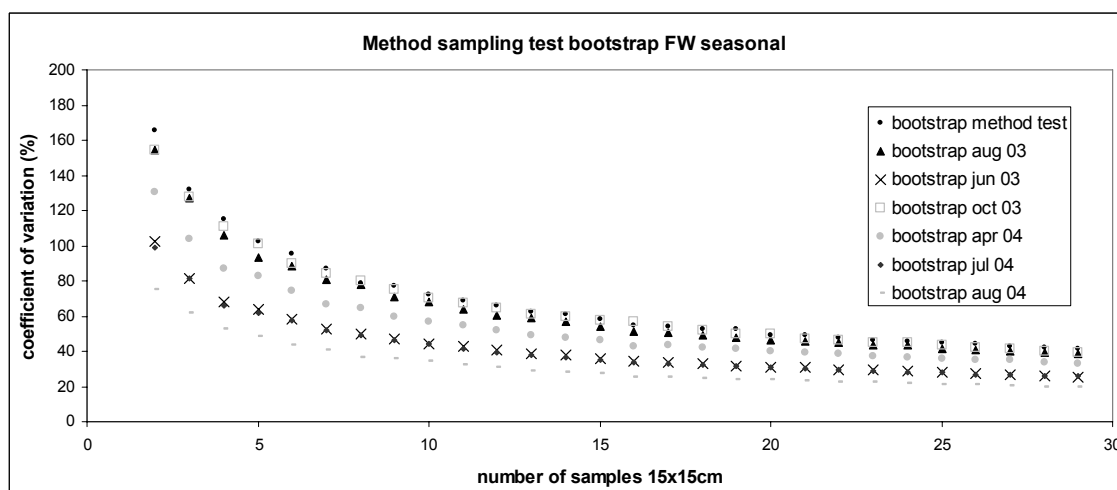
Figure 9: Coefficients of variation generated by bootstrapping fresh weight standing biomass. Results of the method test section are compared with the monthly taken 30 samples of biomass in different seasons.
