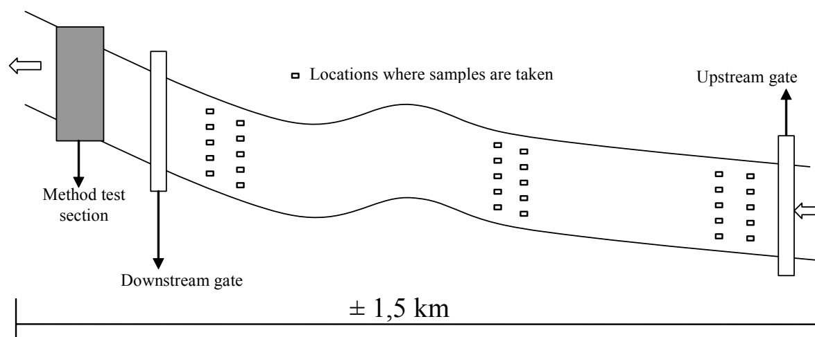
Figure 8: Schematic presentation of the section between the two adjustable weirs on the river Aa.
