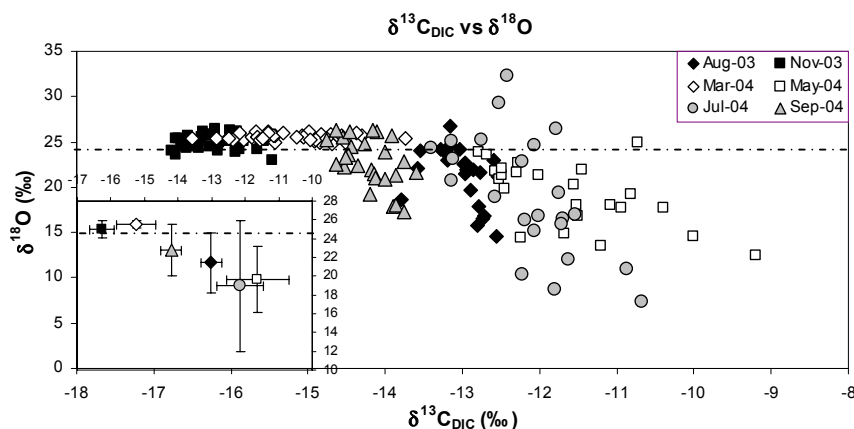
Figure 28. Seasonal variation in the \delta^{13}\text{C}_{\text{DIC}} and \delta^{18}\text{O}_{\text{DO}} composition in the Aa River 2003-2004. The insert shows the mean ( \pm SD) of all months. The dashed line represents the \delta^{18}\text{O}_{\text{DO}} value for a situation where \text{DO} is in equilibrium with air \text{O}_2 (24.2‰).
