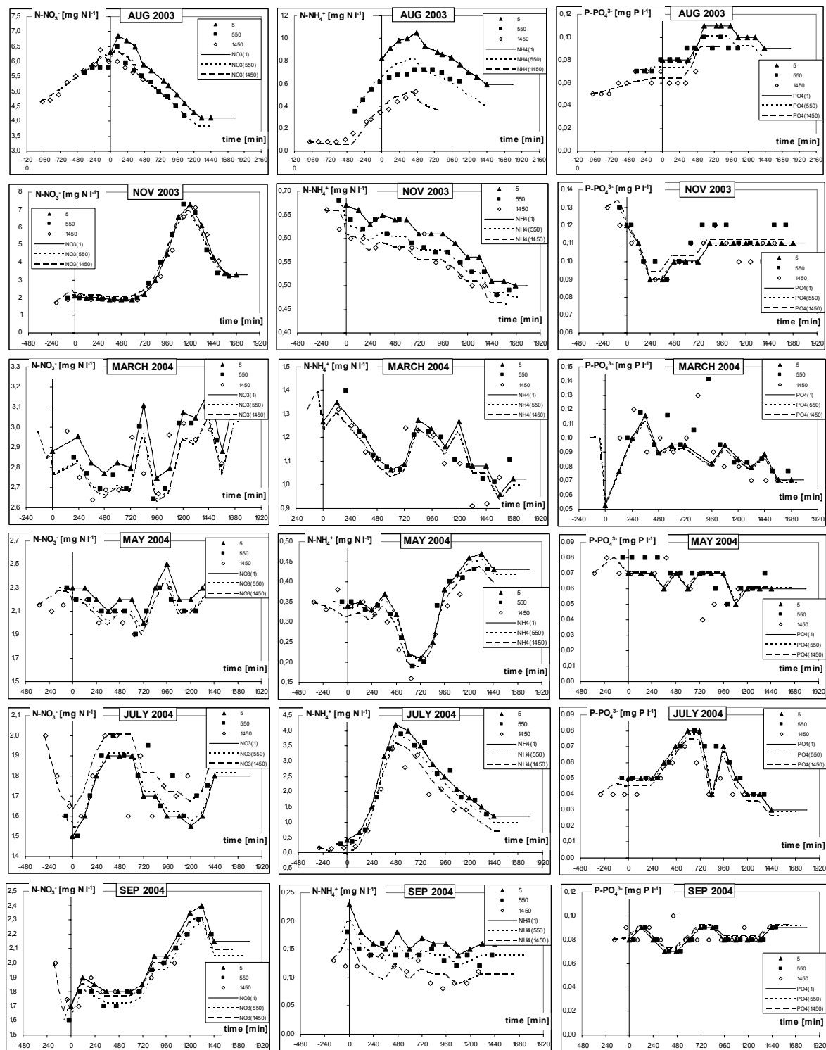
Figure 22: N-NH 4 + , N-NO 3 - and P-PO 4 3- values [mg l -1 ] at the upstream weir (▲), in the middle (■) and at the downstream weir (○) for the six campaigns plotted against relative time [min].
