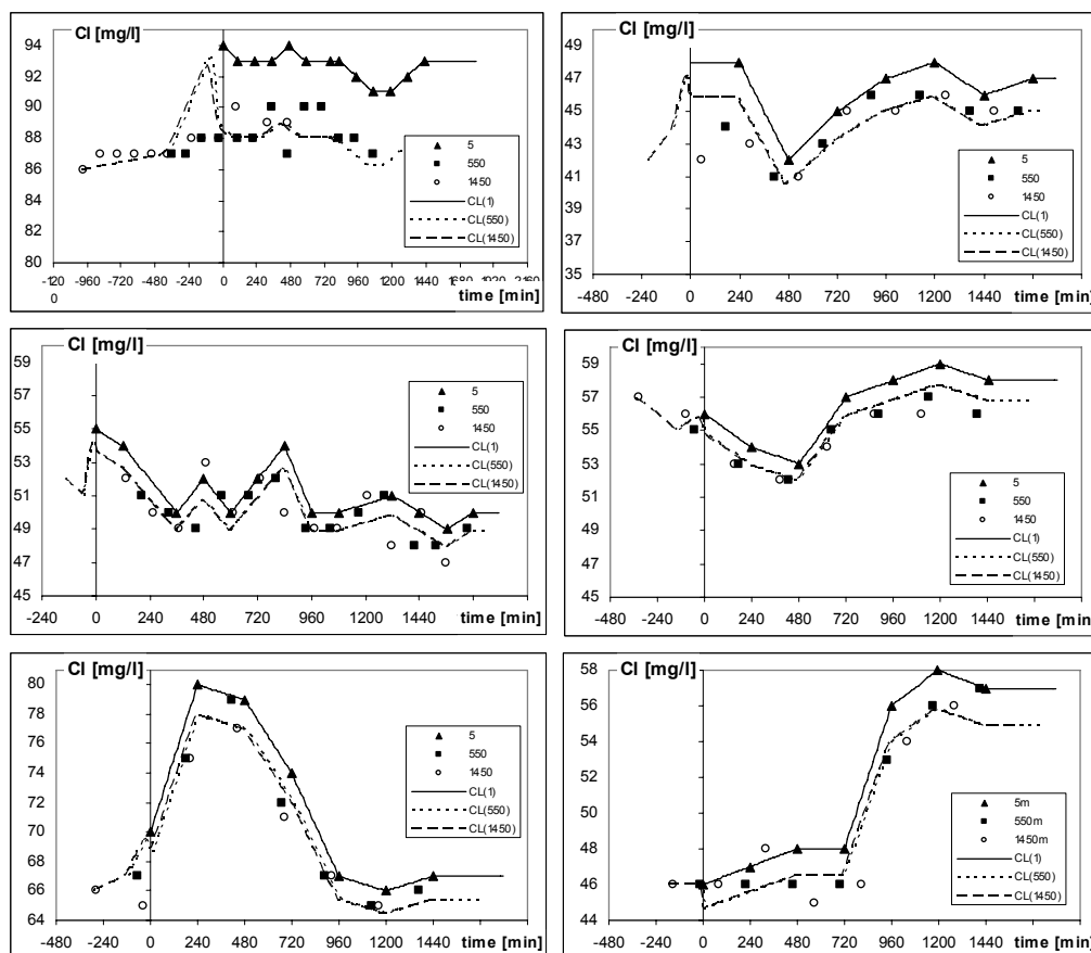
Figure 21: Tracer chloride values [ \text{mg l}^{-1} ] at the upstream weir (▲), in the middle (■) and at the downstream weir (○) for the six campaigns plotted against relative time [min]. Accordingly, the behaviour of one water package is shown. Dotted lines represent chloride values obtained by modelling the dilution originating from the Sloopbeek only in the middle (..... CL(550)) and at the downstream weir (— CL(1450)).
