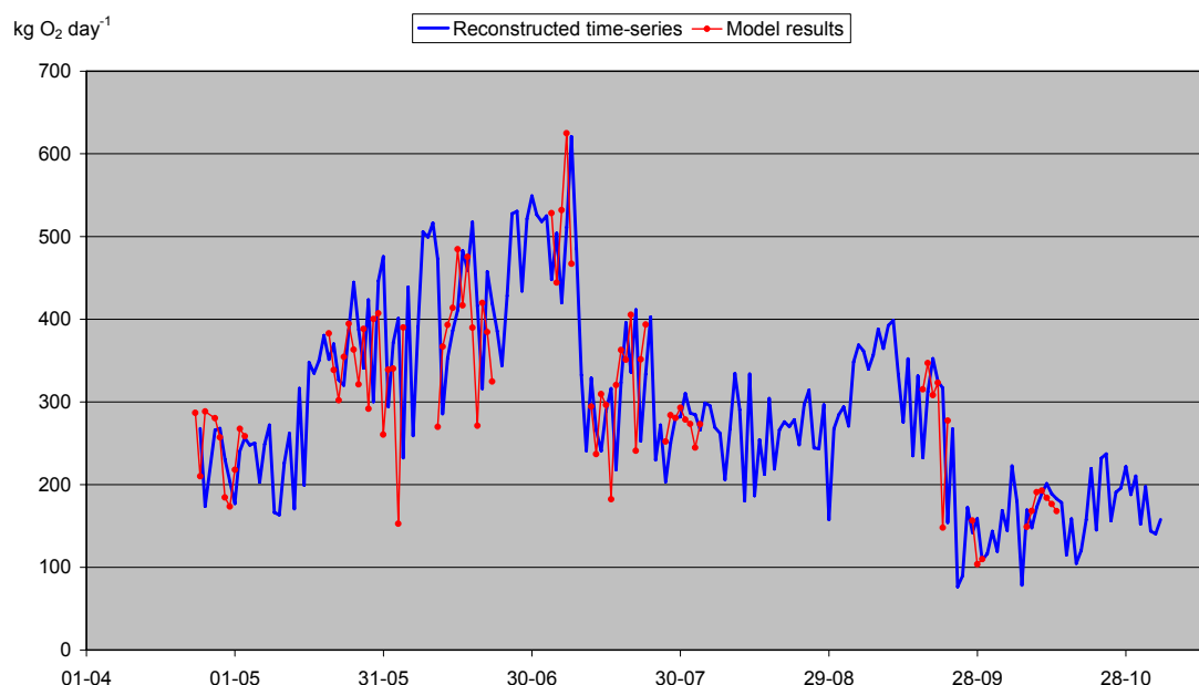
Figure 66: Reconstructed time-series of the daily oxygen production.
