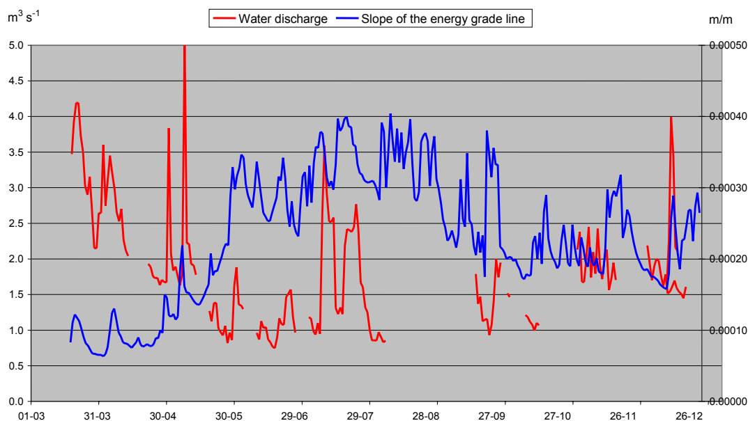
Figure 54: Seasonal evolution of the water discharge and of the slope of the energy grade line (2004)
