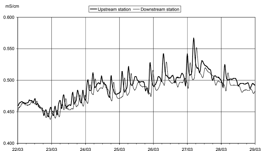
Figure 51: Specific conductivity at the boundaries of the test reach – Week 13, 2004.
