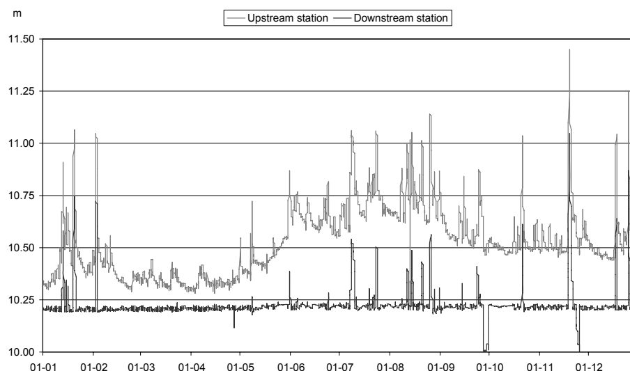
Figure 50: Water surface elevation at the boundaries of the test reach during the year 2004.
