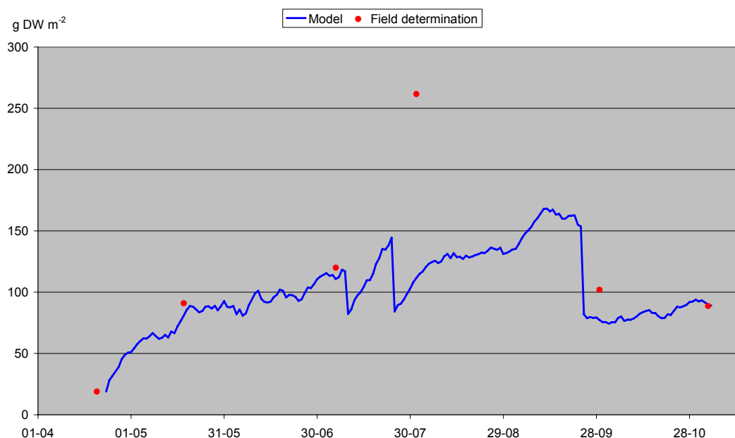
Figure 67: Computed vs. observed macrophyte density.
