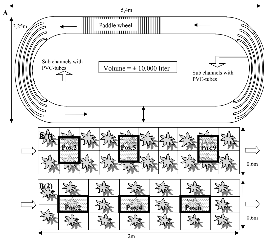
Figure 33: (A) schematic presentation of the flume (top view) and (B) schematic presentation of the arrangement of 20 pots with macrophytes in the test section for (1) Callitriche platycarpa and Potamogeton natans and for (2) Sparganium erectum . \star = macrophytes in each pot. The black rectangles with biomass were selected to analyse ^{15}\text{N} in the biomass standing in the different locations in a patch.
