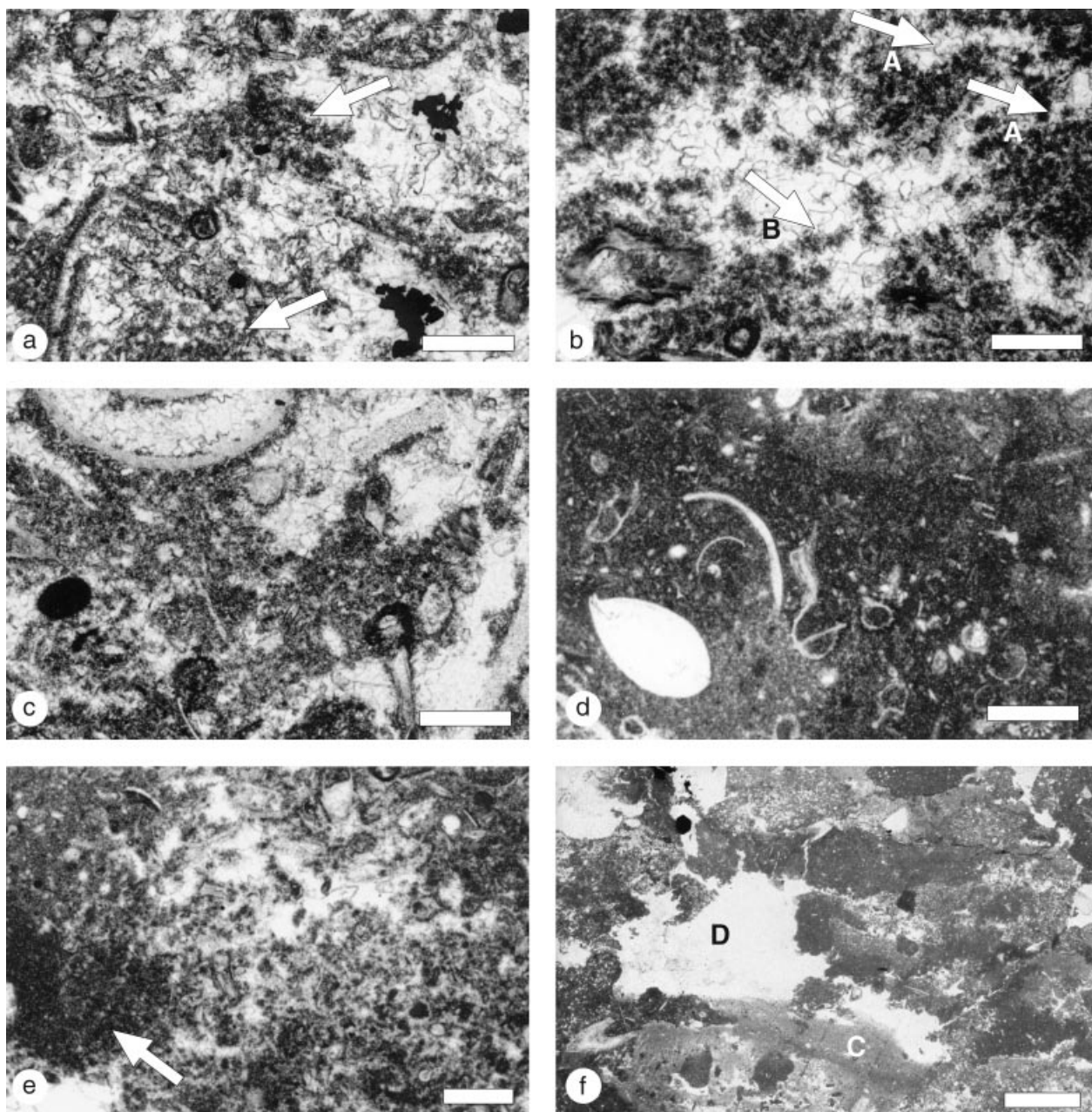
Fig. 2. Features of the precursor mud types and initial polymuds, shown in plain polarized light micrographs. Scale bar = 500 \mu\text{m} in (a)–(e) and 2 mm in (f). (a) Grumous Type 1 (arrows), Knockadrum. (b) Grumous Type 2, Knockadrum: note the sparry fenestrae and their flat floors (arrowed A) with no distinct geopetal sediment, and the rods of grumous fabric (arrowed B) suggesting calcification of microbial filaments (cf. Monty, 1995, fig. 19B). (c) Grumous Type 3, Knockadrum: the large bioclast at top left is a worm tube. (d) Non-grumous wackestone with ostracods and other skeletal debris, Dunmore. (e) Gradation from grumous Type 2 mud (occupying most of field of view) to grumous Type 3 and then to non-grumous mud on left (arrowed), Dunmore. (f) Very early development of polymud fabric at the base of the bank at Hill 707. Note that non-grumous muds are more important than grumous ones. Voluminous geopetal sediments (C) are capped by a final cavity fill of non-fibrous cement (D). The cracking of the non-grumous muds forming the roof of this cavity, together with the small mud clasts in the geopetal sediment below, demonstrate the coherent nature of the muds at an early stage (similar features from a comparable position were illustrated by Miller, 1986, fig. 4A). Such marked cracking may result from the absence of crypto-fibrous cement, characteristically the early cavity-filling fabric, which only appears about 40 cm higher in the bank.
