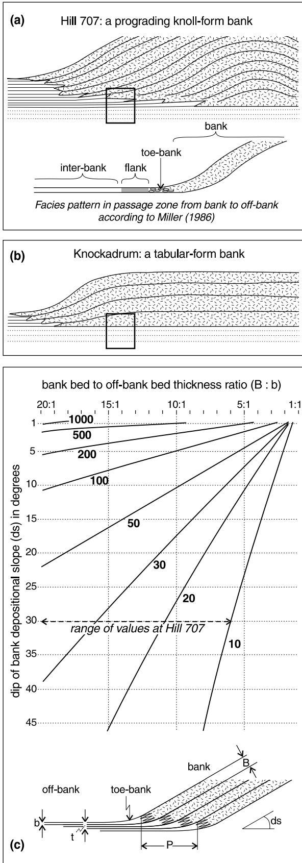
Fig. 8. (a) The upper diagram shows a schematic vertical cross-section through part of a prograding knoll-form bank as displayed at Hill 707. From the position of the studied section (rectangle), it is evident that the beds immediately underlying the bank are the off-bank lateral equivalents of a slightly earlier stage of bank growth. The lower diagram indicates the terminology used by Miller (1986) for the facies developed in the lateral passage from bank to off-bank (his 'inter-bank'). (b) Schematic vertical cross-section through part of a tabular-form bank such as that at Knockadrum. The beds immediately below the bank in the studied section (rectangle) are not the lateral equivalents of bank beds, and the transition facies cannot be explained by progradation. (c) The relationship between the thickness of transition facies beneath a Waulsortian bank and uniform bank progradation. The numbered curves indicate the progradation (P, in cm) required to develop laterally equivalent off-bank beds (t) 1 cm thick. For example, to produce a 1-m-thick transition facies with a sedimentation ratio of 15:1 and a bank slope of 35° requires about 25 m of progradation. The range of values for Hill 707 is indicated. As the transition facies represents a traverse from the edge of the aureole to the bank margin, the progradation distance equals the width of the aureole. Variables are the depositional slope (ds) of the prograding bank margin and the ratio of the thickness of laterally equivalent individual beds in the bank and off-bank (B:b). Note that combinations of very low depositional slopes and high bank/off-bank thickness ratios are not sustainable, as the depositional slope necessarily increases.
