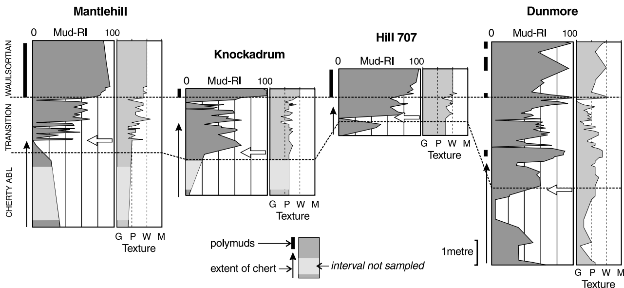
Fig. 7. Stratigraphic plots of the Relay Index of mud characters (Mud-RI) for each locality. Limestone texture and the stratigraphic extent of chert are shown for comparison. The correlation lines across the figure indicate the facies boundaries based on field evidence; the open arrows mark the base of the transition facies based on mud characters. G, P, W and M = grainstone, packstone, wackestone and mudstone. Note the zig-zag increase in Mud-RI through the transition facies at Mantlehill and Hill 707. At both localities, this is preceded by a drop in RI to near zero. Knockadrum shows quite a different pattern as there is no initial drop, and the trend up-section shows a decrease in average RI. The RI curve at Dunmore is much more irregular.
