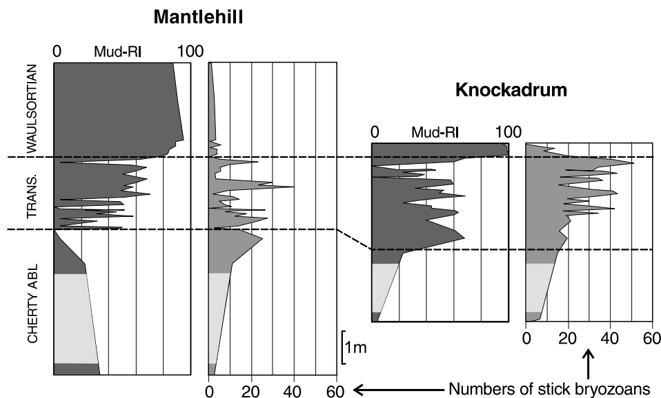
Fig. 12. Numbers of stick bryozoans at Mantlehill and Knockadrum and their relation to the characters of precursor muds (as represented by the Mud-RI). Note the broadly inverse relationship between the Mud-RI and bryozoan numbers in the transition facies. The term 'bryozoan numbers' expresses the number of individuals counted per thin-section standardized to an area of 10 cm 2 .
