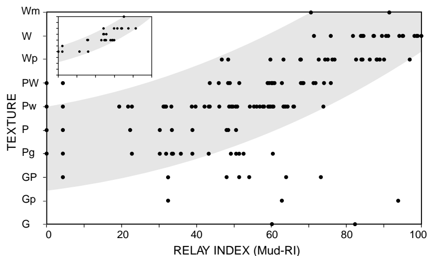
Fig. 6. Relay Index of mud characters (Mud-RI) plotted against limestone texture for all samples. 90% of them lie in the shaded area showing a broad trend of increasing muddiness with increasing RI, i.e. with increasing complexity of the precursor mud system culminating in the Waulsortian polymuds. This trend is also evident when samples of the transition facies are considered alone (see inset: Mantlehill). Samples outside the main trend, mainly from Dunmore, are grainy rocks in which the muddy masses are too small to influence the textural classification. G, P, W and M = grainstone, packstone, wackestone and mudstone. Intermediate texture codes indicate the presence of more than one category and their relative importance: for example, in Gp, the packstone component is subordinate to grainstone, whereas in GP, the proportions are equal.
