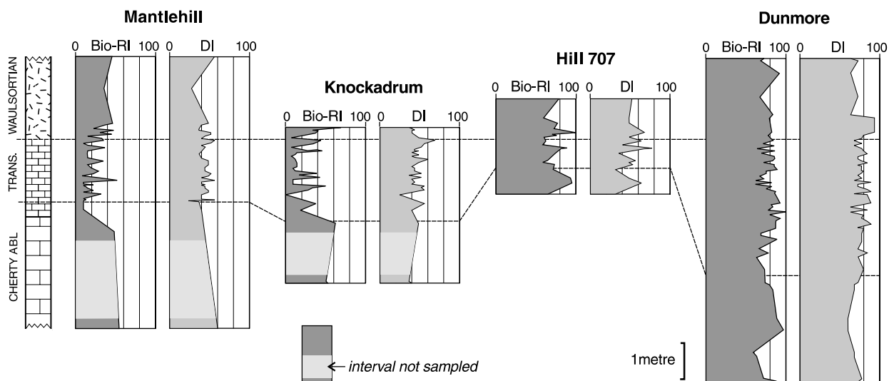
Fig. 14. Stratigraphic plots of Relay Index (Bio-RI) from correspondence analysis of skeletal grain-types (see Fig. 13) together with logs of the Diversity Index (DI). The latter records, as a percentage, the number of grain-types present in a given sample out of those shown in Fig. 10. The lithofacies indicated by ornaments in the left-hand column are those determined in the field, whereas the correlation lines across the figure show the limits determined by the arrival of precursor muds and polymuds. Note: (1) the increase in average values of both RI and DI from Mantlehill to Dunmore; (2) how the RI curves (but not the DI) distinguish the transition facies at Mantlehill and Knockadrum, but not at the other localities.
