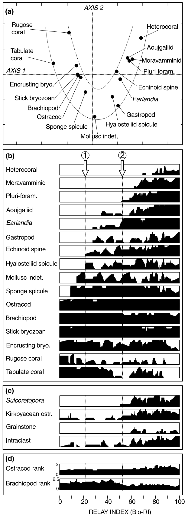
Fig. 13. Results of correspondence analysis (presence/absence mode) of skeletal grain-types. (a) Plot of the plane containing axes 1 and 2 showing the point cloud of the 16 grain-types. Envelope curves outline the arch effect. (b) Relay derived from the analysis. The Relay Index (labelled 'Bio-RI' to distinguish it from the Mud-RI used earlier) was obtained from the intercept of each sample on axis 1 (for details of the technique, see Hennebert & Lees, 1991, p. 630; Lees & Miller, 1995, fig. 22). The presence/absence of each sample was then graphed, and the moving average of five samples was taken. Vertical scale = 0 (absence) to 1 (presence). The height of each curve thus provides an indication of the frequency of presence. (c) Other parameters not included in the analysis but plotted for comparison. Vertical scale = 0 (absence) to 1 (presence). (d) Two of the grain-types included in the analysis but plotted here in terms of rank. Compare with presence/absence plots in (b). Although both organisms are virtually ubiquitous, and rank was not taken into account in the analysis, the brachiopods are shown to rank more highly at the 'deeper' (low Bio-RI) end of the relay, whereas ostracods tend to be more important at the 'shallow' (high Bio-RI) end. The vertical lines arrowed (1) and (2) indicate the levels in the relay at which the hyalosteliid spicules and plurilocular foraminifera appear, key grain-types for Waulsortian Phases B and C respectively.
