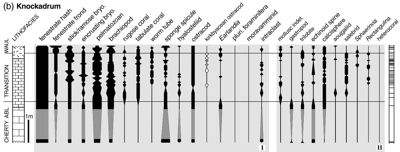
Fig. 10. Distribution of grain-types: (a) Mantlehill ( n = 43 ); (b) Knockadrum ( n = 35 ); (c) Hill 707 ( n = 20 ); (d) Dunmore ( n = 63 ). Each grain-type was recorded on a four-point ranking scale based on visual estimates of the volumetric importance of grains independent of the proportions of matrix or cement. Pale ornament in the logs of the Cherty ABL at Mantlehill and Knockadrum indicates an interval not sampled. The sampling column indicates the mid-point of each thin-section. The grain-types plotted in box I are those that exceed the lowest rank in at least one locality. The kirkbyacean ostracods are an exception, but they are placed here for comparison with the main ostracod trend. The width of the bar corresponds to the ranking – the wider the bar, the higher the rank; a thin vertical line indicates absence. In box II, the grain-types are always minor, never exceeding the lowest rank at any locality. The lithofacies indicated by ornaments in the left-hand column are those determined in the field, whereas the horizontal lines across the figure show the limits of the transition and Waulsortian facies based on the arrival of precursor muds and polymuds. Conventions: ‘fenestrate bryozoan’, small hash is logged separately from larger fragments of frond (five zooecia or more); ‘pelmatozoan’, mainly crinoid; ‘sponge spicule’, this column excludes the large ‘hyalosteliid’ spicules, which are logged separately; ‘moravaminid’, groups all the tubular microfossils, septate or not, of the order Moravaminida (Termier et al. , 1975, 1977) and includes some, such as the palaeoberesellids, which have been regarded as dasycladacean algae (Skompski, 1987); ‘pluri-foraminifera’, plurilocular foraminifera of all types; ‘mollusc indet.’, includes all mollusc fragments not identifiable as gastropods, which are logged separately.
