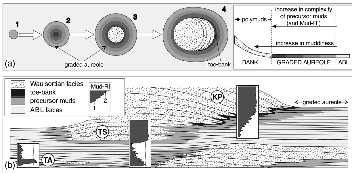
Fig. 9. Model showing the envisaged relationships of precursor muds to Waulsortian banks. (a) Schematic plan view of the postulated developmental sequence starting from (1) an initial patch of simple precursor muds. (2) As the patch spread, the muds gradually increased in complexity centripetally. (3) The Waulsortian polymuds then began to form in the centre. (4) The precursor muds persisted as a graded aureole around the bank, which is shown prograding. (b) Vertical section showing the relationships between the precursor muds and various bank growth-forms. The degree of development of the precursor mud sequence is indicated by the Mud-RI curves, where (1) marks the value at which precursor muds start and (2) the beginning of polymud formation. TA = an aborted tabular-form bank (such as that below the main Waulsortian bank at Dunmore): the Mud-RI shows a rapid increase through a thin transition facies because it is a true precursor and there is no progradation. TS = a tabular-form bank with static margin (e.g. Knockadrum): the Mud-RI in the thin transition facies unit immediately below the bank shows a rapid increase for the same reason as TA; the thicker unit of transition facies in the lower part of the log with Mud-RI decreasing upwards is related to another bank that is migrating away from the site. KP = a prograding knoll-form bank (e.g. Hill 707 and, probably, Mantlehill): because of bank progradation, the Mud-RI increases gradually through a thick transition facies (including a toe-bank facies).
