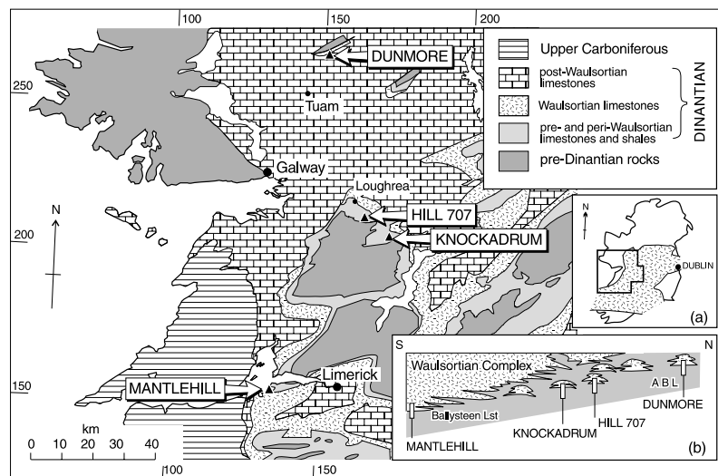
Fig. 1. The regional and stratigraphic context of the four studied localities. Faults omitted for clarity. Numbers shown in the margin refer to the Irish National Grid. The area shaded on the inset (a) shows the original extent of the Waulsortian Complex when fully developed in the late Tournaisian. Inset (b) is a highly schematic cross-section (with gross vertical exaggeration) indicating the broadly transgressive nature of the Waulsortian Complex and the tendency for isolated bank masses to occur under and on the original landward (here the northern) side of the continuous bank development. In inset (b), ABL = Argillaceous Bioclastic Limestone. In the text, the Ballysteen Limestone and the Argillaceous Bioclastic Limestone are grouped as the ABL facies.
