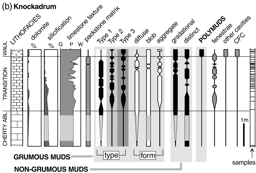
Fig. 3. Lithological and textural characters with particular emphasis on the carbonate muds and associated features. (a) Mantlehill ( n = 43 ). (b) Knockadrum ( n = 35 ). (c) Hill 707 ( n = 20 ). (d) Dunmore ( n = 63 ). As the general dip in the Dunmore section is low ( 5\text{--}10^\circ measured in the ABL facies), no correction has been made for true thickness; the base of the Waulsortian bank in the drill-core lies at a depth of 155.2 m. Horizontal lines mark the boundaries between facies as determined in the field. The sampling column indicates the mid-point of each thin-section. Limestone texture is recorded on the Dunham scale (G, P and W = grainstone, packstone and wackestone). Textures intermediate between standard types indicate the presence of more than one category in the thin-section and their relative proportions. All mud characters and associated features (see text for descriptions) are recorded as presence/absence. CFC = crypto-fibrous calcite. 'Other cavities' includes shelter and stromatactoid cavities (spar-filled) generally much larger than the sparry fenestrae, which rarely exceed a few millimetres.
