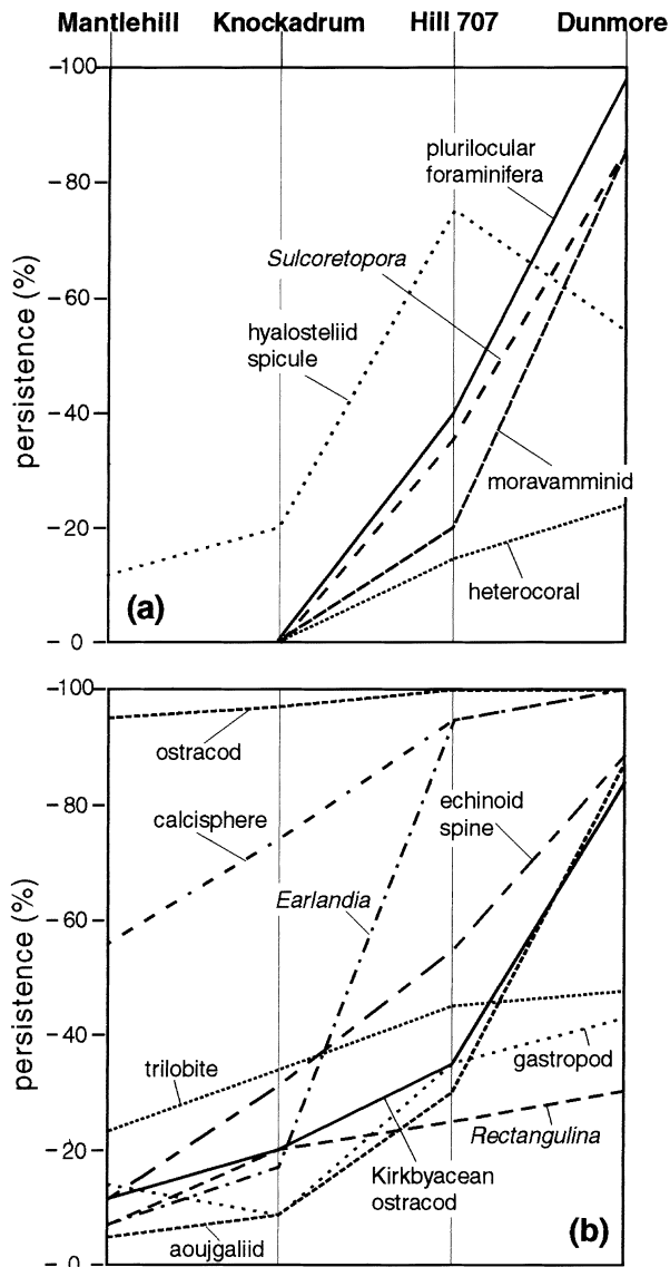
Fig. 11. Skeletal grain-types showing the regional trend of increasing persistence towards the north. (a) Four grain-types occurring only in the two northern sections; the hyalosteliid spicules are added to show their behaviour relative to the foraminifera and moravaminids (all three being key grain-types in Waulsortian Phases B and C). (b) Grain-types present in all localities but displaying increasing persistence northwards.
