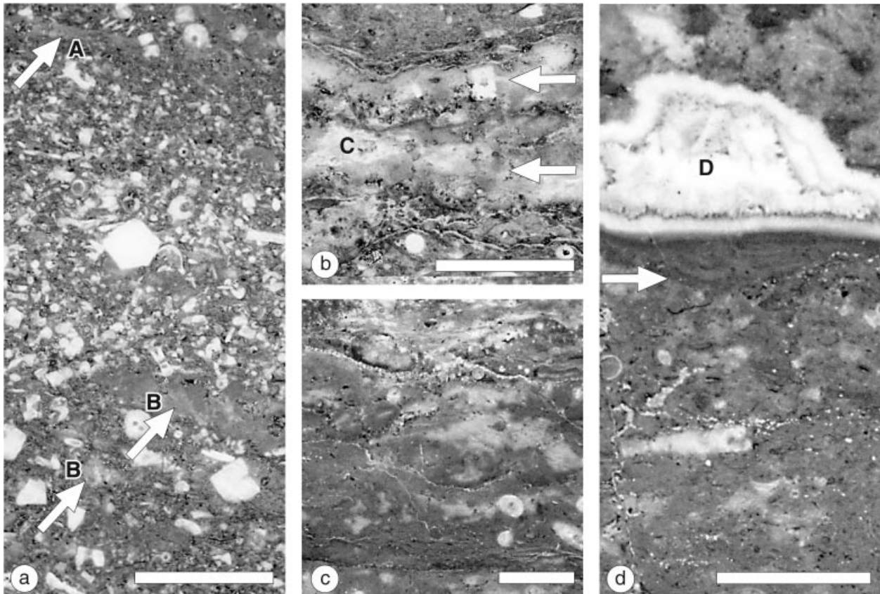
Fig. 5. Polished surfaces illustrating macroscopic features of precursor muds at various stages in the developmental sequence (indicated below by the Mud-RI for the corresponding thin-section). For details of the fabrics present at the various Mud-RI values, see Fig. 4. Note the general increase in muddiness from (a) to (d). Scale bar = 1 cm in all cases. (a) Thin, discontinuous layer (arrowed A) and a slightly disrupted mass of blobs and small aggregates (lower third of photograph; two examples arrowed B) of precursor muds lying in a crinoidal packstone–grainstone; 90 cm below the base of bank, Dunmore. Mud-RI = 60. (b) Two irregular layers of precursor muds (arrowed), locally bounded by stylolites, in a packstone–wackestone setting; Knockadrum. Mud-RI = 63. The pale blotches (e.g. at C), often pinkish in colour, are a common feature of these muds and can be seen, less well developed, in the other samples; their cause is unknown. (c) Bed formed from an aggregate of precursor mud blobs, mainly wackestone; 30 cm below the base of bank, Hill 707. Mud-RI = 80. (d) Basal contact (arrowed) of the bank at Knockadrum showing polymuds overlying a continuous mass of precursor muds (lower half of photograph). The precursor muds are mainly non-grumous. Textures are wackestone throughout. Mud-RI = 90–100. Note that the form of the large cavity (D) in the basal polymuds is unusual, as its walls were locally modified by dissolution before the introduction of the geopetal sediment and the cement fill (CFC followed by blocky calcite).
