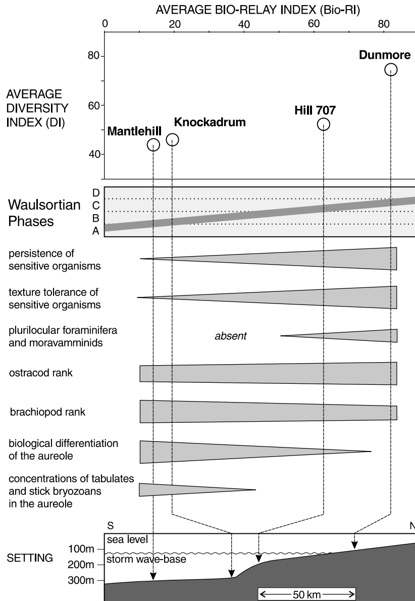
Fig. 16. Summary and interpretation of main regional trends shown by the distributions of the organisms recorded during petrographic analysis. 'Sensitive organisms' are those that vary in abundance systematically along the bathymetric gradient (for persistence, see Fig. 11; for texture tolerance, see Fig. 15). 'Rank' refers to the systematic change in relative importance of the organisms concerned. The 'aureole' is the area around growing banks that was characterized by the presence of 'precursor' muds. The bathymetric model presents the postulated situation for each locality at the time when the Waulsortian facies was initiated there. However, the stratigraphic differences between localities mean that this model cannot be regarded as static. At least some of the northward shallowing expressed here may have been the result of falling sea level if the late Tournaisian regression recorded elsewhere in Europe also affected western Ireland.
