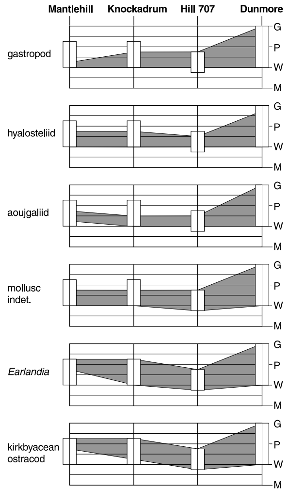
Fig. 15. Textural range occupied by some organisms showing increased textural restriction from north (Dunmore) to south (Mantlehill). The broad white bars at each locality indicate the total textural range present there. G, P, W and M = grainstone, packstone, wackestone and mudstone. For details of organisms, see description in Fig. 10.
