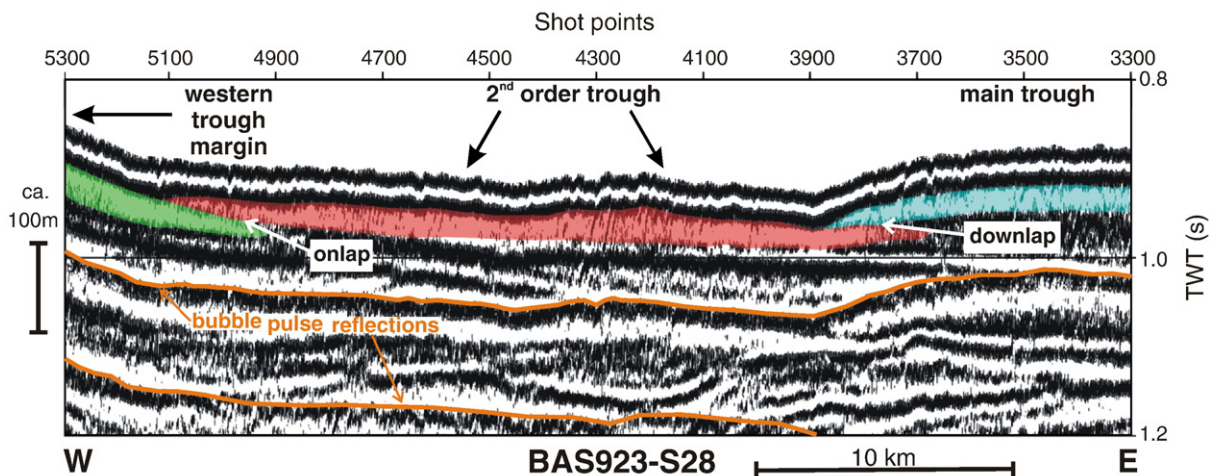
Fig. 13. Single-channel seismic profile crossing the western flank of Belgica Trough on the outer shelf, including the small second-order trough incised into the main trough (for location of profile see Fig. 1). Downlap and onlap relationships between near-seabed sedimentary units indicate their diachronous deposition. Bubble pulse reflections are also indicated. (The seismic source was a single 4.9 l airgun towed at a water depth of 4 m. The interaction of the initial pulse from the airgun with the “ghost” reflection from the sea surface gives a characteristic peak-trough-peak signature, which is reflected from the seafloor and masks other reflections for ca. 35 ms. The data is also affected by bubble pulse reverberations with a period of ca. 135 ms, which have been partially suppressed by predictive convolution.)
