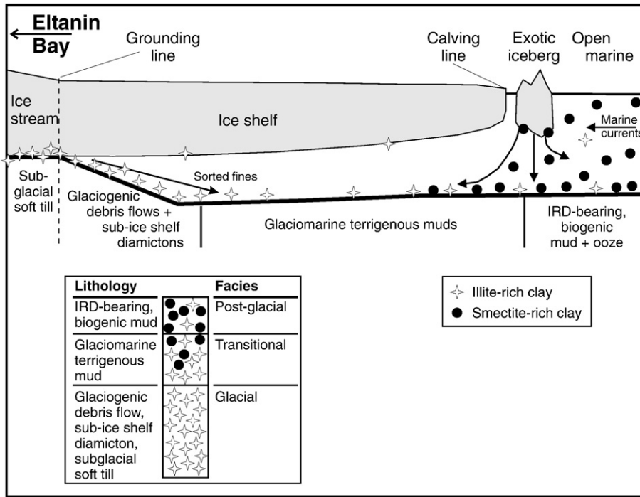
Fig. 10. Conceptual model for the deposition of the facies types and their associated clay mineral assemblages on the southern Bellingshausen Sea shelf since the last glacial maximum (facies model modified from Domack et al., 1999). This model applies only to core sites from Group B, which were affected by ice draining through Eltanin Bay. In a model for core sites from Group C, which were affected by ice draining through Ronne Entrance, smectite- and illite-rich clay would have to be exchanged.
