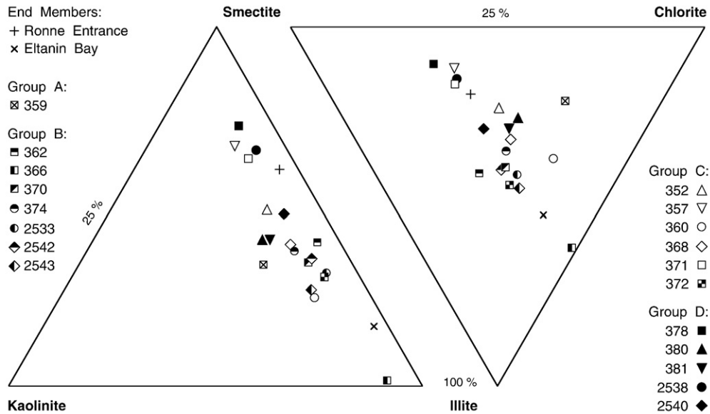
Fig. 7. Ternary diagrams showing the average clay mineral composition of the sediments in the middle lithological unit of the studied cores. End members and groups as in Fig. 5.
