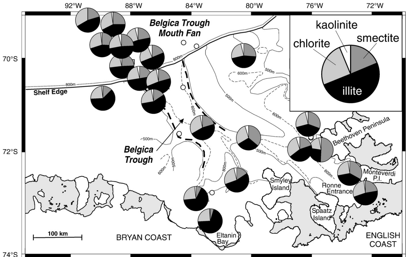
Fig. 2. Clay mineral composition of seabed surface sediments in the study area (for sample locations see Supplementary Table).
