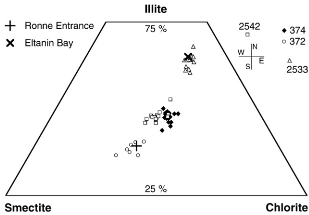
Fig. 12. Ternary diagram showing the clay mineral composition of all samples taken from the glacial diamictons in cores PS2533-2 and GC374 collected from the middle and outer shelf in Belgica Trough and cores GC372 and PS2542-2 recovered from the second-order trough that is incised into Belgica Trough on the outer shelf (site numbers in the key in the upper right are orientated according to their approximate relative location, see Fig. 1). End members and groups as in Fig. 5.
