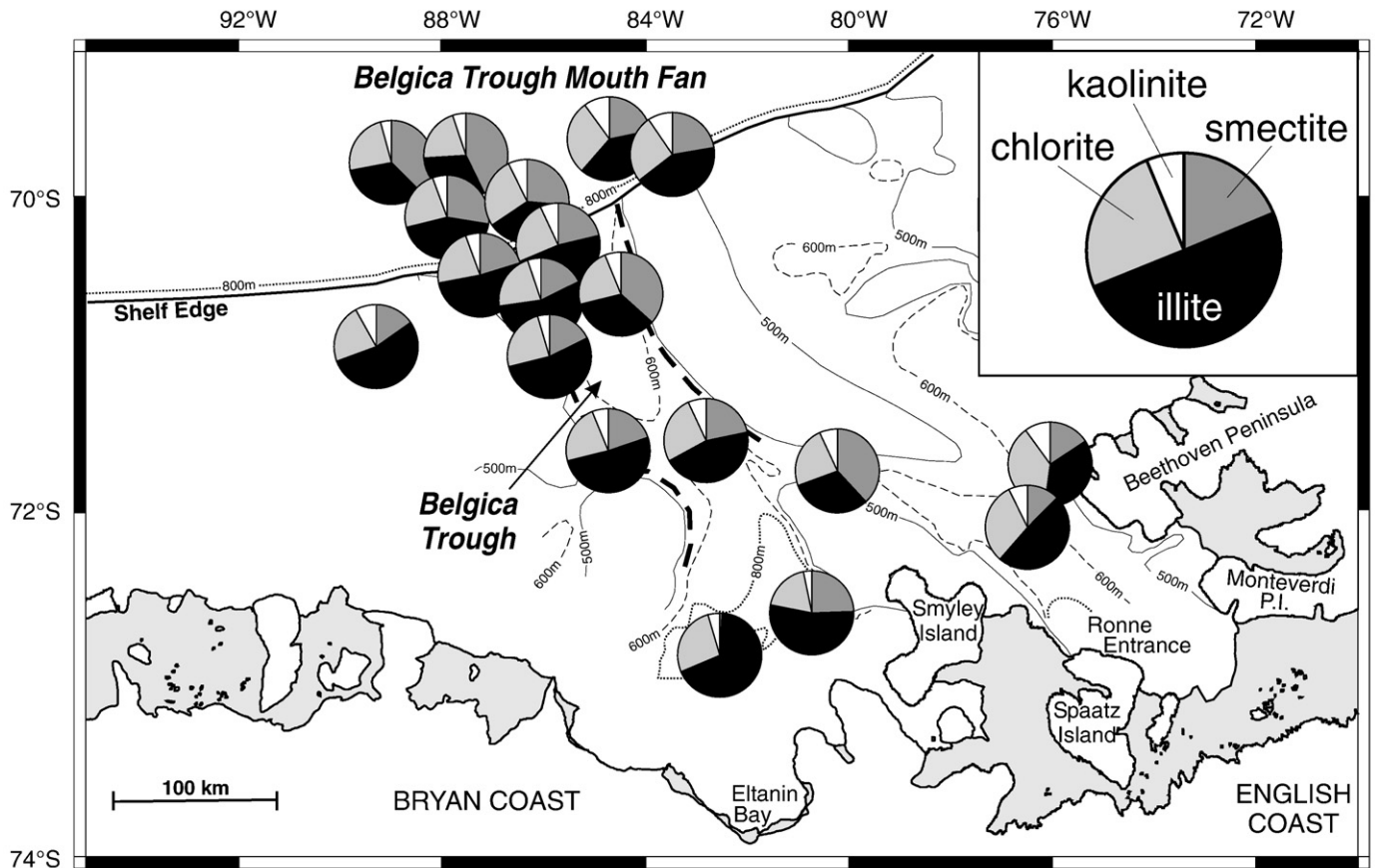
Fig. 6. Average clay mineral composition of sediments in the middle lithological unit of the studied cores.
