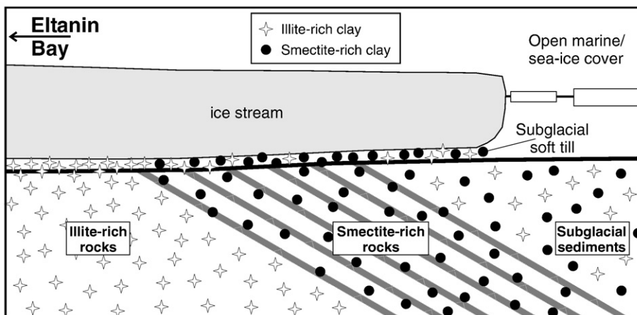
Fig. 11. Conceptual model for the subglacial erosion of old, smectite-bearing sediments on the southern Bellingshausen Sea shelf and the deposition of subglacial sediments during the last glacial period. This model explains, for example, the differences in clay mineral composition of the glacial diamictons recovered at sites PS2533-2 and GC372 (see Fig. 12).
