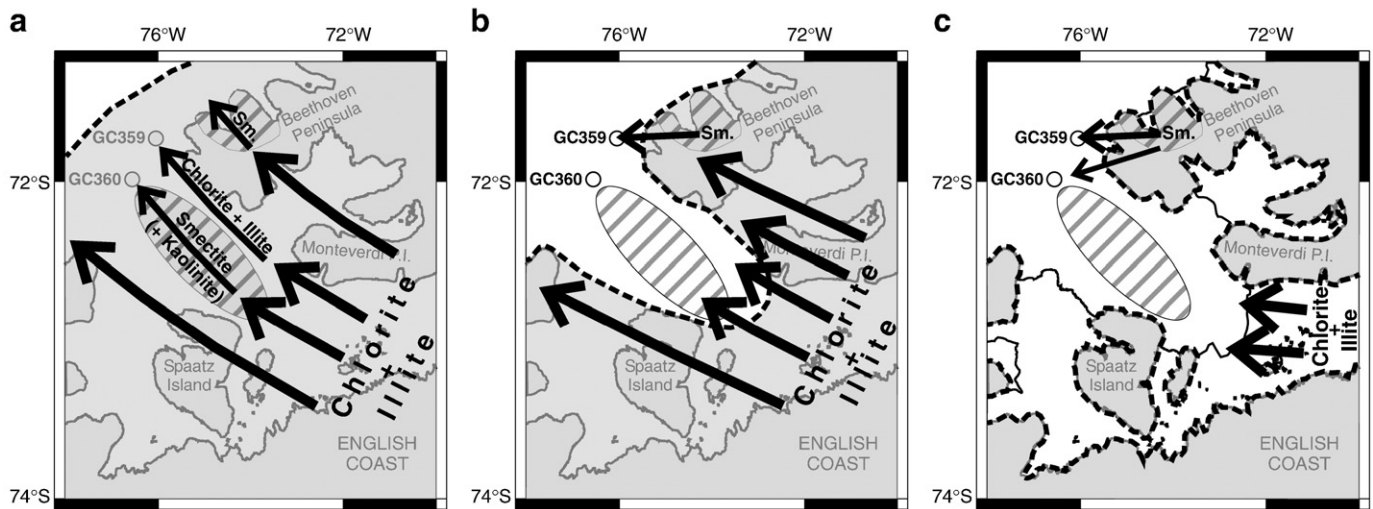
Fig. 15. Inferred ice-flow directions (arrows) and clay mineralogical provenance of subglacial debris supplied to sites GC359 and GC360 during the last glacial period (a), the deglaciation (b) and the present interglacial period (c). The grey shaded area indicates the spatial distribution of grounded ice (schematically), the bold broken line marks the position of the grounding line (schematically). The hatched area on Beethoven Peninsula highlights the occurrence of Cenozoic volcanic rocks as a smectite source. The hatched area in Ronne Entrance indicates the inferred position of smectite-rich sedimentary strata in a deep shelf basin.
