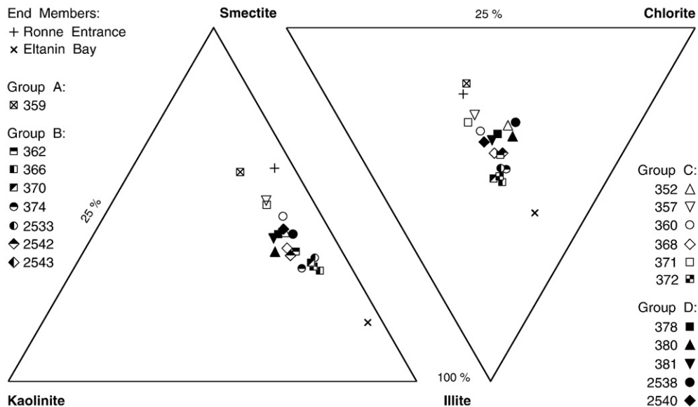
Fig. 9. Ternary diagrams showing the average clay mineral composition of the sediments in the upper lithological unit of the studied cores. End members and groups as in Fig. 5.
