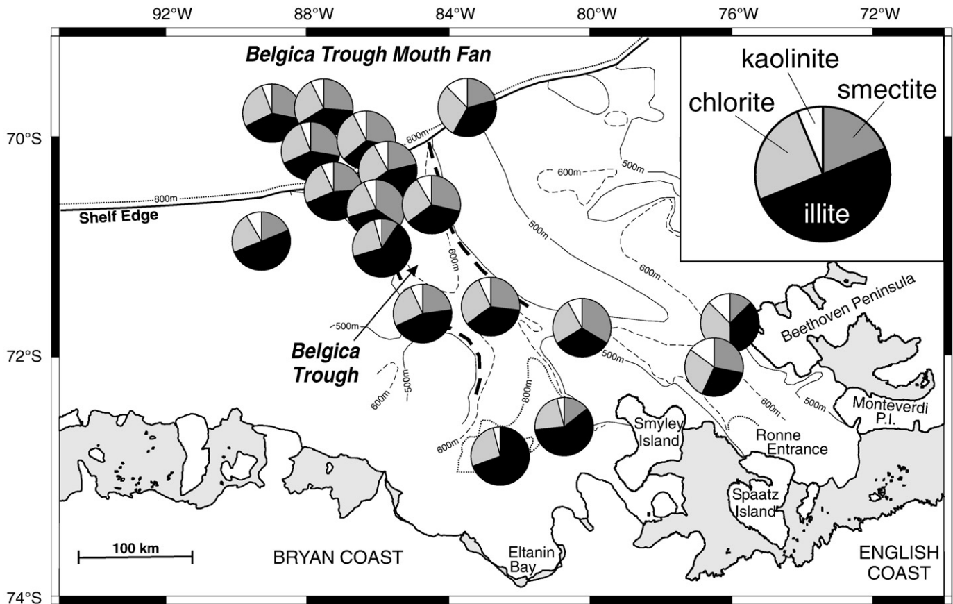
Fig. 4. Average clay mineral composition of sediments in the lower lithological unit of the studied cores.
