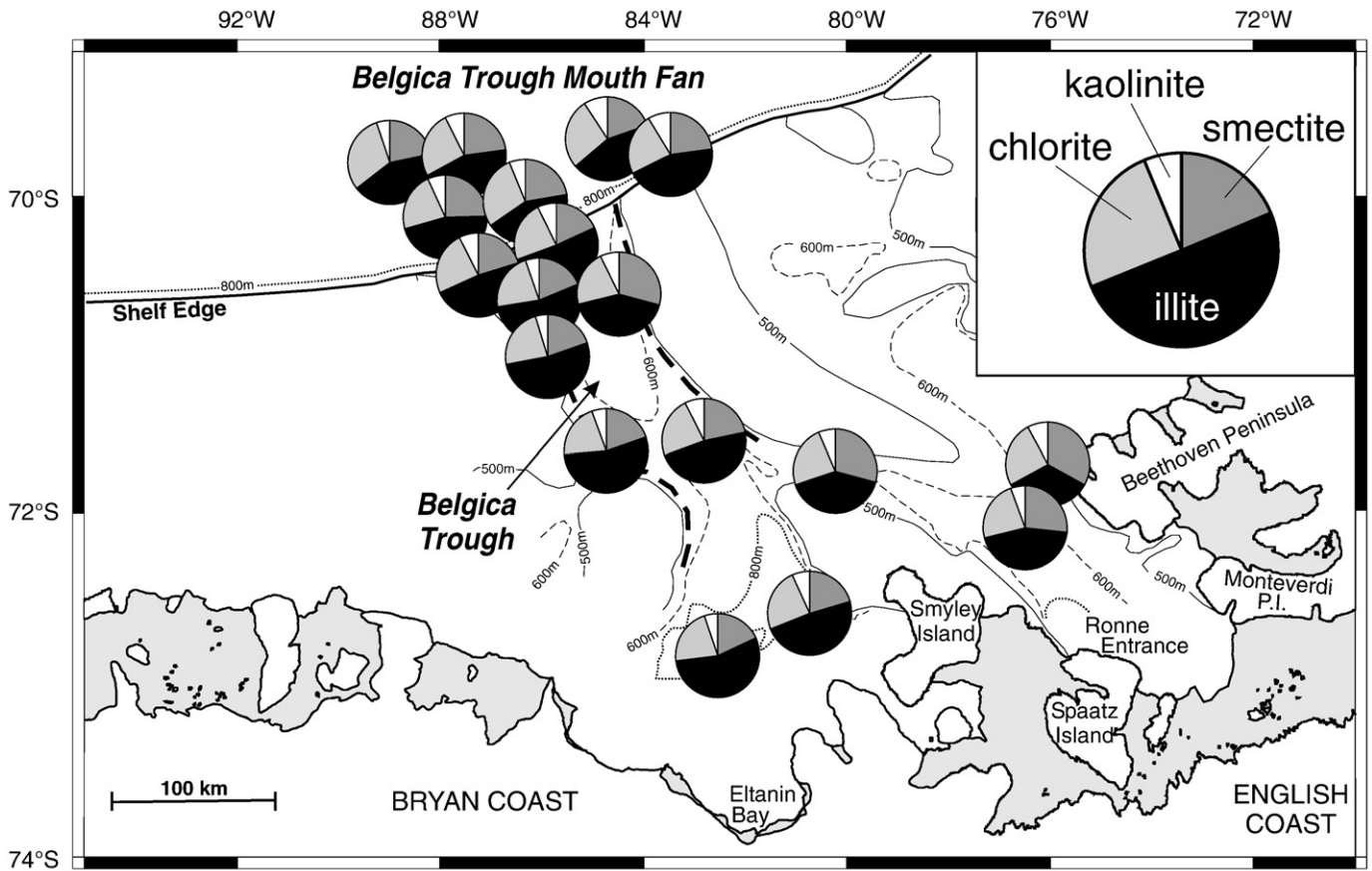
Fig. 8. Average clay mineral composition of sediments in the upper lithological unit of the studied cores.
