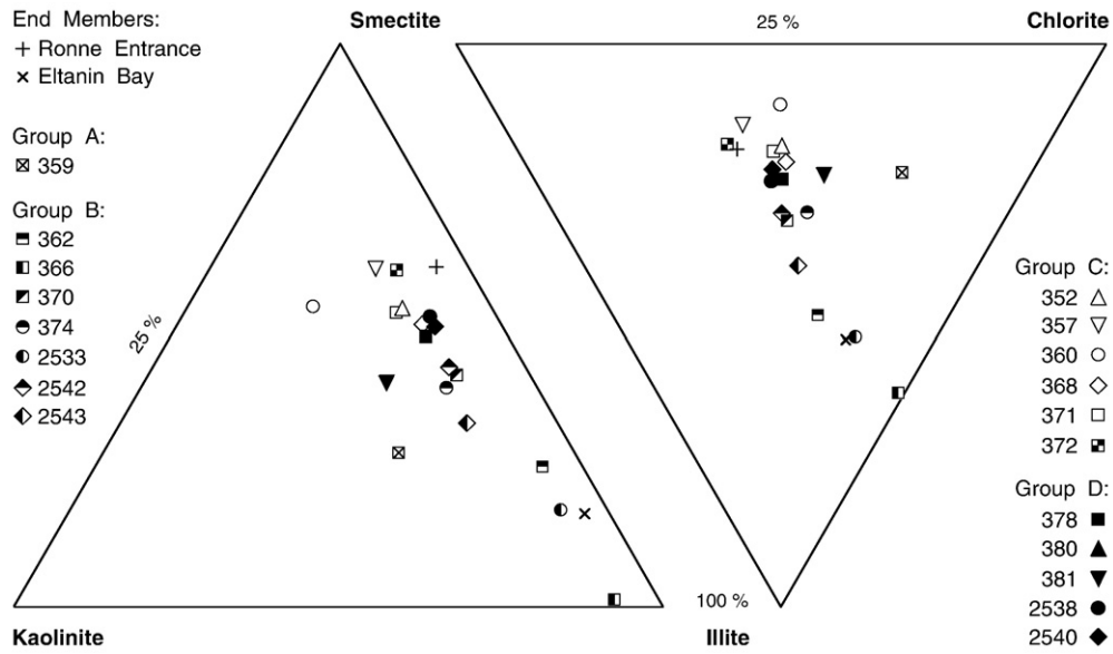
Fig. 5. Ternary diagrams showing the average clay mineral composition of sediments in the lower lithological unit of the studied cores. End members are the average clay mineral composition of surface sediment samples from Ronne Entrance and Eltanin Bay (Fig. 2). Group A comprises site GC359, where grounded ice did not flow into Belgica Trough (cf. Fig. 1), Group B comprises core sites on the shelf west of the Belgica Trough main axis, Group C comprises sites on the shelf east of the trough axis, and Group D comprises sites from the continental slope.
