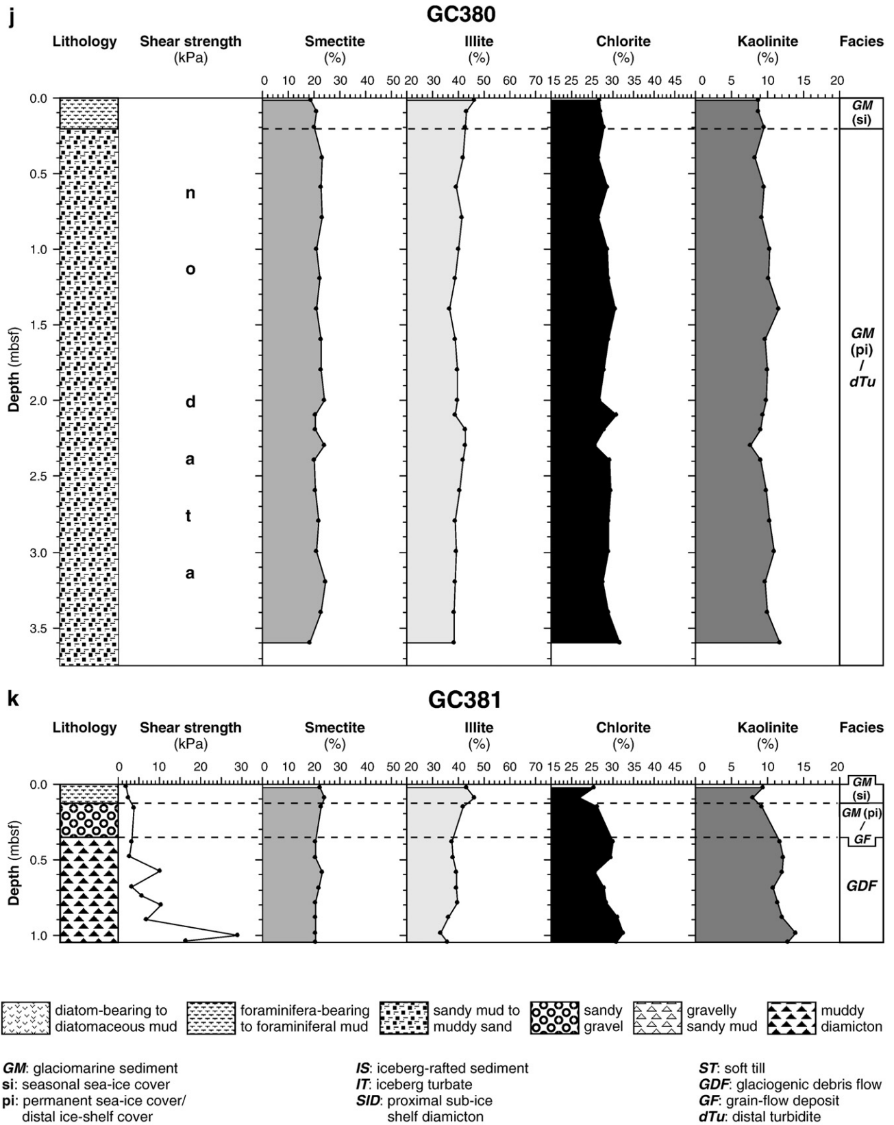
Fig. 3. Lithology, shear strength, clay mineral content and facies types of cores GC366 (Fig. 3a), GC360 (Fig. 3b), GC359 (Fig. 3c), GC357 (Fig. 3d), PS2533-2 (Fig. 3e), GC371 (Fig. 3f), PS2542-2 (Fig. 3g), GC374 (Fig. 3h), PS2538-2 (Fig. 3i), GC380 (Fig. 3j) and GC381 (Fig. 3k) (see also Supplementary Figure).
