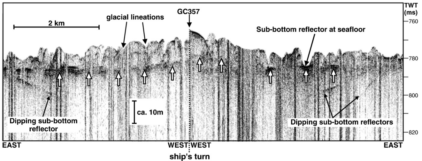
Fig. 14. TOPAS acoustic sub-bottom profile from near site GC357 (for location of profile see Fig. 1). A flat sub-bottom reflector (white arrows) that probably corresponds to a glacial unconformity truncates seaward dipping sub-seafloor reflectors and crops out locally at the modern seafloor. The dipping reflectors are interpreted as eroded, old sedimentary strata. (Vertical noise stripes on the profile are reverberations caused by contact between the ship's hull and sea ice.)
