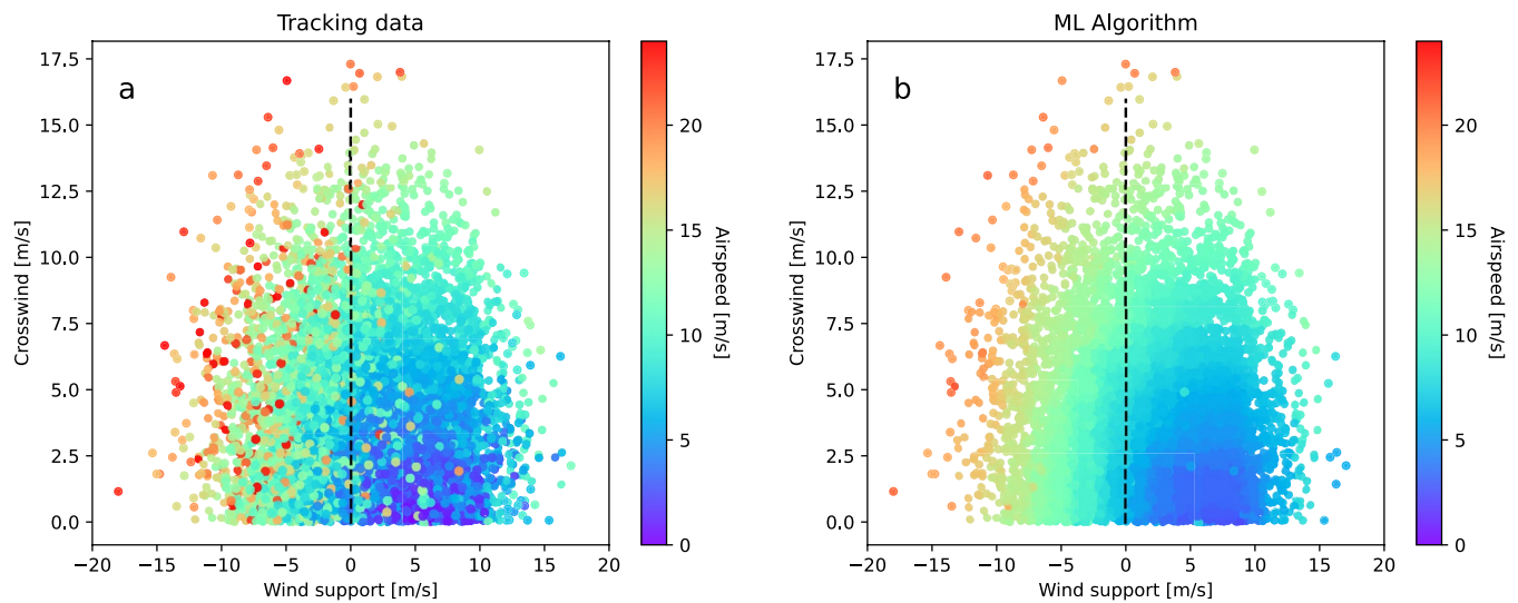
FIGURE 3 | Airspeed (colours) against wind support (x-axis) and crosswind (y-axis) for each arctic tern location (dots). The airspeed of the birds was (a) calculated using trigonometry on the GLS tracking data, with the wind conditions and the bird's groundspeed per location, while in (b) the airspeed was calculated by applying the trained ML algorithm on the wind conditions of the annotated tracking data.
