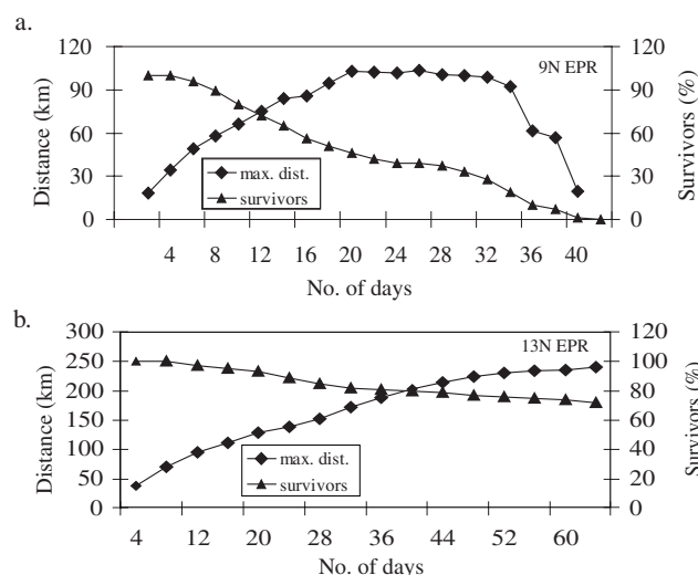
Figure 2. Maximum dispersal distance and survivors (% larvae remaining within 25 km of ridge axis) calculated from dispersal model for larvae of different life spans at two locations on East Pacific Rise: a) at 9°N for larval life span of 2 - 42 days (from Marsh et al., 2001); b) at 13°N for larval life span of 4 - 64 days.
