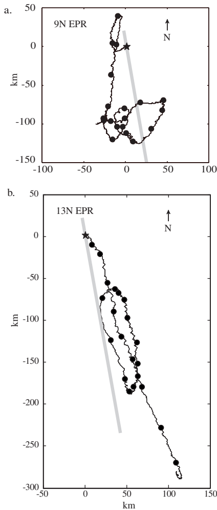
Figure 1. Progressive vector diagrams showing currents at two locations on the East Pacific Rise. Gray lines denote approximate position of ridge axis, additional bathymetric detail can be found in Crane et al. (1988). Diagrams assume lateral homogeneity of flow in order to track the trajectory of a water parcel originating at the location of the current meter (filled star), with filled circles at 7-day intervals: a) currents from 9°50.9'N, 104°17.6'W (9°N), measured at 175 m above bottom, (from Marsh et al. 2001); b) currents from 12°48.9'N, 103°56.6'W (13°N) measured 100 m above bottom (from Chevaldonné et al., 1997).
