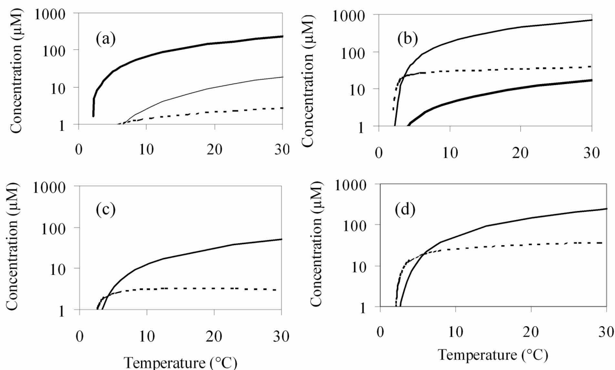
Figure 4. Contribution of \text{H}_2\text{S} (thin line), \text{HS}^- (dotted line) and dissolved or precipitated \text{FeS} forms (bold line) as a function of temperature as predicted from the conservative mixing of the local hydrothermal fluid source and seawater. (a) Alvinellid habitat at Elsa (EPR 13°N), (b) Alvinellid habitat at Genesis (EPR 13°N), (c) Riftia habitat at Tica (EPR 9°N), (d) Riftia habitat at Riftia Field (EPR 9°N).
