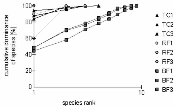
Figure 1. Mean cumulative dominance of nematode species from the three sites (TC = Tica; RF = Riftia Field; BF = Buckfield); relative abundances of species were plotted against species rank (i.e. number of species) for each sample.
