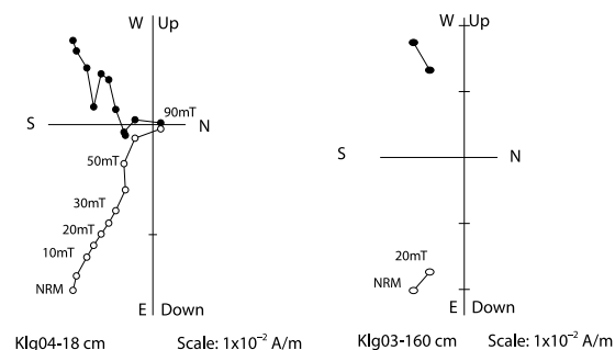
Figure A1. Zijderveld diagram of demagnetization for cores Klg04 at 18 cm in depth and Klg03 at 160 cm in depth. The solid circles represent the projection on the horizontal plane, and the open circles the projection on the vertical plane.
