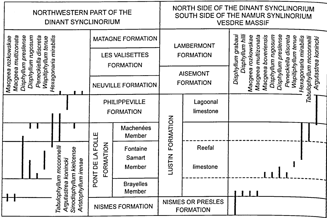
Fig. 9 — Lithostratigraphic units and stratigraphic distribution of the rugose coral species mentioned herein in the Frasnian from the northwestern part of the Dinant Synclinorium as well as from the north side of the same structural area, the south side of the Namur Synclinorium and the Vesdre Massif.
