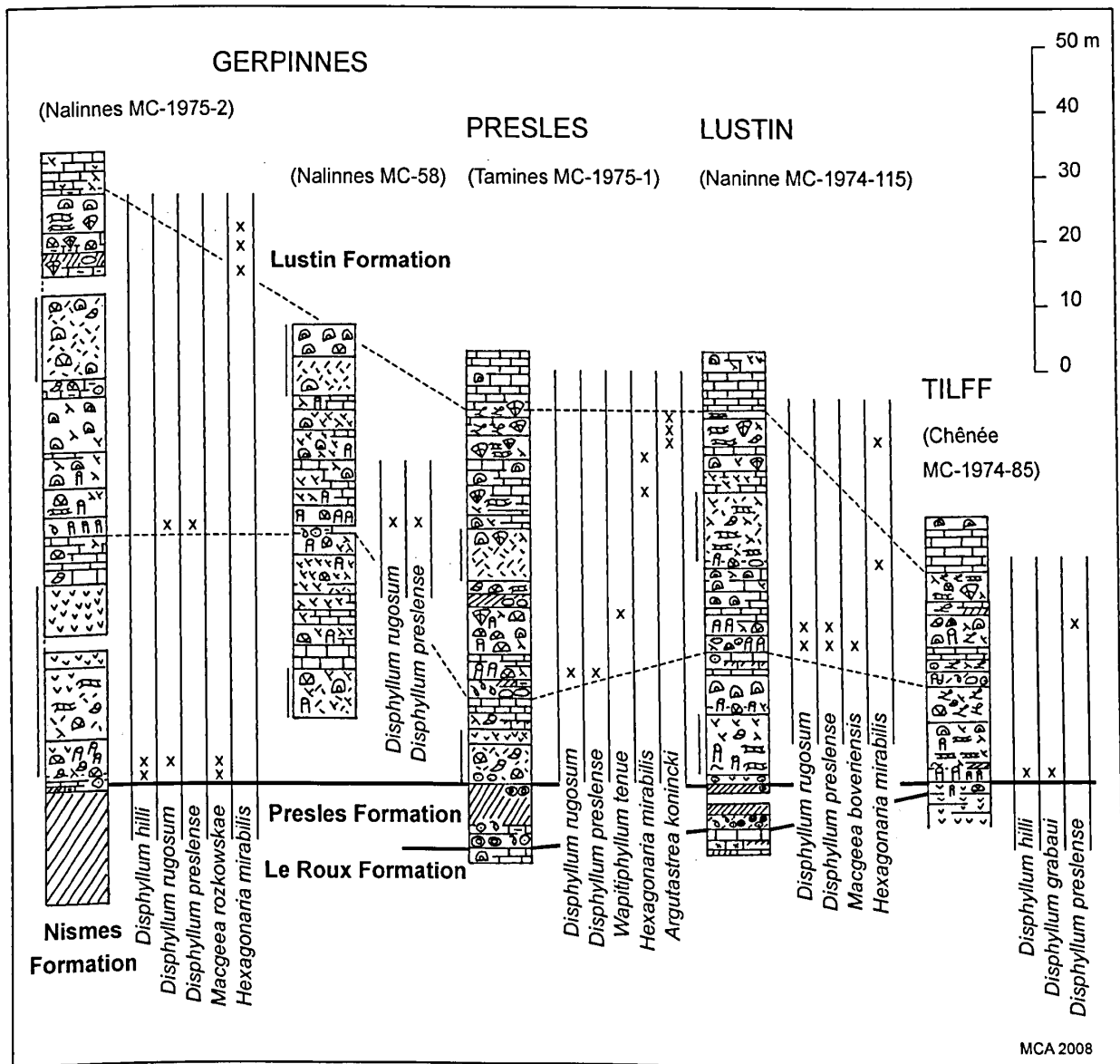
Fig. 5 – Comparative logs from the lower part of the Lustin Formation at Gerpennes, Presles, Lustin and Tilff with the distribution of the rugose corals. (For explanation of conventional signs, see Fig. 3).
