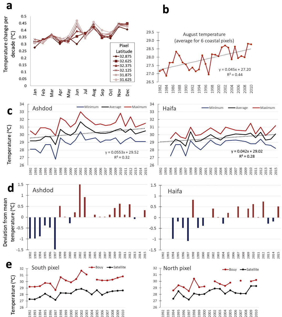
Figure 5. Evidence for sea surface temperature (SST) changes in the southeast Levant coastal waters.
