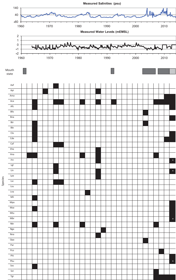
Figure 2. Records of gastropod species collected at Lake St Lucia in relation to changes in salinity, water levels and mouth state during the period 1960-present. Dark gray bar indicates closed mouth, light gray bar indicates intermittent connection with the ocean. No continuous physico-chemical measurements are available for the period prior to 1960. Species codes: Aaf: Afrolittorina africana ; Api: Alaba pinnae ; Ama: Aplexa marmorata ; Aca: Assiminea cf. capensis ; Afc: Assimineidae sp. (“ Assiminea ” aff. capensis ); Bfo: Bulinus forskalii ; Bna: Bulinus natalensis ; Btr: Bulinus tropicus ; Ble: Bursatella leachii ; Cla: Cassidula labrella ; Cde: Cerithidea decollata ; Cdi: Cerithium dialeucum ; Ehe: Ergalatax heptagonalis ; Hna: Haminoea natalensis ; Jsu: Jujubinus suarezensis ; Lgl: Littoraria coccinea glabrata ; Lin: Littoraria intermedia ; Lpa: Littoraria pallescens ; Lsc: Littoraria scabra ; Lsu: Littoraria subvittata ; Lna: Lymnaea natalensis ; Mli: Melampus lividus ; Mpa: Melampus parvulus ; Mse: Melampus semiaratus ; Mtu: Melanoides tuberculata ; Mbr: Murex brevispinus ; Nkr: Nassarius kraussianus ; Nga: Neritina gagates ; Nna: Neritina natalensis ; Opa: Oxyloma patentissima ; Par: Phalium areola ; Pco: Pseudosuccinea columelli ; Phi: Pterotrachea cf. hippocampus ; Pbu: Purpura bufo ; Soc: Siphonaria oculus ; Sst: Stylocheilus striatus ; Tgr: Tarebia granifera .
