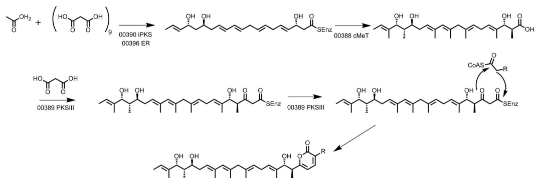
Figure 6. Proposed scheme for lagunapyrones A-D biosynthesis.
