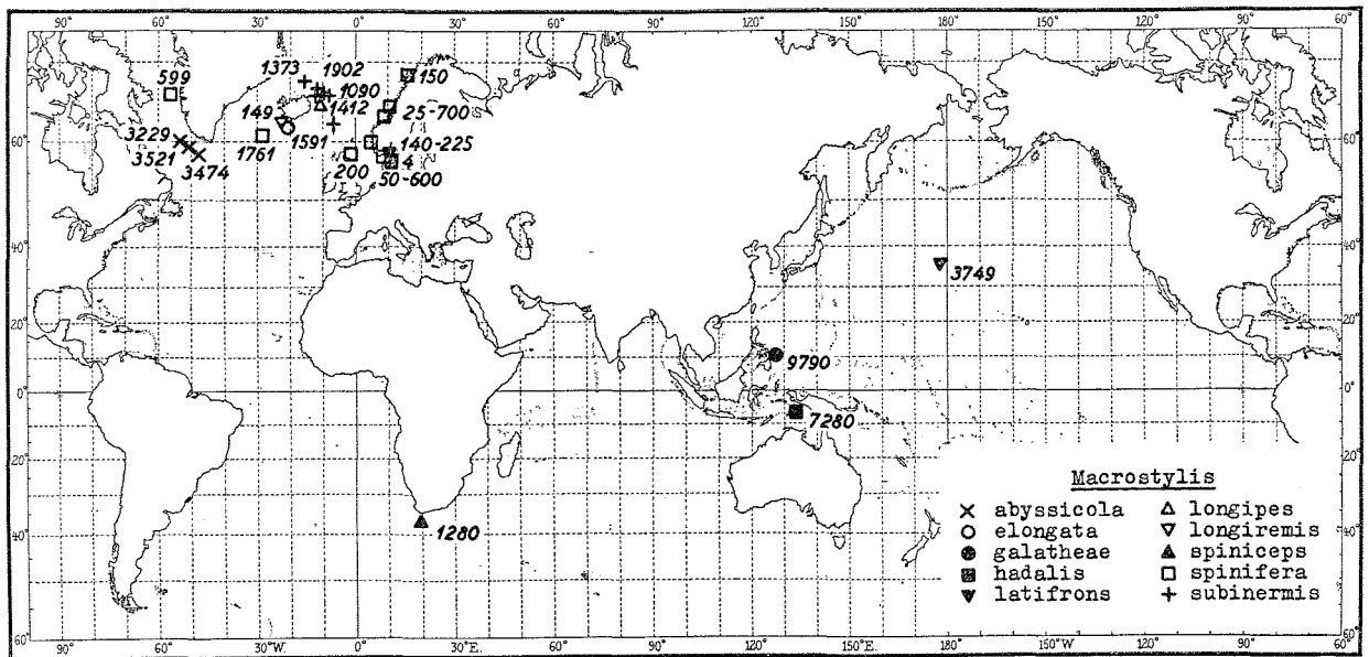
Fig. 55. Distribution of the deep-sea genus Macrostylis . Depths in metres.
