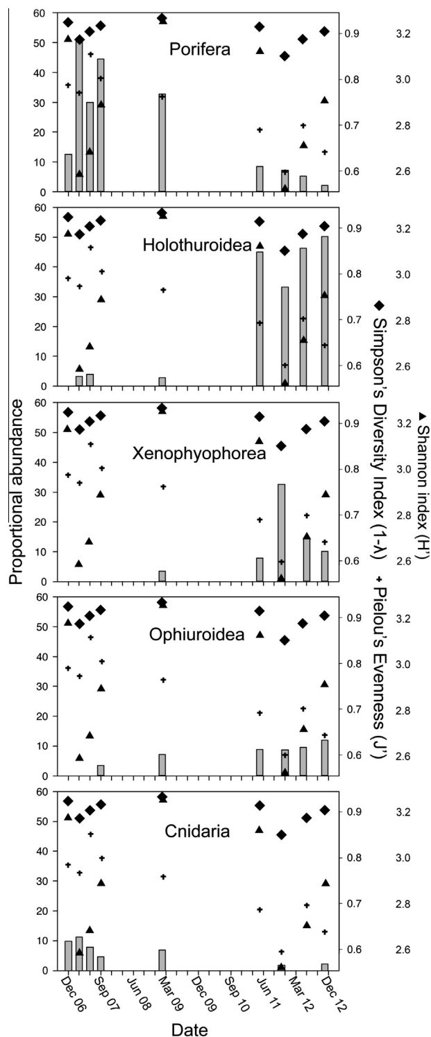
Fig. 3. Relative proportion (as a percent) of higher-taxa groups having the most effect on community structure, based on ROV surveys between 2006 and 2012 (bars). We show Simpson's Diversity Index (SDI), Pielou's Evenness and the Shannon Index (right axis) for each period. Note that due to the short transect length, species richness for June 2007 is likely underestimated.
