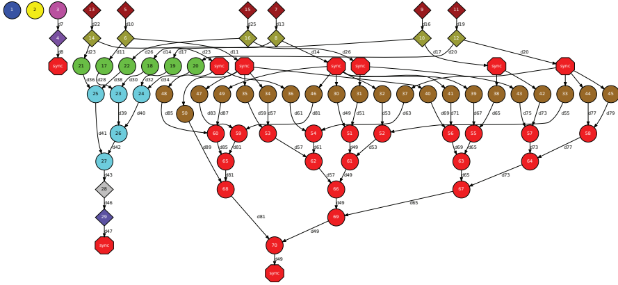
Fig. 8. Graph generated for a Gene Detection execution. The different colors for circles and diamonds represent the different invocations of method CEs and Service CEs. Arrows represent data dependencies and stops represent synchronization points
