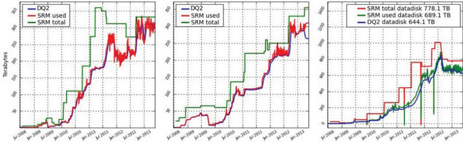
Fig. 5. Occupancy of the T2-ES DATADISK space token: IFAE (left), UAM (center), IFIC (right).
