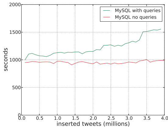
Fig. 4. Time to insert 100000 tweets in MySQL using an empty database and tweets processed with ORM. Linking (green) and duplicating information (red)
