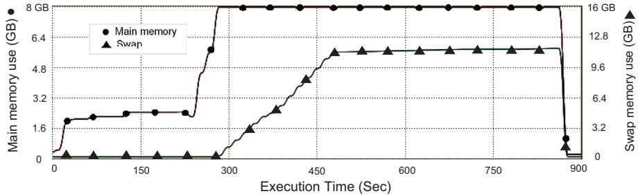
Fig. 2. Memory use for BW_search.
