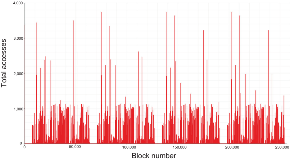
Fig. 3. Total accesses by block (Sequence A).
