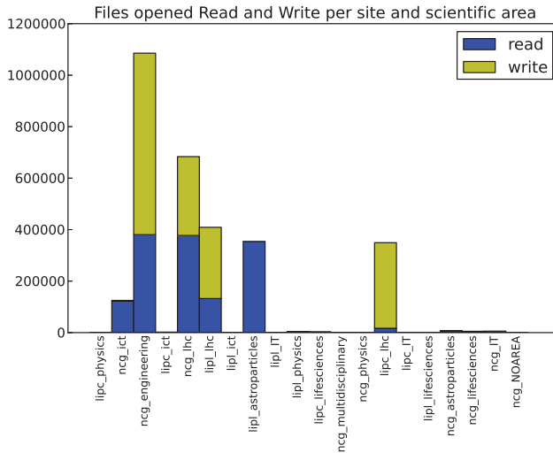
Fig. 2. Number of open operations per scientific domain
