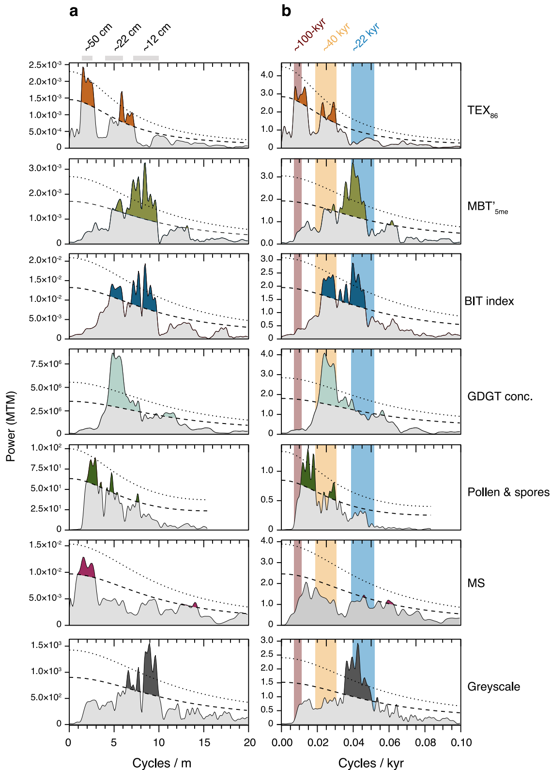
Figure 4. MTM Power spectra in depth (a) and age (b) domains. Dashed and dotted lines indicate 90% and 99% confidence intervals of AR(1), respectively.
