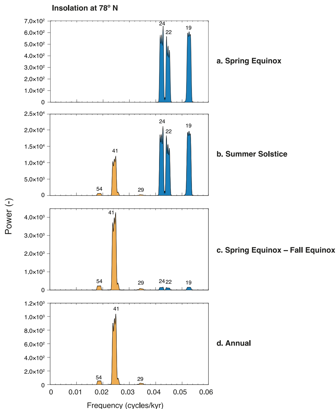
Figure 2. Power spectra of insolation at 78°N, showing obliquity (orange) and precession (blue) frequencies. (a) Insolation spectra during the spring equinox (~21 March). (b) Insolation spectra during the summer solstice (~21 June). (c) Averaged insolation spectra between the spring and fall equinoxes (~21 March–22 September). (d) Mean annual averaged insolation spectra. All spectra are calculated using the Multitaper Method in Acycle (Li et al., 2019) over insolation curves for the past 2 million years (Laskar et al., 2004). Numbers above spectral peaks indicate the corresponding periods in kyr.
