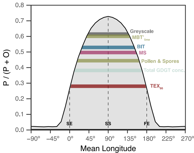
Figure 8. Precession/obliquity index ( P/(P + O) ) of insolation for different periods surrounding the summer solstice. The gray bell curve represents the spectral amplitude of precession divided by the summed amplitudes of precession and obliquity for any given time period surrounding the summer solstice. The colored bands on the bell curve correspond to P/(P + O) values extracted from power spectra of the different proxy records generated in this study. The horizontal axis depicts the mean longitude of Earth's orbit, with the dates of the spring equinox, summer solstice and fall equinox marked by dashed lines. Plot based on MTM spectra of La04 insolation curve (Laskar et al., 2004) at 78°N during the pre-ETM2 interval. SE, spring equinox; SS, summer solstice; FE, fall equinox.
