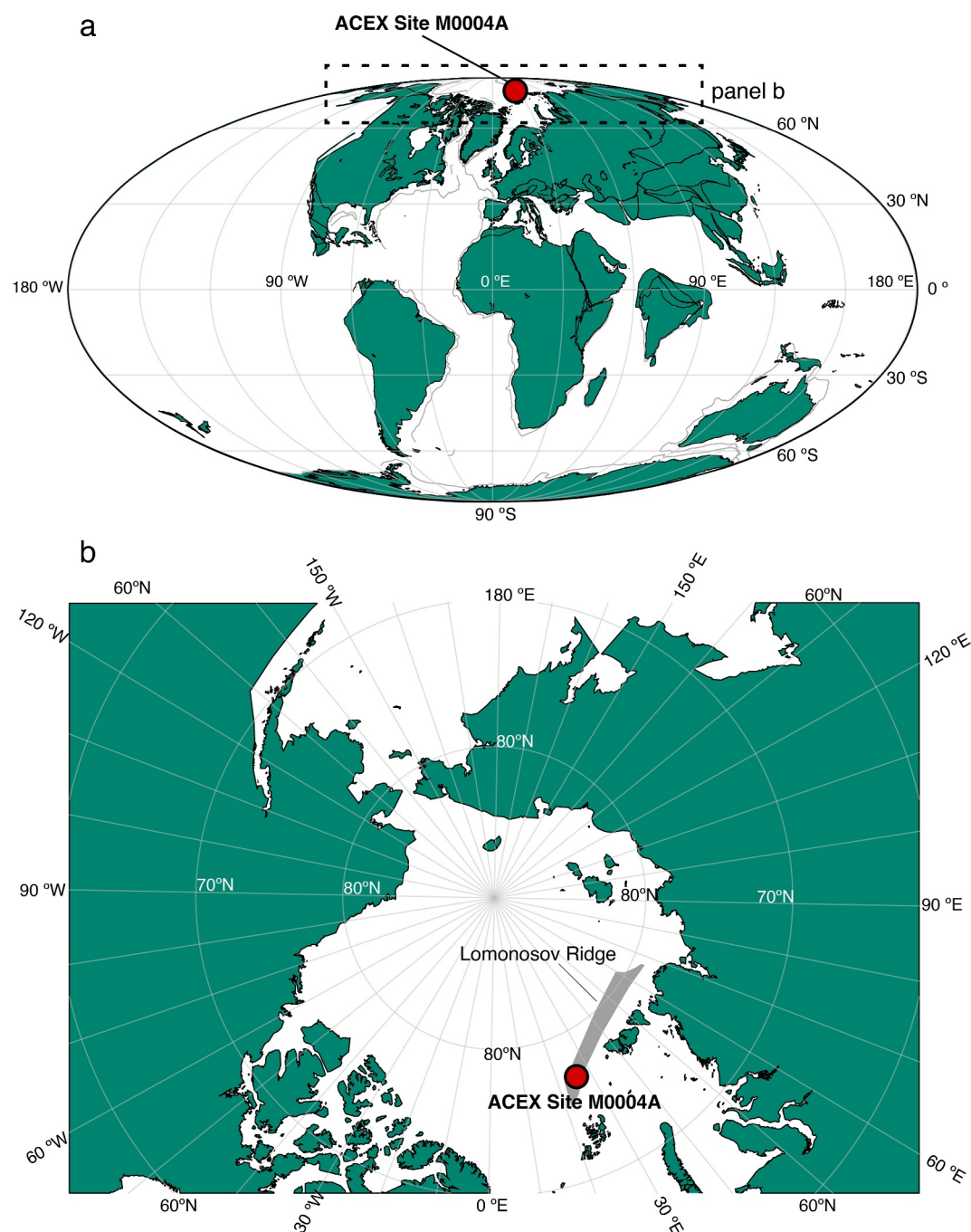
Figure 1. Paleogeographic maps showing the position of ACEX Site M0004A (red dot) in the early Eocene Arctic Ocean. (a) Global map, generated with Gplates (Müller et al., 2018), utilizing the paleomagnetic reference frame of Torsvik et al. (2012) and modern coastlines and plate boundaries by Seton et al. (2012). (b) Regional map adapted from Sluijs et al. (2020), showing the position of the study location on Lomonosov Ridge (gray area).
