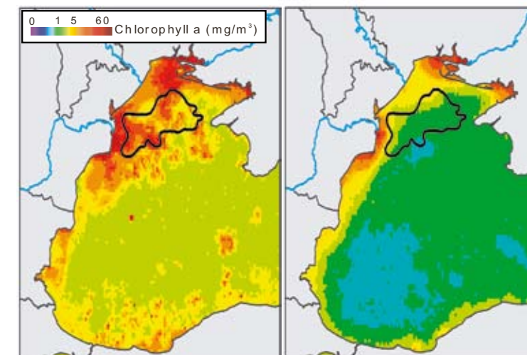
Fig. 9 Maximum extent of Zernov's Phyllophora field prior to eutrophication superimposed over phytoplankton productivity (chlorophyll concentration) on the northwestern shelf of the Black Sea in July 1979 (left) and July 2002 (right).
