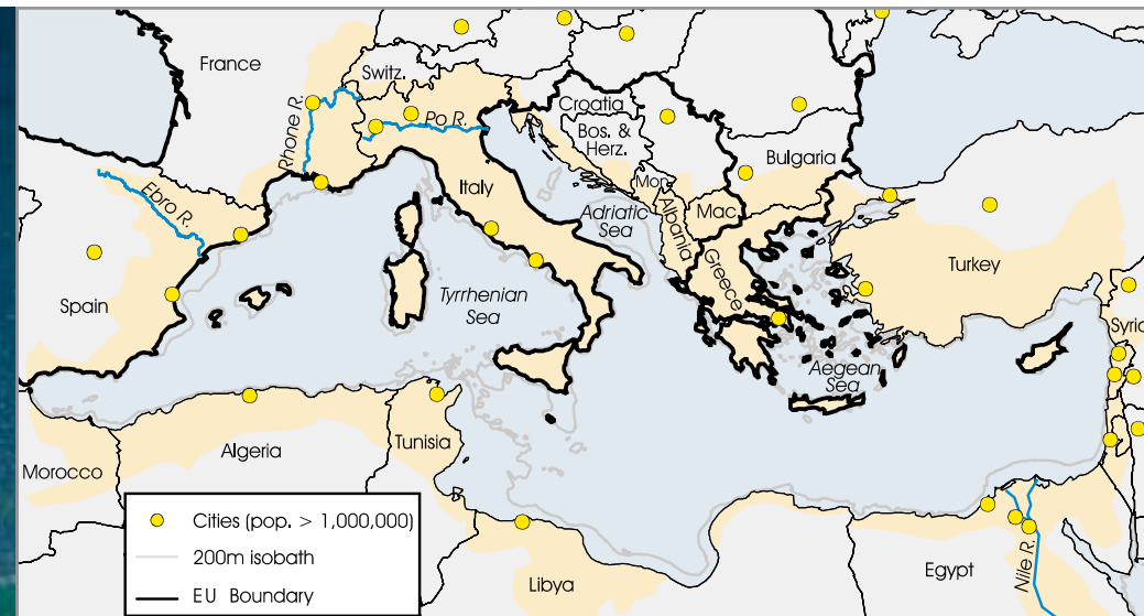
Catchment map of the Mediterranean Sea.
