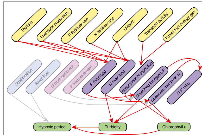
Fig. 13 Conceptual model of the northern Adriatic with the simulation model embedded within it (colours follow those used in the regional model).
