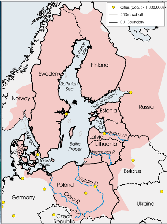
Catchment map of the Baltic Sea.
