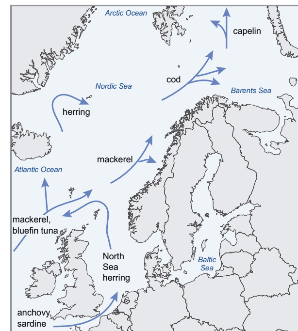
Fig 29 Likely extension of the feeding areas for some fish populations if sea temperature continues to increase (after German Advisory Council on Global Change, 2006).
