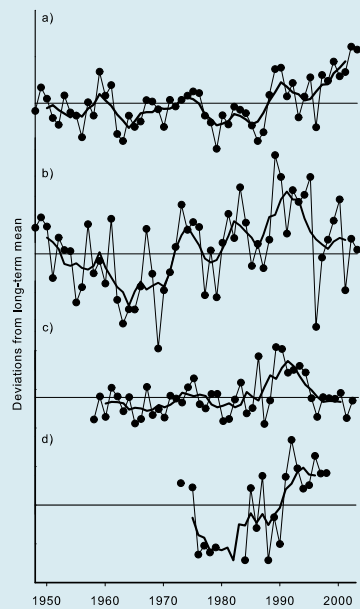
Fig. 19 Changes in (a) North Sea SST, (b) the NAO, (c) Atlantic inflow to the North Sea, and (d) water clarity of coastal waters have occurred in recent years (after McQuatters-Gollop et al. 2007).
