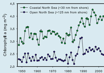
Fig. 17 The 1980s regime shift caused increased chlorophyll in North Sea waters (after McQuatters-Gollop et al. 2007).
