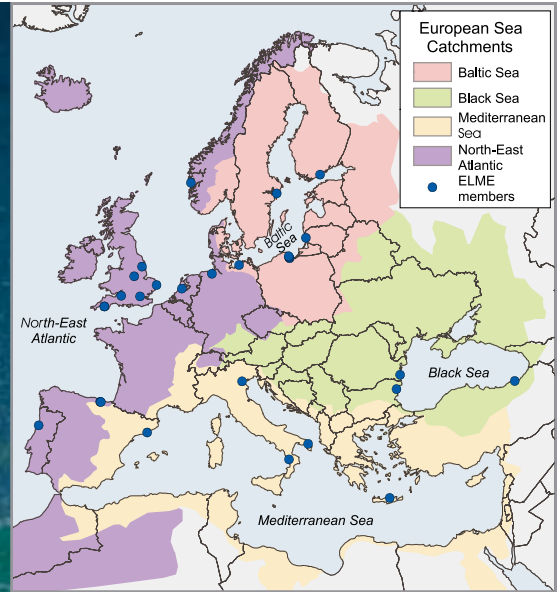
Map of catchment locations for each European regional sea.
