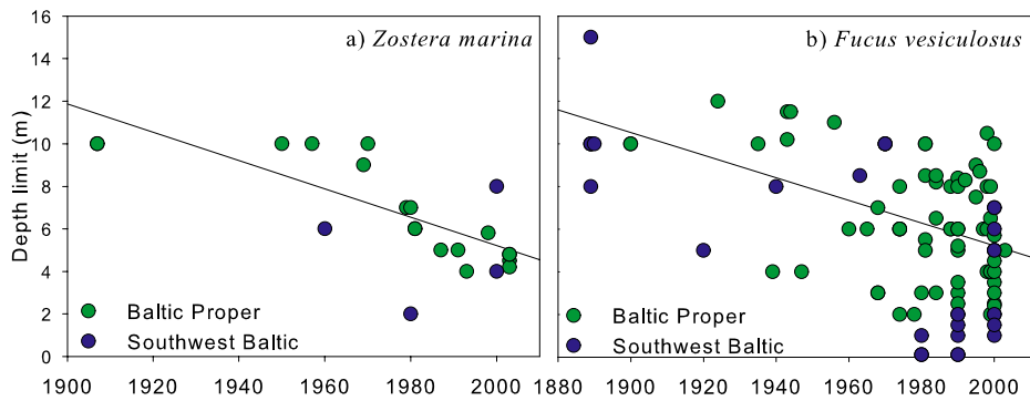
Fig. 6 Long-term trends in depth limit of (a) eelgrass ( Zostera marina ) and (b) bladder wrack ( Fucus vesiculosus ). Note that the trend for Fucus is less clear, possibly suggesting a more complex response to eutrophication such as competition with filamentous algae.
