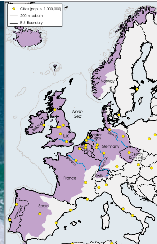
Catchment map of the North-East Atlantic.
