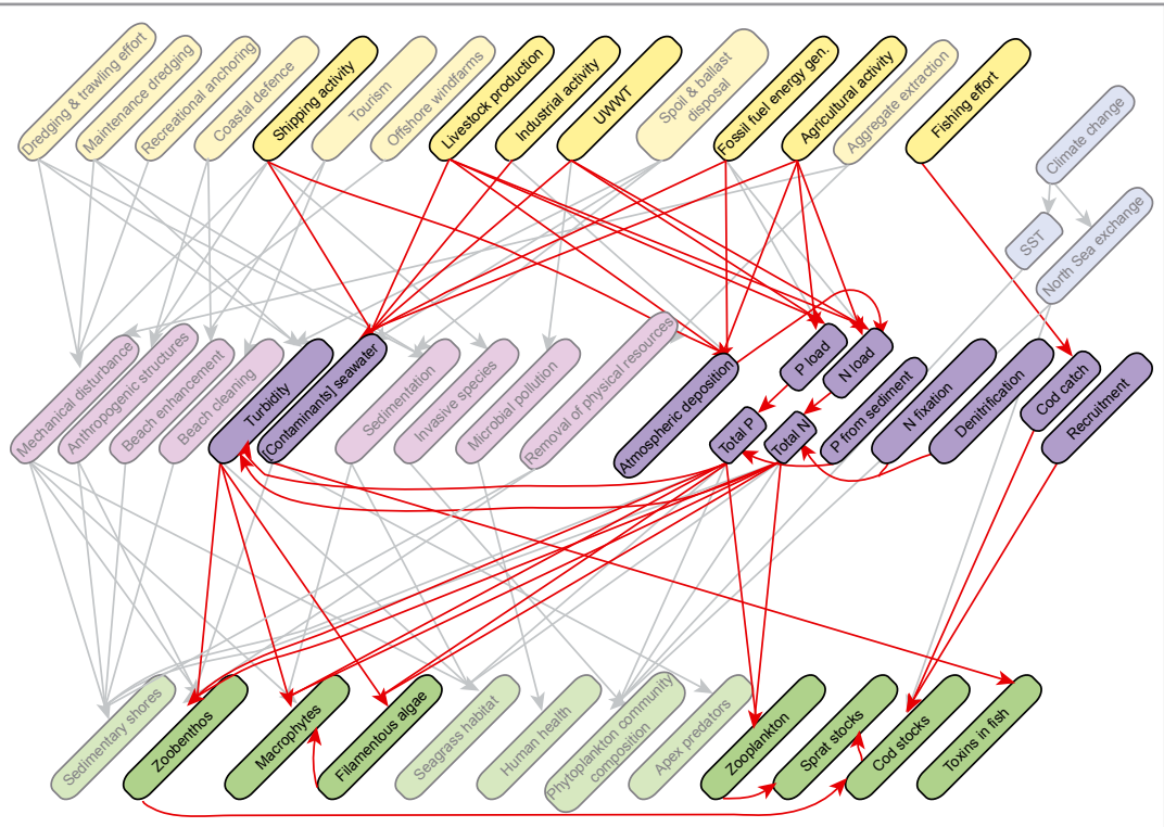
Fig. 3 Baltic Sea conceptual model with the simulation model embedded within it (red arrows show pathways between variables included in the simulation model, while grey arrows indicate where linkages were made conceptually but were not included). Yellow indicates anthropogenic driver variables; blue indicates exogenous climatic driver variables; purple indicates pressures, while green indicates ecological state variables.
