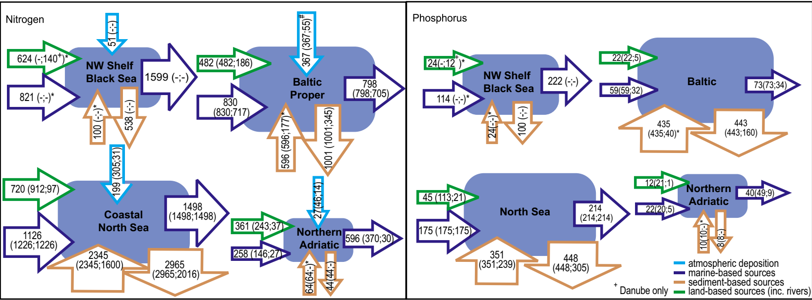
Fig. 24 Nutrient budgets for the four regional areas compared. All values are fluxes of TN or TP in thousands of tonnes per year, except fluxes evidenced by * that are DIN or DIP. Values between brackets respectively show fluxes during eutrophication and pre-eutrophication conditions. When an estimate was not possible, no value (-) is shown. Blue areas are proportional to basin surfaces.
