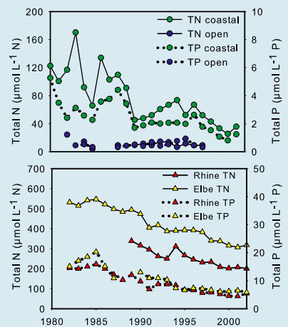
Fig. 18 Total nitrogen (TN) and total phosphorus (TP) have decreased in the Elbe and Rhine rivers resulting in decreased nutrient concentrations in the coastal North Sea (after McQuatters-Gollop et al. 2007).
