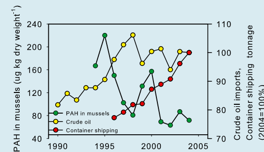
Fig. 14 Decoupling of PAH contamination from oil imports and shipping.
