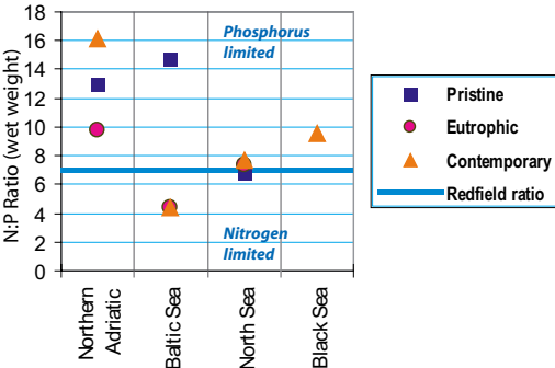
Fig. 25 Estimates of N:P ratios of inputs to all four seas.
