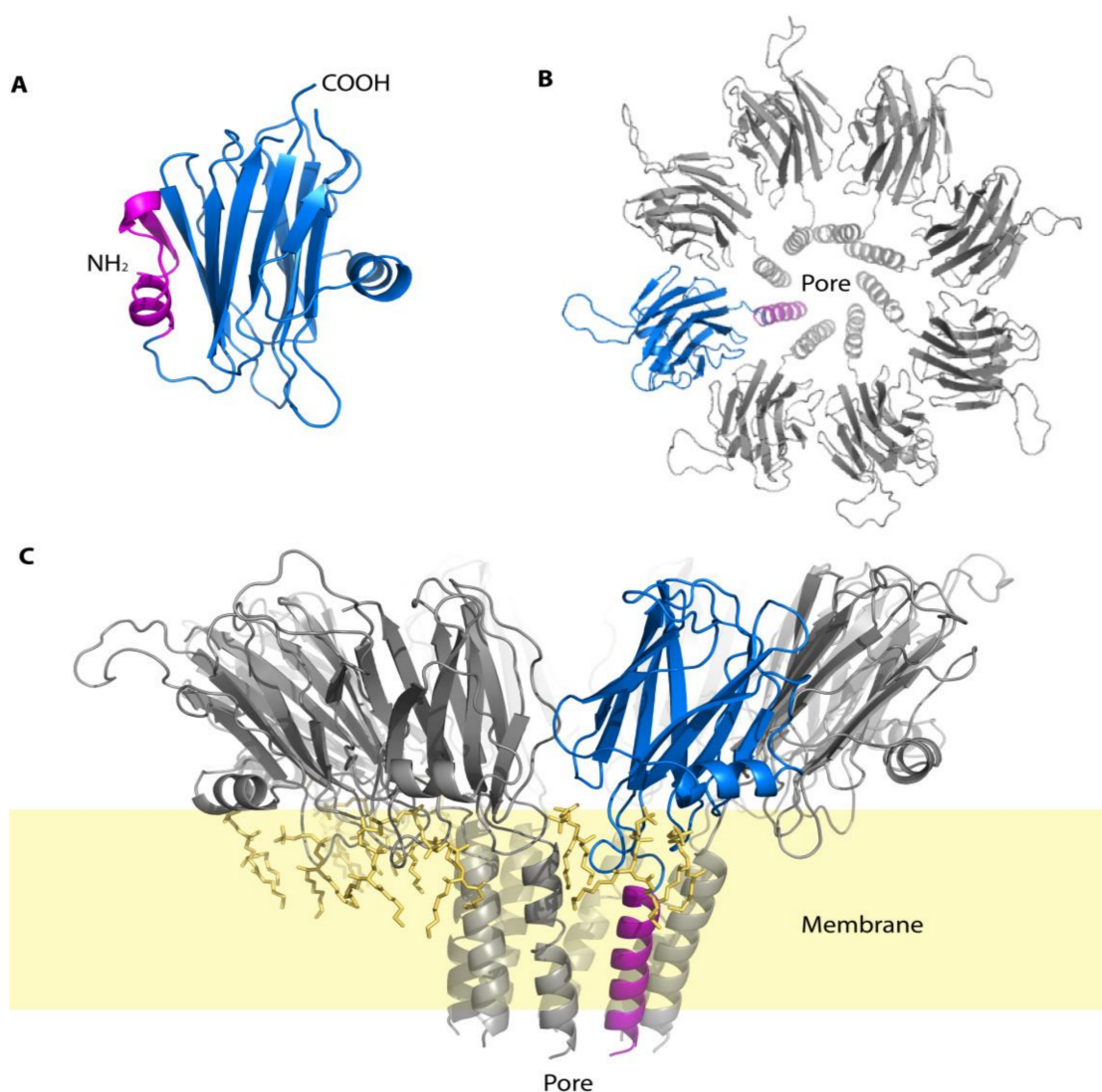
Figure 5. Putative three-dimensional structure of echotoxin 2 in monomeric (solution) and octameric (membrane-bound) forms. The structure was obtained by homology modeling using the crystallographic structure of fragaceatoxin C and generated using PyMol [73]. (A) Molecular model of monomeric, inactive echotoxin 2 (B) View from the extracellular side of the molecular model of echotoxin 2 in an octameric form (C) Side view of the molecular model of the octameric of echotoxin 2 embedded in a lipid bilayer (yellow). One of the monomer in each panel was represented in blue and its N-terminal active region shown in pink. This region change conformation depending if the monomer is in solution (A) or embedded in the membrane (B,C). The shaded region in (C) represent the approximate position of the membrane.
