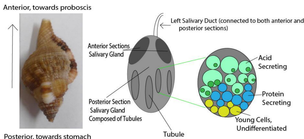
Figure 6. Diagram of the left salivary gland of Cymatium , showing the spatial differentiation within the blind tubules of the posterior salivary gland as described by Andrews et al. [58].
