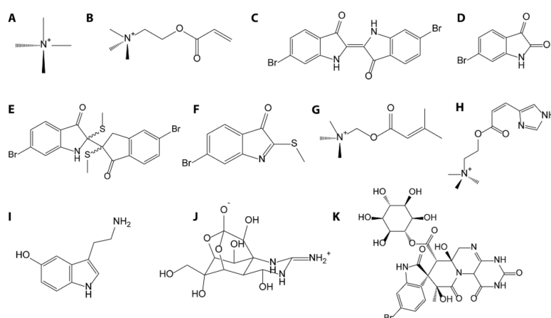
Figure 4. Small molecule compounds discussed in this review. (A) Tetramine, (B) acrylylcholine, (C) Tyrian purple, (D) 6-bromoisatin, (E) tyriverdin, (F) tyrindoleninone, (G) senecierylcholine, (H) urocanycholine (murexine), (I) serotonin (J) tetrodotoxin, and (K) surugatoxin.
