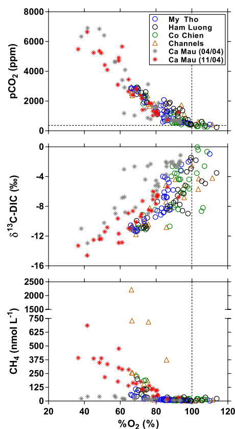
Figure 10. Distribution as a function of oxygen saturation level ( \%O_2 , %) of the partial pressure of CO 2 (pCO 2 , ppm), stable isotope composition of dissolved inorganic carbon ( \delta^{13}\text{C-DIC} , ‰), and dissolved CH 4 concentration ( \text{nmol L}^{-1} ) in the three branches of the Mekong delta (Mỹ Tho, Hầm Luông, and Cốc Chiên) and side channels and in the mangrove creeks of the Ca Mau province in April and October 2004. The vertical dotted line indicates O 2 saturation (100 %); the horizontal line indicates the average atmospheric pCO 2 value.
