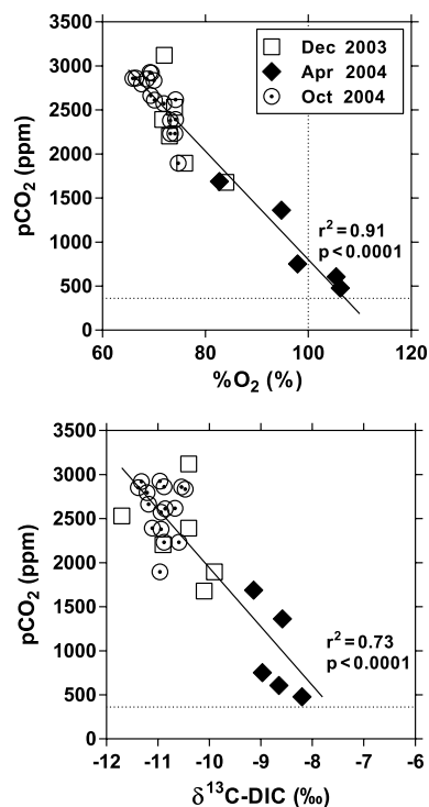
Figure 4. Variation in the partial pressure of CO 2 (pCO 2 , ppm) as a function of oxygen saturation level (%O 2 , %) and stable isotope composition of dissolved inorganic carbon ( \delta^{13}\text{C-DIC} , ‰) in the freshwaters (salinity 0) of the three branches of the Mekong delta (Mỹ Tho, Hàm Luông, and Cỏ Chiền) in December 2003, April 2004, and October 2004. The vertical dotted line indicates O 2 saturation (100 %); the horizontal line indicates the average atmospheric pCO 2 value.
