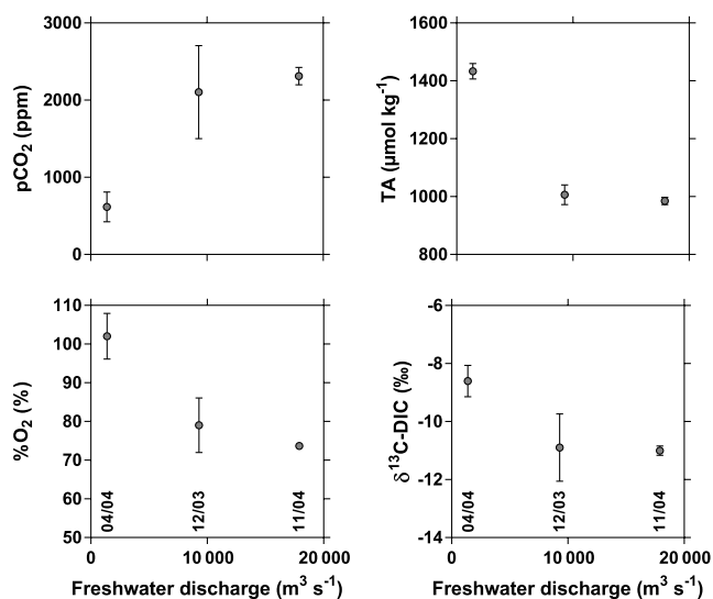
Figure 5. Variation as a function of freshwater discharge ( \text{m}^3 \text{s}^{-1} ) of the partial pressure of CO 2 (pCO 2 , ppm), oxygen saturation level (%O 2 , %), total alkalinity (TA, \mu\text{mol kg}^{-1} ), and stable isotope composition of dissolved inorganic carbon ( \delta^{13}\text{C-DIC} , ‰) in the freshwaters (salinity 0) of the three branches of the Mekong delta (Mỹ Tho, Hàm Luông, and Cốc Chiên) in December 2003, April 2004, and October 2004. Sampling dates (mm/yy) are indicated in the bottom panels.
