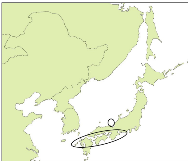
Fig. 31. Distribution of Heterocapsa circularisquama in Japan.
