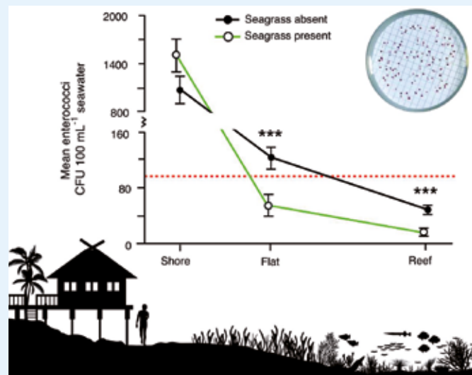
Figure 1.1 Seagrass meadows on intertidal flats reduce bacterial loads below the U.S. Environmental Protection Agency recommended human health risk exposure levels for a single water sample in recreational waters (dashed red line). From Lamb et al. , 2017.
