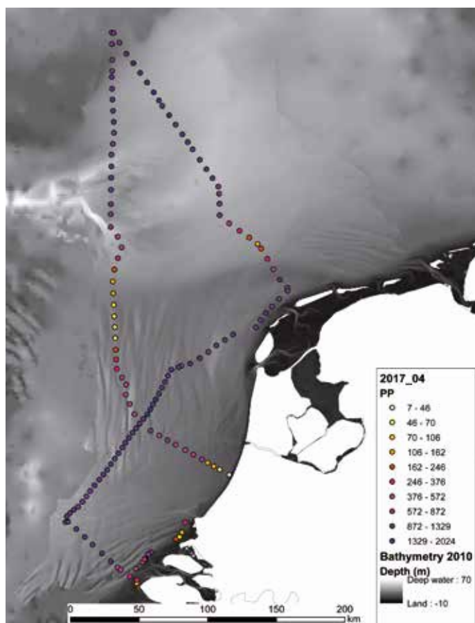
Figure 4.4 Primary production based on automated Fast Repetition Rate Fluorometry, using the water inlet of the ship (RV Zirfaea ), so the estimates of the daily water column productivity (mg C/m 2 /day) are based on samples taken at a fixed (subsurface) depth. From Aardema et al. , (2018).
