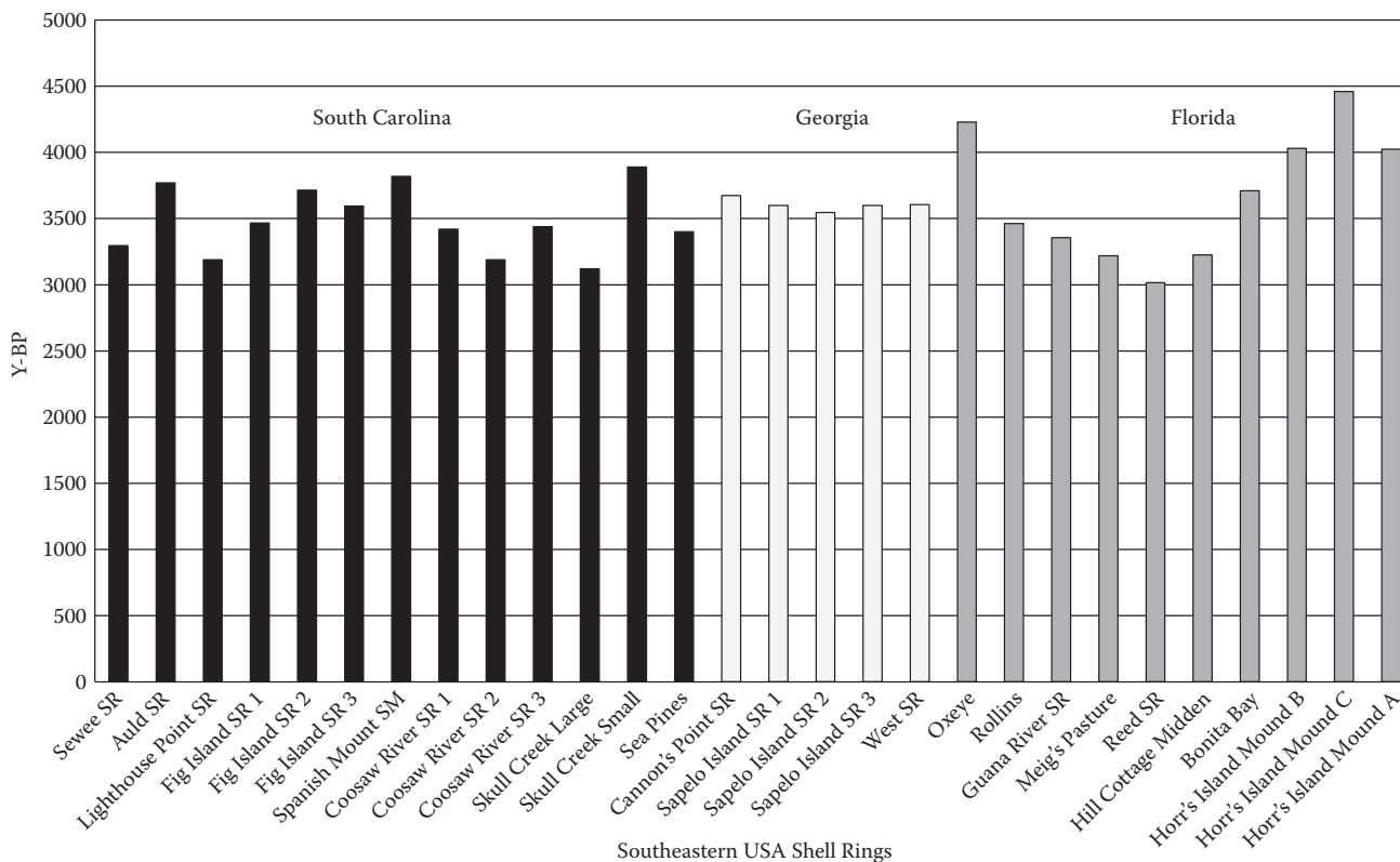
FIGURE 2.2 Radiocarbon dates of southeastern United States shell rings. (From Russo, M. 2006. Archaic Shell Rings of the Southeast U.S.: National Historic Landmarks . Southeastern Archeological Center.)
