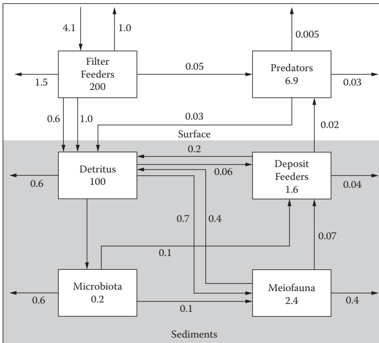
FIGURE 7.2 Carbon flow through an intertidal oyster reef in South Carolina. Flow = \text{gC m}^{-2} \text{d}^{-1} ; states = \text{gC m}^{-2} . (Adapted from Dame, R.F. and Patten, B.C. 1981. Analysis of energy flows in an intertidal oyster reef. Mar. Ecol. Prog. Ser. , 5, 115–24.)
