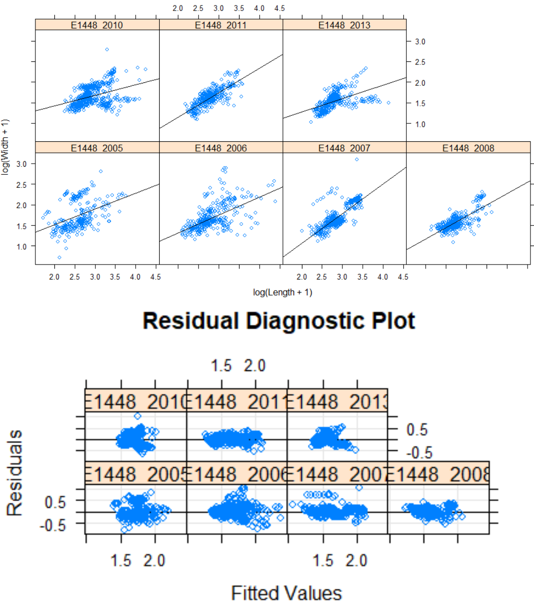
AnnexFigure 18 General Linear model of Width over Length ( \log(x+1) ) of the Veral in Zuriza site. Heterosedasticity and bias.
