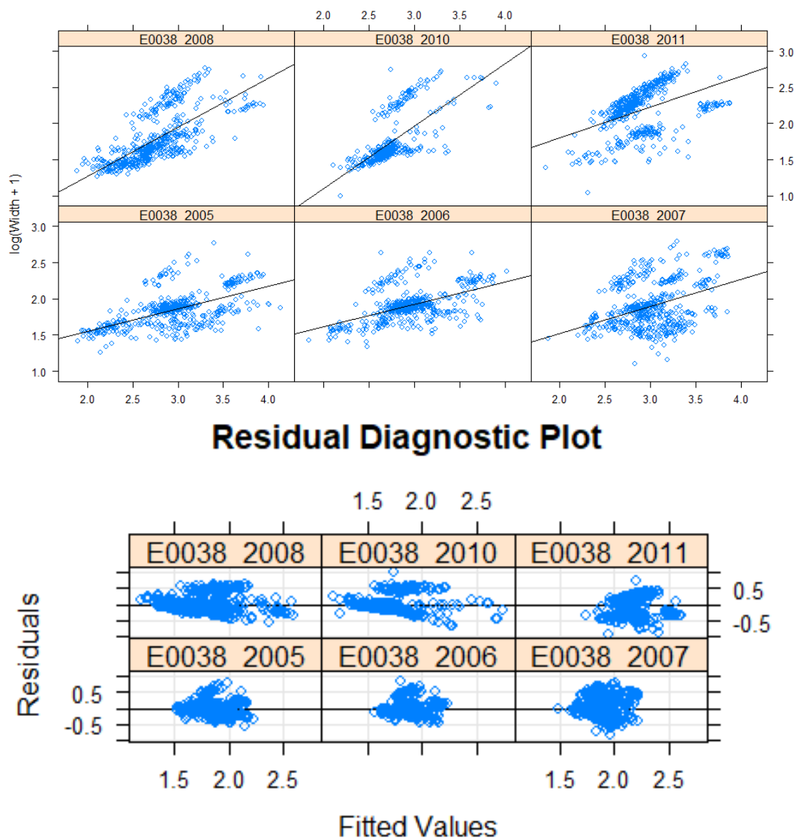
AnnexFigure 14 General Linear model of Width over Length ( \log(x+1) ) of the Najerilla in Torremontalbo site. Heterosedasticity and bias.
