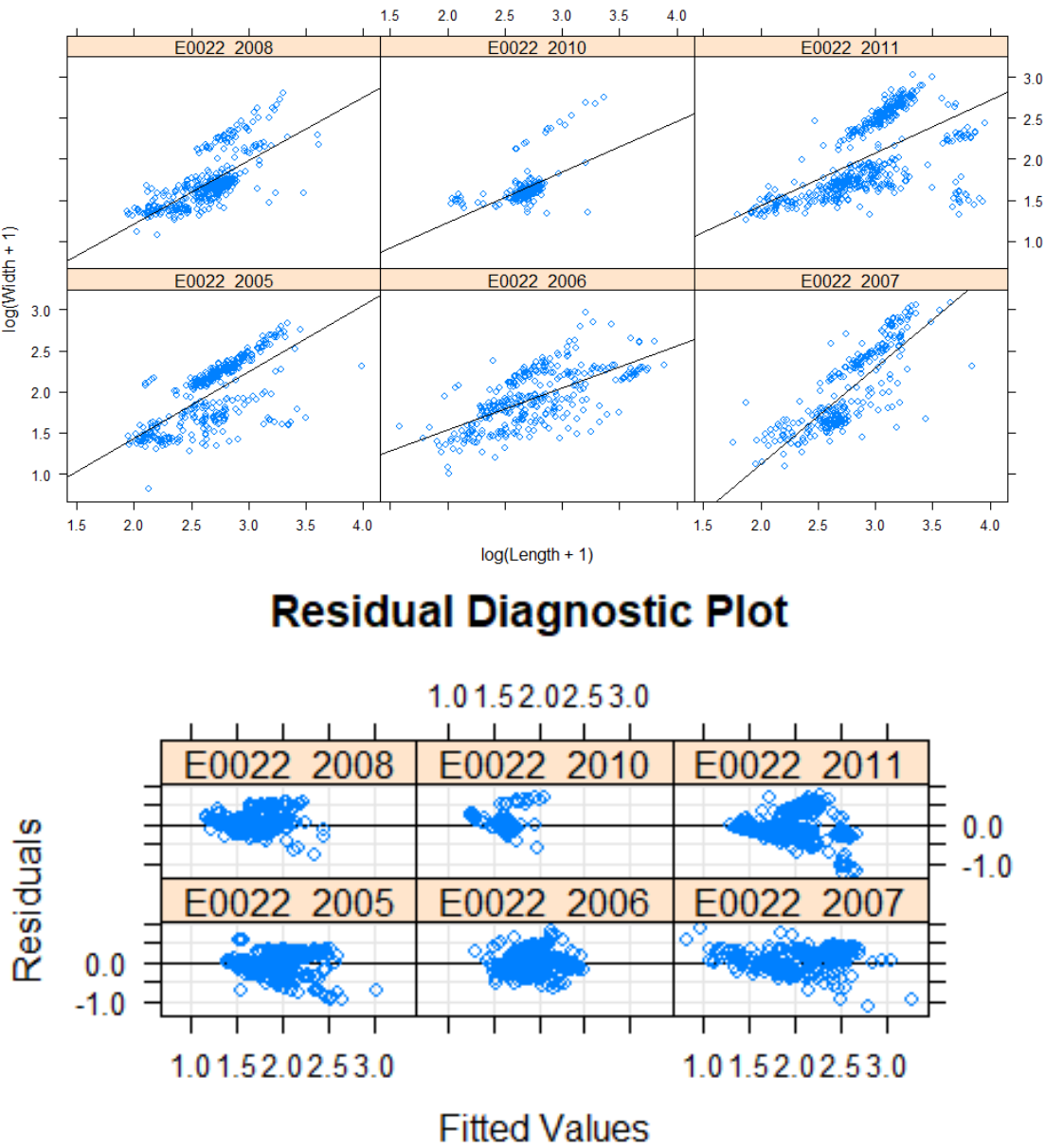
AnnexFigure 13 General Linear model of Width over Length ( \log(x+1) ) of the Valira in Anserall site. Heteroscedasticity and bias.
