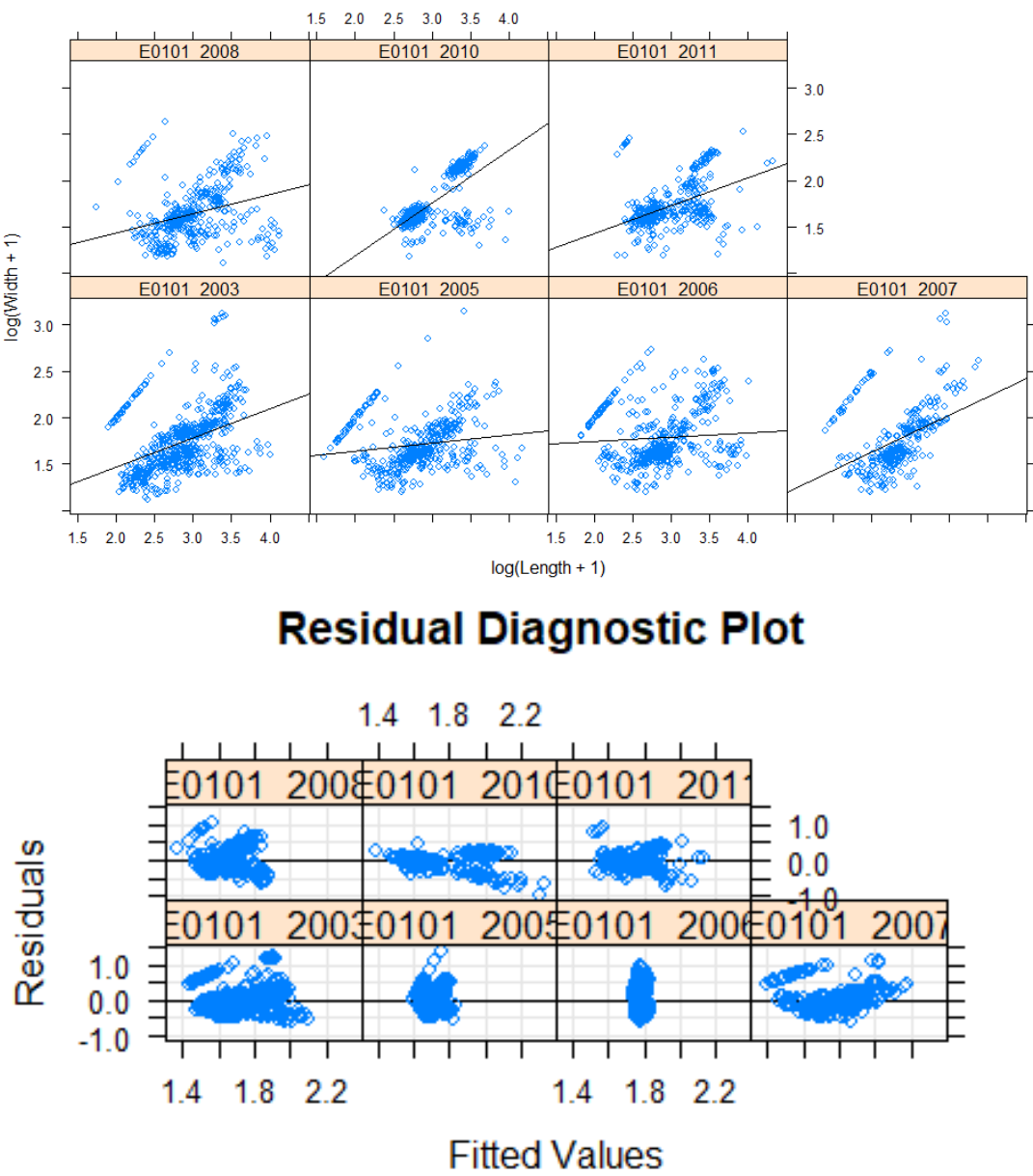
AnnexFigure 15 General Linear model of Width over Length ( \log(x+1) ) of the Aragón in Yesa site. Heterosedasticity and bias.
