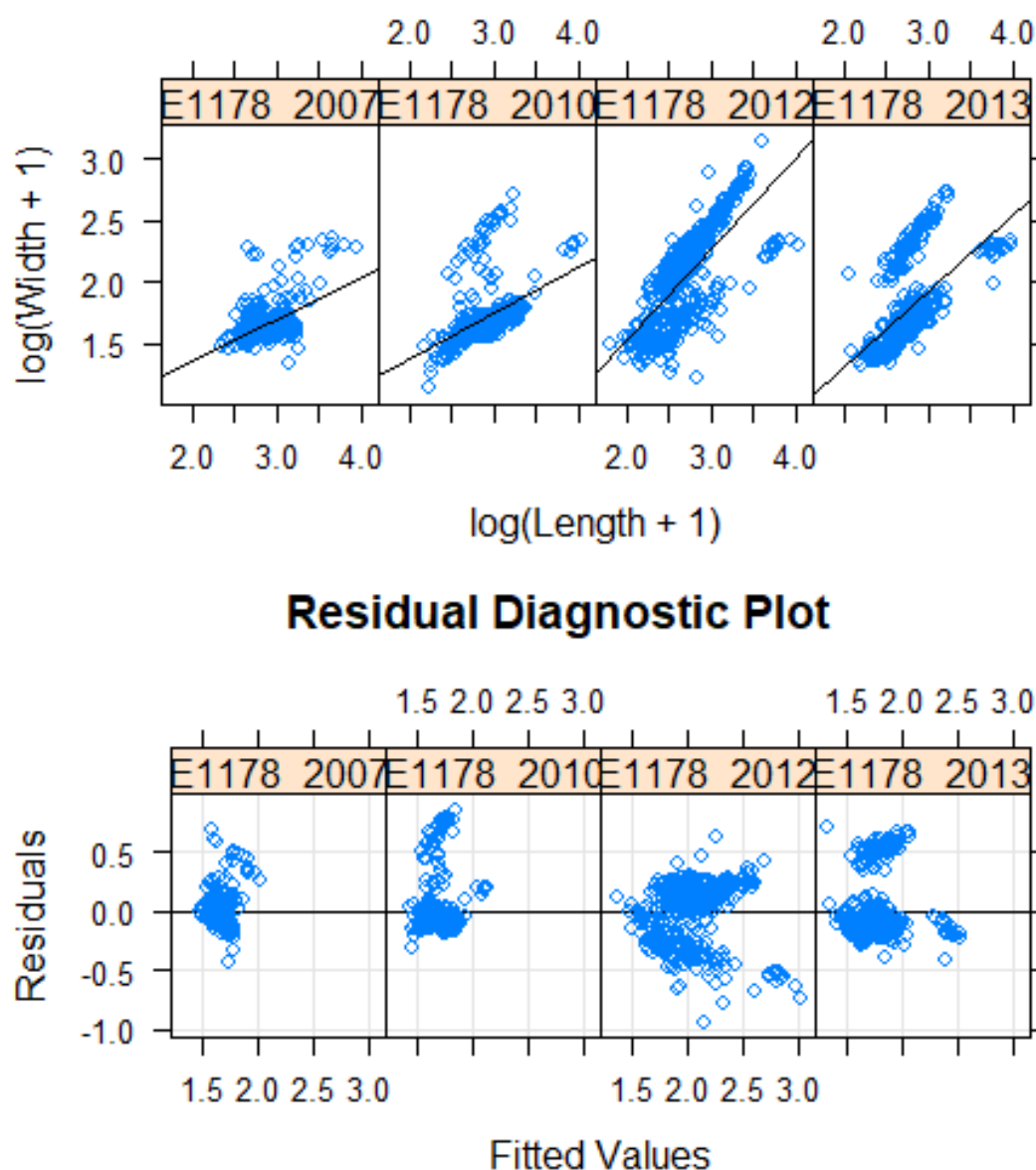
AnnexFigure 17 General Linear model of Width over Length ( \log(x+1) ) of the Najerilla in Villavelayo site. Heteroscedasticity and bias.
