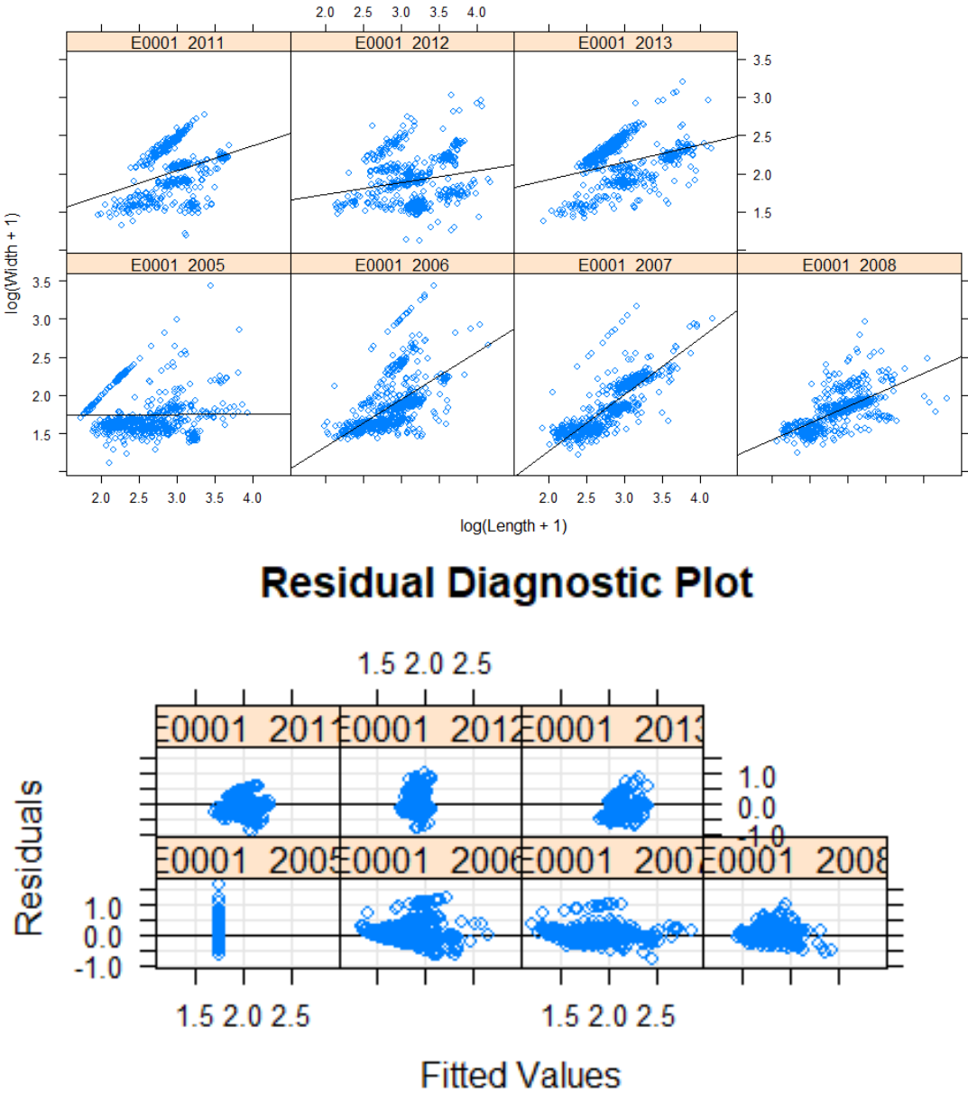
AnnexFigure 11 General Linear model of Width over Length ( \log(x+1) ) of the Ebro in Miranda site. Heterosedasticity and bias.
