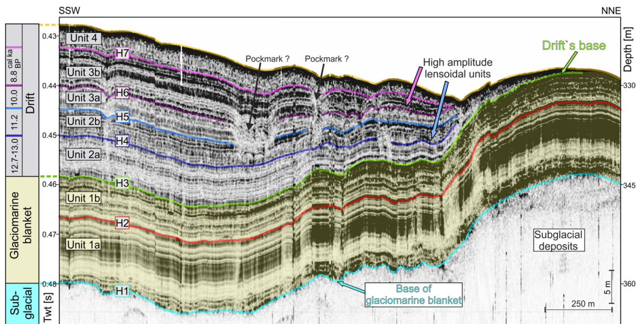
Fig. 6. Close up of NNE-SSW PARASOUND profile across the northern edge of the Kveithola Drift. Identified seismic horizons and intervening units are indicated. The available datings are indicated in the column to the left. The relatively minor extent and higher amplitude of Units 2.b and 3.b are apparent. See location in Fig. 1.
