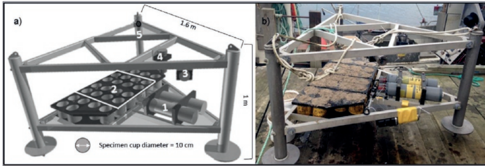
Fig. 2. 1: a) Benthic lander details (triangular aluminum frame): 1. Valve gape recorders, 2. Specimen cups: 16 for valve gape the experiment (within white rectangle), and 12 controls for future growth studies, 3. ALEC fluorimeter, 4. ALEC PAR sensor, 5. Conductivity and Temperature. b) Benthic lander before deployment.
