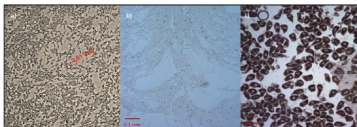
Fig. 7B. 2: a) Male gonadal tissue of Arctica islandica , b) no cellular structures definable as male or female c) female oocytes (October 2015)
