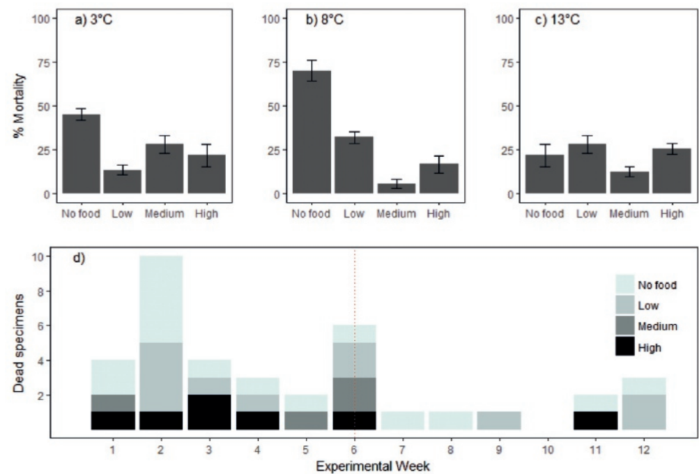
Fig. 4. 5: Percentage of average mortality at: a) 3 °C, b) 8 °C and c) 13°C. d) Number of dead specimens per food level and experimental week. Vertical line indicates the week that the midterm measurements were done. NOTE: No specimens died at week 10.
