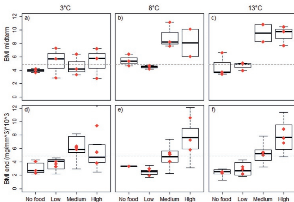
Fig. 4. 3: Body Mass Index (BMI) per treatment: at midterm (45 d; n=34 ): a) 3°C, b) 8°C, c) 13°C, and at the end of the experiment (93 d ) d) 3°C, e) 8°C, f) 13°C. Horizontal line denotes average BMI at the start of the experiment (reference BMI). Red diamonds indicate average per aquarium (data used for the statistical analysis) and boxplot show the inter-specimens variation ( n_{\text{midterm}}=34, n_{\text{end}}=89 ).
