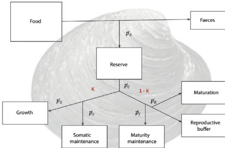
Fig. 6.2: Representation of the main metabolic processes in DEB theory (Kooijman 2010). There are six energy fluxes: assimilation ( \dot{p}_A ), mobilization ( \dot{p}_C ), somatic maintenance ( \dot{p}_S ), growth ( \dot{p}_G ), maturity maintenance ( \dot{p}_J ), and maturation + reproduction ( \dot{p}_R ). NOTE: The parameter \kappa (red kappa) is the fraction of the mobilized energy allocated to growth and somatic maintenance. The remaining portion 1-\kappa is the fraction allocated to maturity maintenance and to maturation (for juveniles) or reproduction (for adults). See supplementary material for equations.
