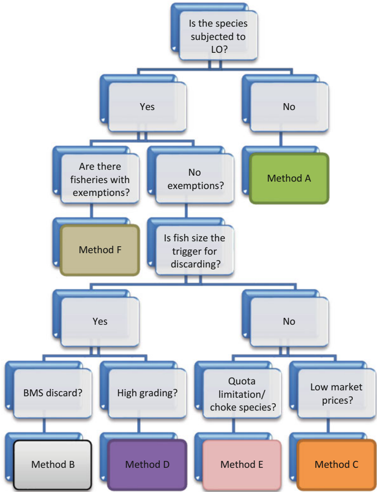
Fig. 19.4 Decision tree of the several methodologies used to estimate the discard ratio using reference data
