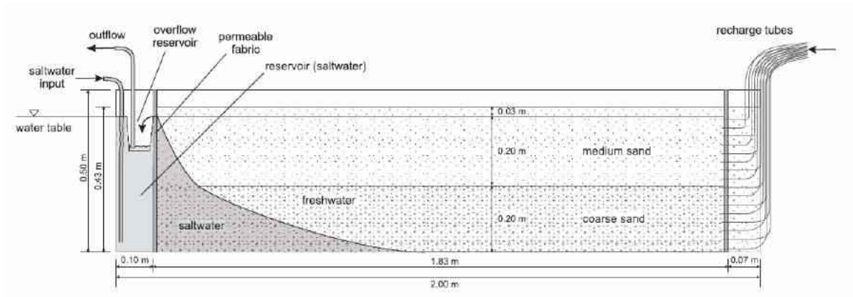
Figure 2. Sketch of the physical model experiment (Strack et al. 2016).
