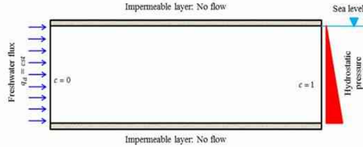
Figure 1. Schematic configuration of Henry Problem.
