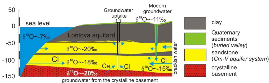
Figure 1. Conceptual model characterizing the different sources of saline water affecting the glacial palaeogroundwater in the Cambrian-Vendian aquifer system at Viimsi peninsula, northern Estonia. The general features of this conceptual model are characteristic to all other case studies reported in the study.
