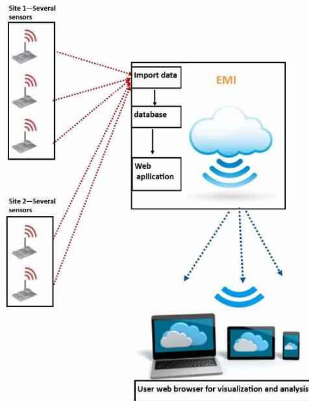
Figure 1: EMI architecture.
