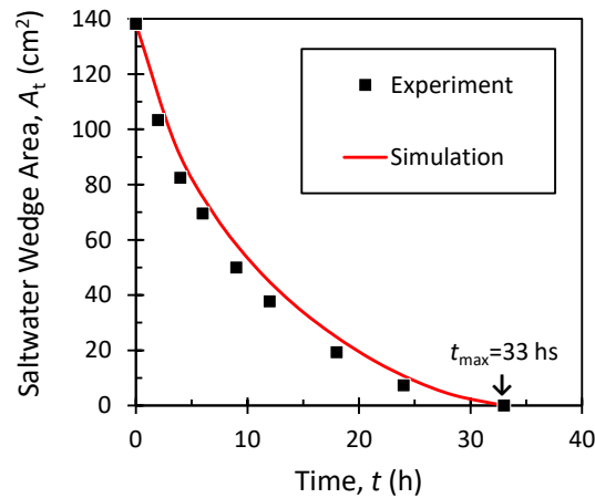
Figure 3. Comparison between the experiments and numerical simulations.
