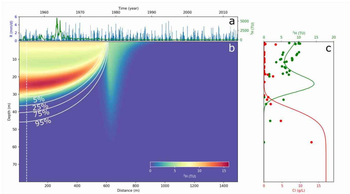
Figure 1. Graph showing the monthly recharge rate (blue) and 3 H activities (green) versus time. (b) Modeled contour plots of the 3 H activity (colours) and percentage of seawater (white contour lines). (c) Graph showing the 3 H activity (green) and chloride concentrations (red) as a function of depth along the white stippled line in (b). Lines indicate model results, data points represent samples from various locations across the lens from Houben et al. (2014) .
