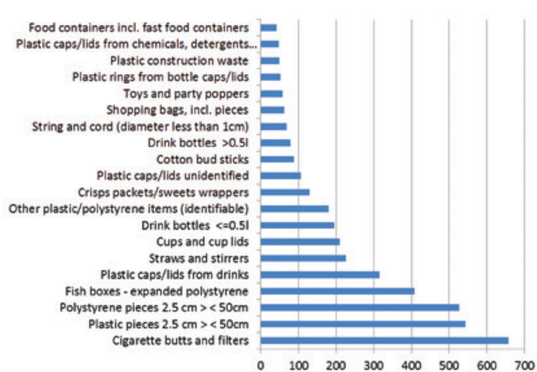
Figure 2.14. Top 20 items found in Greece , on an aggregated basis of total litter counts in all surveyed beaches.
