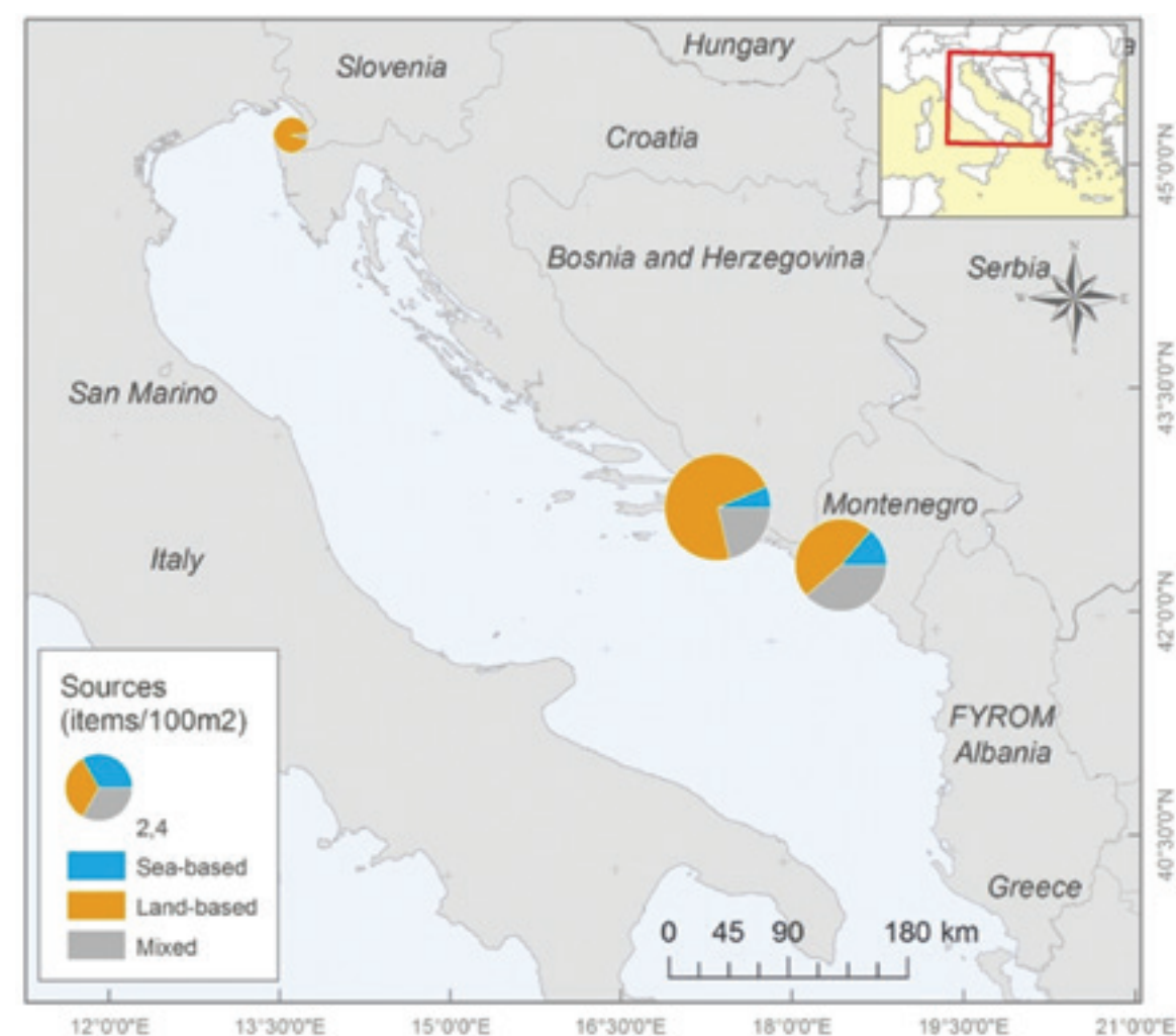
Figure 4.38. Relative densities of the sea-based vs land-based items (items/100 m 2 ), showed by country.
