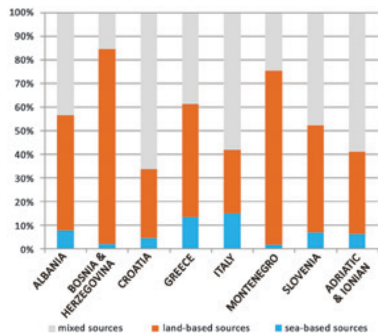
Figure 2.20. Assessing the comparative importance of sea-based versus land-based sources of litter within the sourced items fraction.
