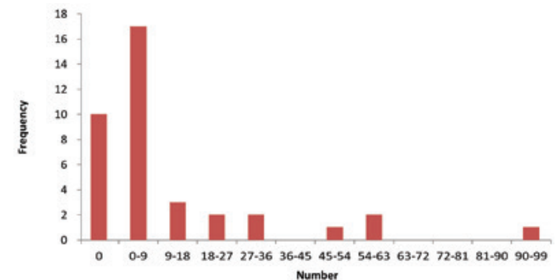
Figure 4.22. Frequency distribution (ten classes of frequency) of the number of seafloor litter items found in the 38 transects performed.
