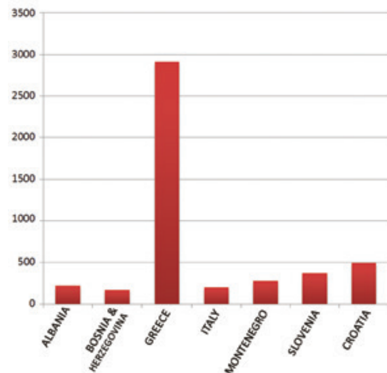
Figure 2.7. Aggregated results on national level showing the abundance of litter on average (number of items per 100-metre stretch)
