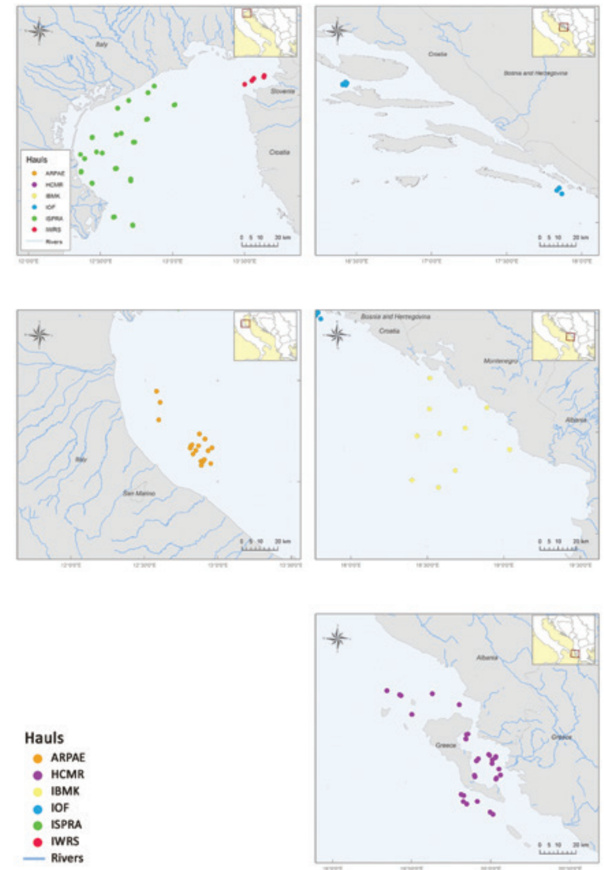
Figure 4.4. Magnified maps of the locations for bottom trawl surveys showing a central point for every haul performed by ARP AE, HCMR, IOF, ISPRA, IWRS and IBM.
