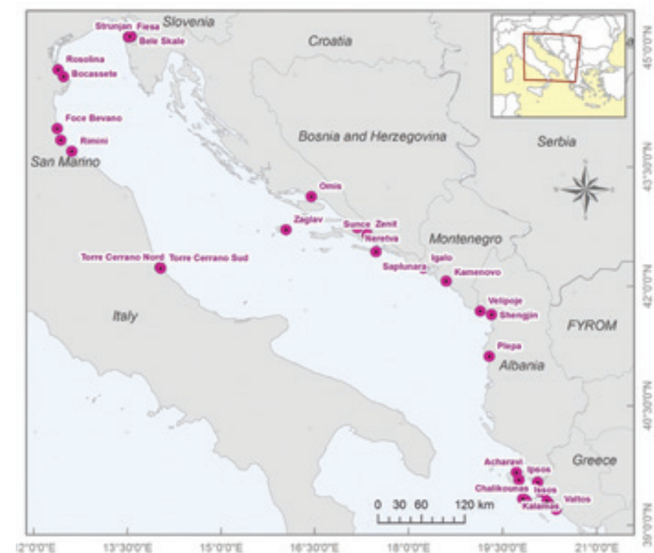
Figure 2.1. Map of the 31 study sites located on the coastline of the Adriatic and Ionian Seas.
