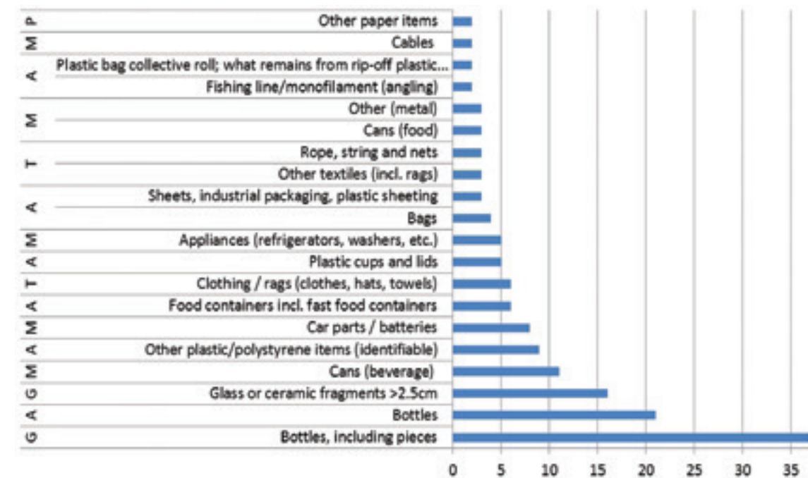
Figure 4.28. Top 20 seafloor litter items found in Montenegro , on an aggregated basis on an aggregated basis at national level (number of items). (A=artificial polymer materials; G = glass/ceramics; M = metal; P = paper/cardboard; R = rubber; T = cloth/textile; W = processed/worked wood).
