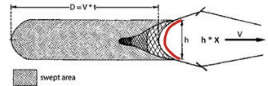
Figure 4.5. Swept area (source: http://www.fao.org/docrep/w5449e/w5449e0f.htm ).
