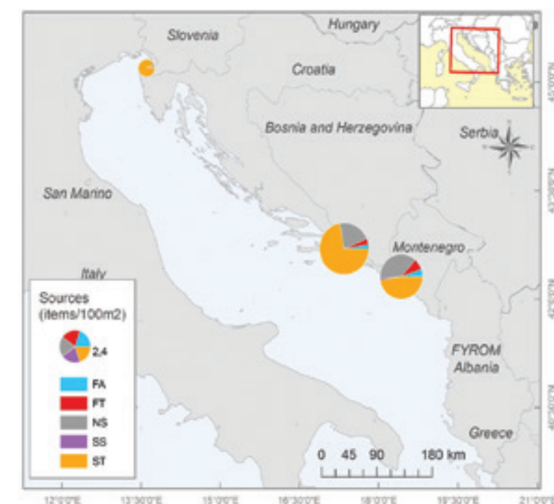
Figure 4.37. Aggregated results at national level with the densities of the seafloor litter items according to their source (items/100 m 2 ). (FA: fisheries & aquaculture; FT: fly-tipping; NS: non-sourced; SS: sanitary & sewage related; ST: shoreline, tourism and recreational activities).
