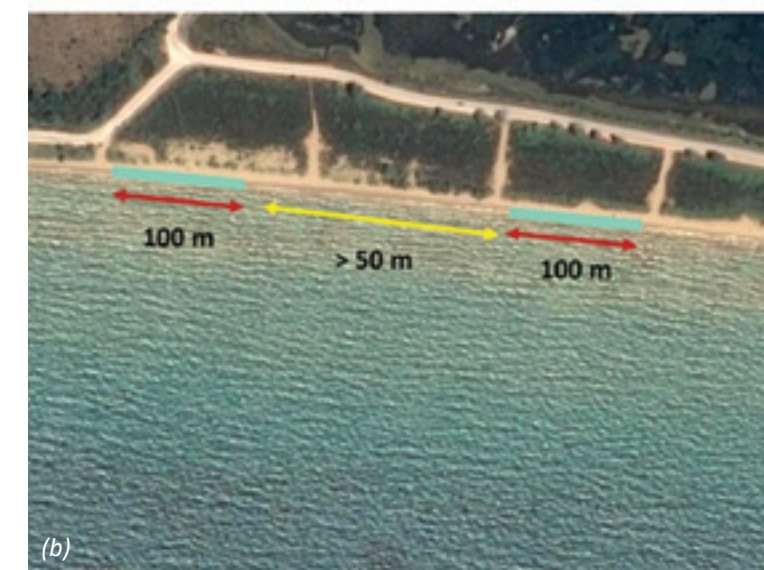
Figure 2.3. (a) The sampling unit; (b) Two sampling units (replicates) separated at least by a 50-metre stretch.
