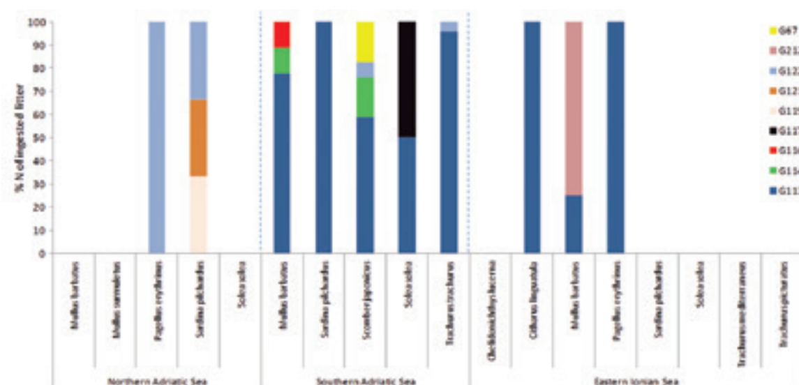
Figure 5.8. Percentage contribution (%N) of the ingested litter categories by species and area.
