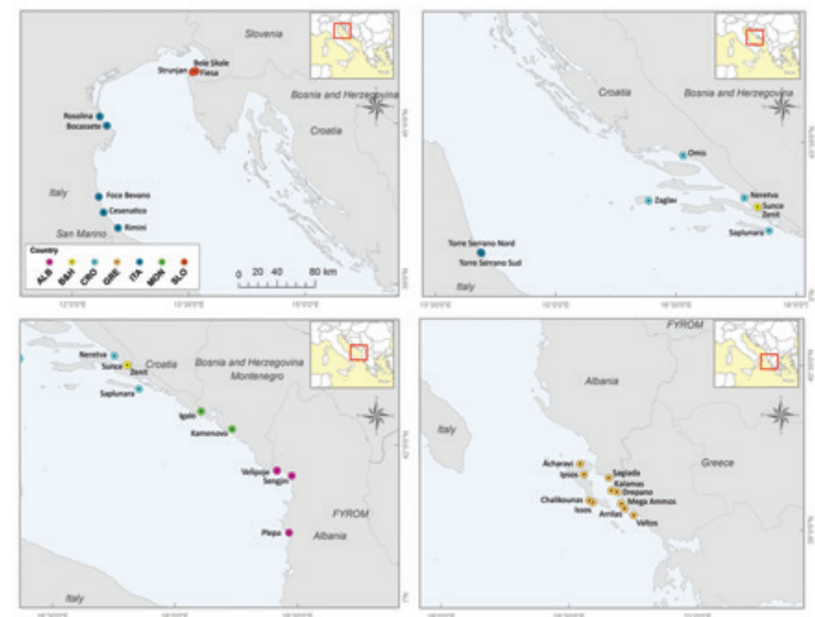
Figure 2.2. Magnified maps of the 31 study sites located on the coastline of the Adriatic and Ionian Seas.
