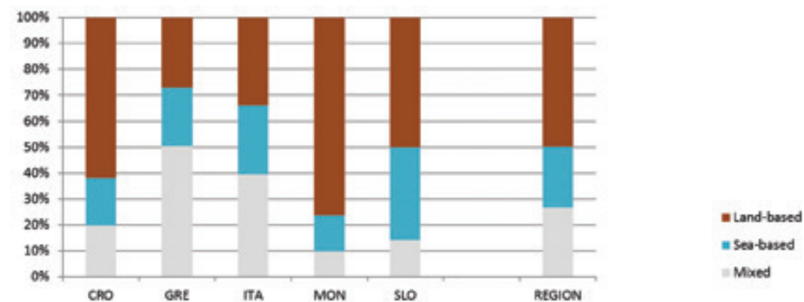
Figure 4.33. Aggregated results at a national and regional level for the contribution land-, sea-based and mixed sources related items found on the seafloor (%). (CRO: Croatia; GRE: Greece; ITA: Italy; MON: Montenegro; SLO: Slovenia).
