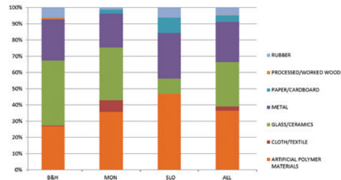
Figure 4.25. Seafloor litter composition in terms of number of items found in each country and as average value (B&H: Bosnia and Herzegovina; MON: Montenegro; SLO: Slovenia; ALL: average value).
