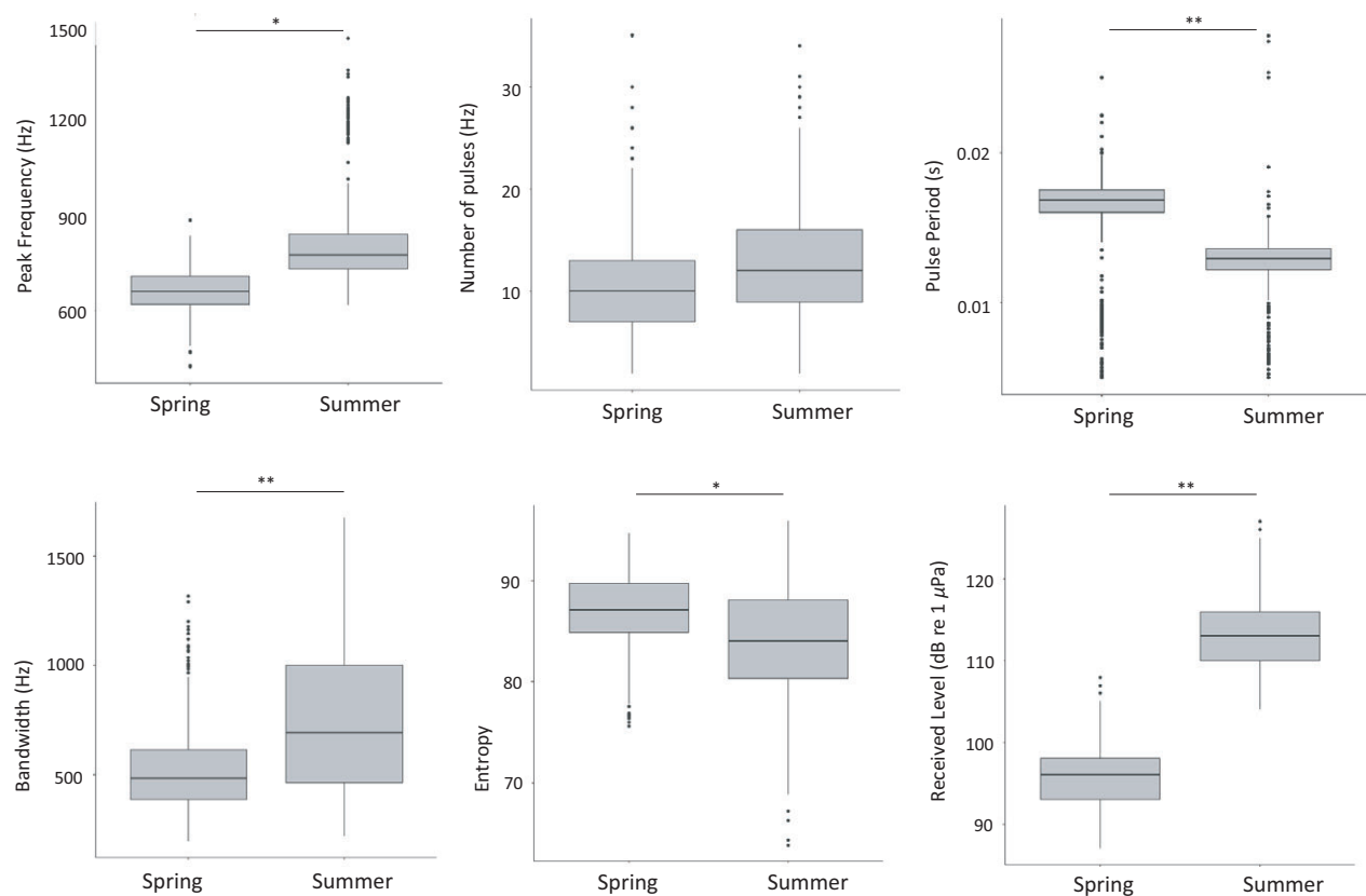
Figure 7. Feature comparisons of /kwa/ between spring (left) and summer (right) from meadow i and b , for which data across seasons were available from the same recording positions. Two night-time recordings were used for each season (09/04/15 and 26/04/15; 07/08/15 and 07/06/15). * P < 0.01 , ** P < 0.001 .
