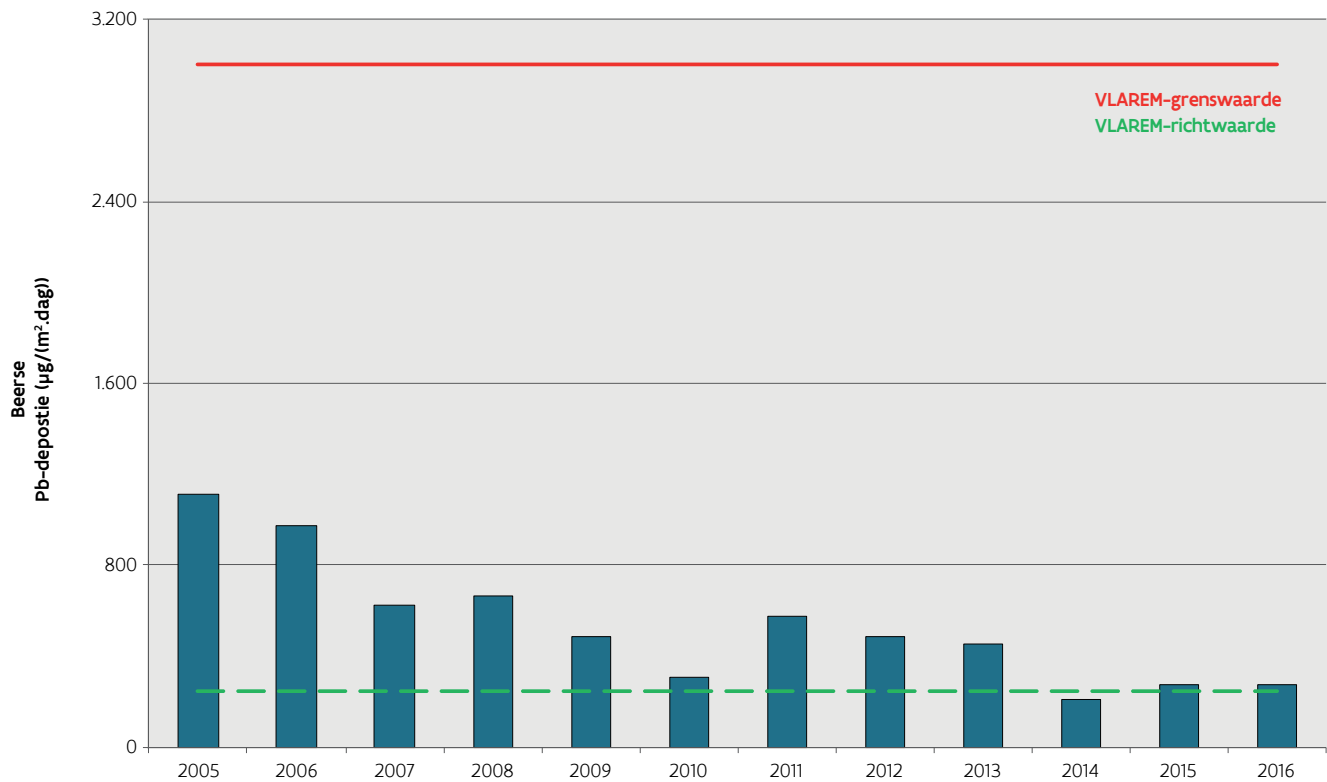
Figuur 11.33: Trend looddepositie in Beerse, 2005-2016
